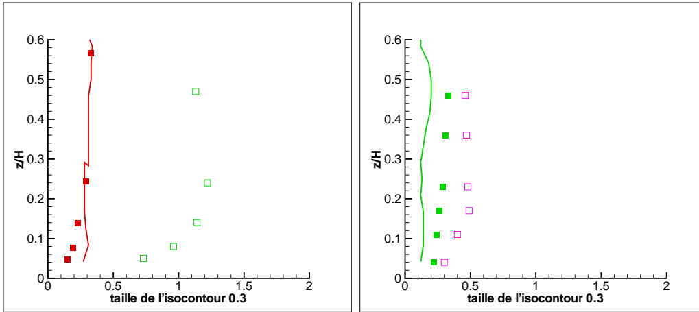
(a) \Delta x/\delta de \rho_{u'u'} = 0.3
