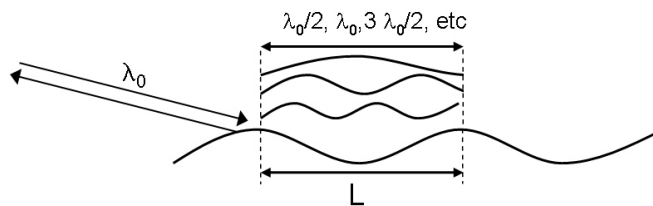
Figure 4.4: Trochoidal waves
