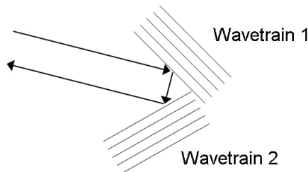
Figure 4.5: Horn reflection
