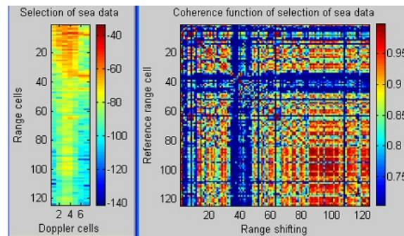
Figure 5.12: Coherence of positive Bragg line alone
