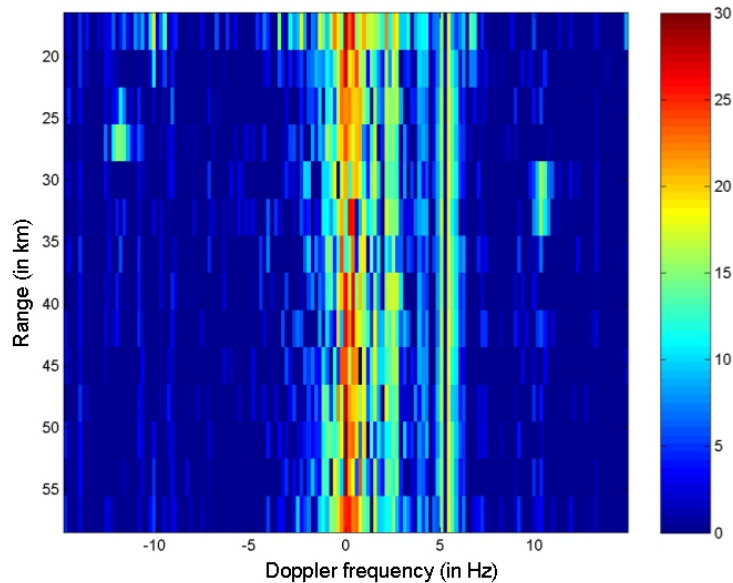
Figure 3.33: SNR level (in dB) detected by the biconical antenna at 14.80 MHz
