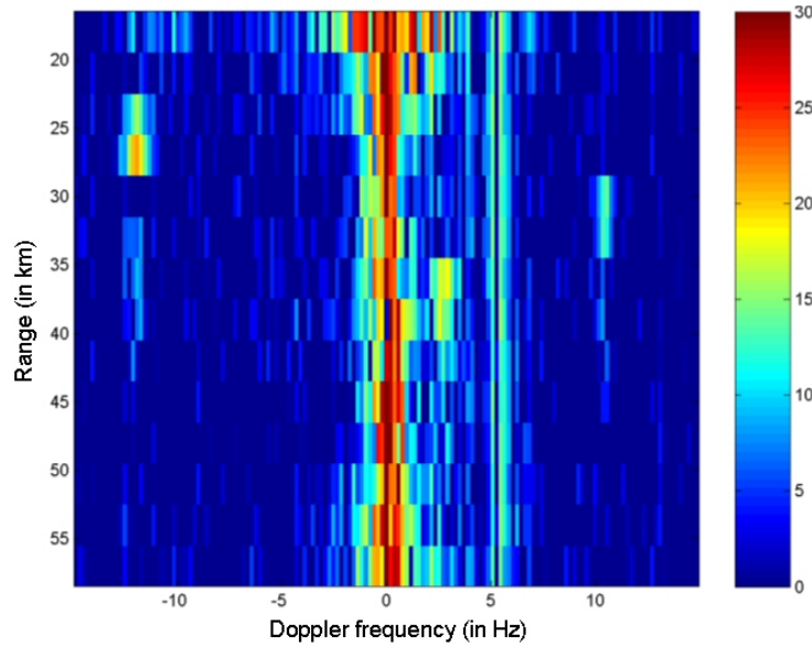
Figure 3.34: SNR level (in dB) detected by the prototype of compact HF antenna at 14.80 MHz
