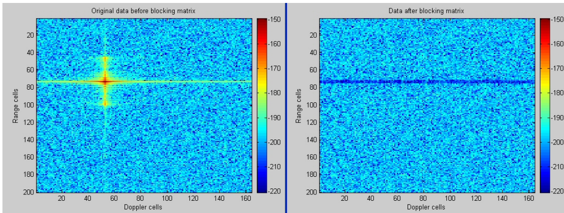
Figure 5.38: Effect of the blocking matrix on a simulated target at the range cell 73
