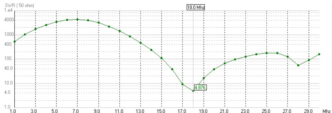
Figure 3.4: VSWR of the double MLA simulated with NEC-2
