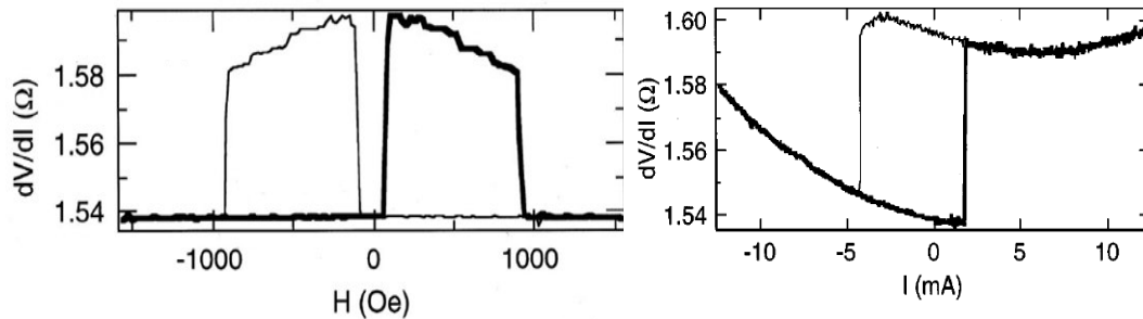
Fig. A.4 - 2 Left: Magnetoresistance curve (differential resistance dV/dI as a function of magnetic field H applied parallel to the long axis of the ellipse). Right: Differential resistance dV/dI as a function of the applied current I . (Extracted from ref. 6).
