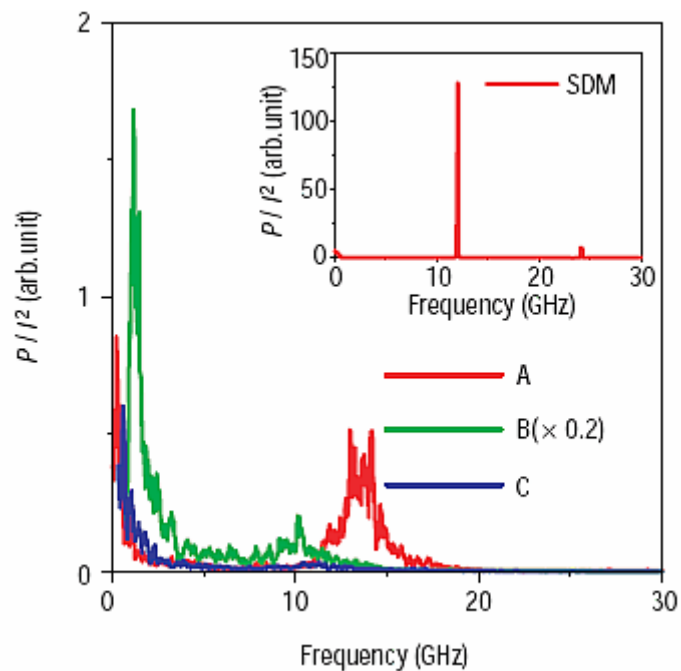
Fig. B.5 - 17 Calculated spectra corresponding to the current / field values marked A, B, C along Line 2 in fig. B.5 – 16. Inset: Macrospin microwave spectrum at I = 7 mA, H = 600 Oe.
