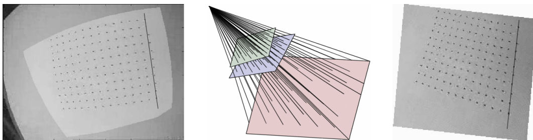
Figure 6.3: Calibration of a fish-eye's central image region using the central camera model. Left: one of three input images (in white the region that was calibrated). Center: calibrated lines of sight and estimated pose of calibration grids. Right: input image after distortion correction based on the calibration result. The distortion corrected for is not spectacularly large, but note that no parametric distortion model has been used here.
