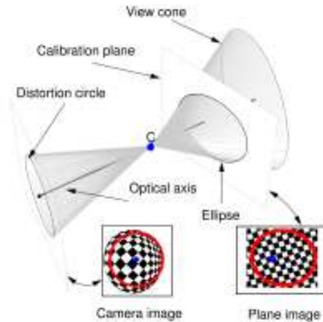
Figure 6.4: Radially symmetric camera model. Also shown is a calibration plane.
