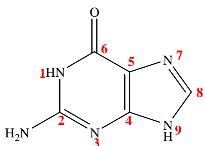
Guanine
