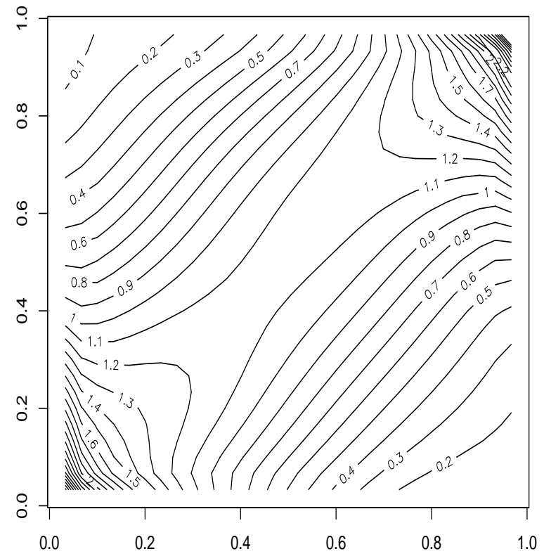
Estimation of the copula density (Beta kernel, b=0.1 )
