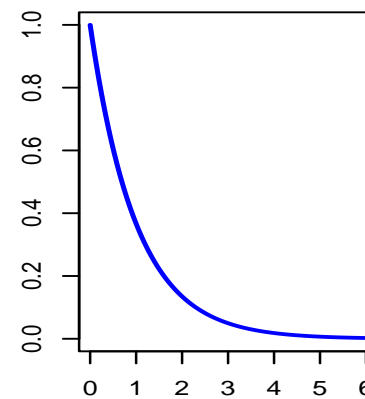
Laplace Transform
