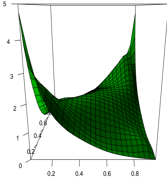
Estimation of Frank copula
