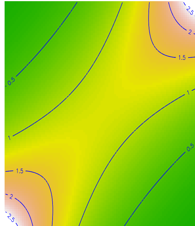
Level curves of the copula
