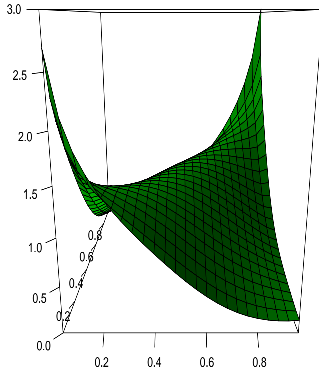
Estimation of the copula density (Beta kernel, b=0.1 )
