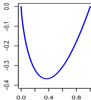
Lambda function
