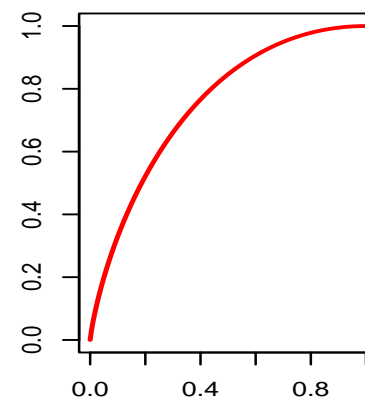
Kendall cdf
