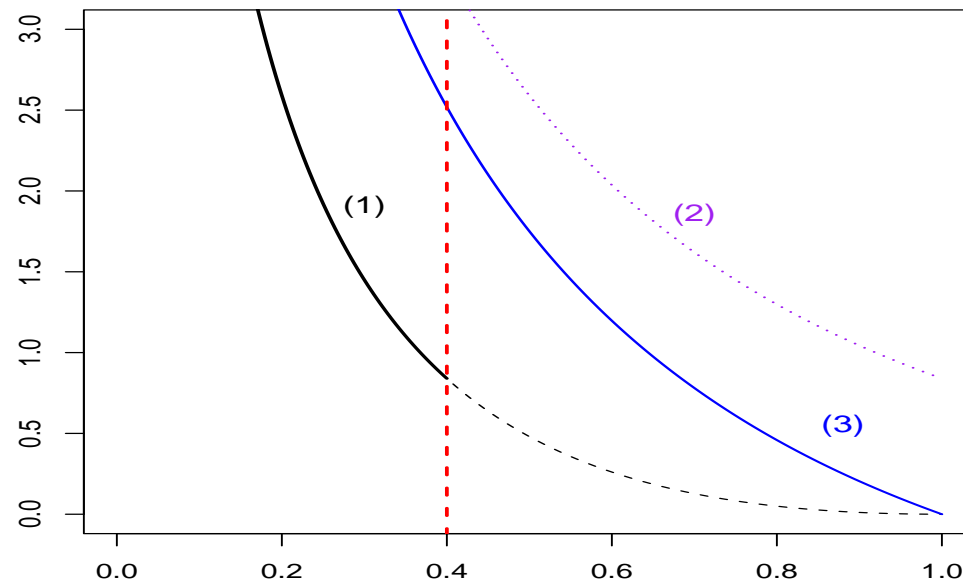
Generators of conditional Archimedean copulae
