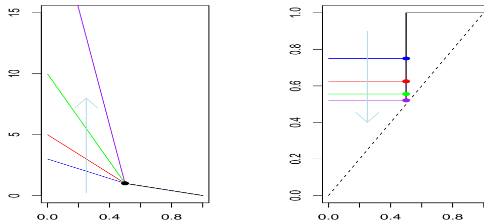
Sequence of generators and Kendall cdf's
