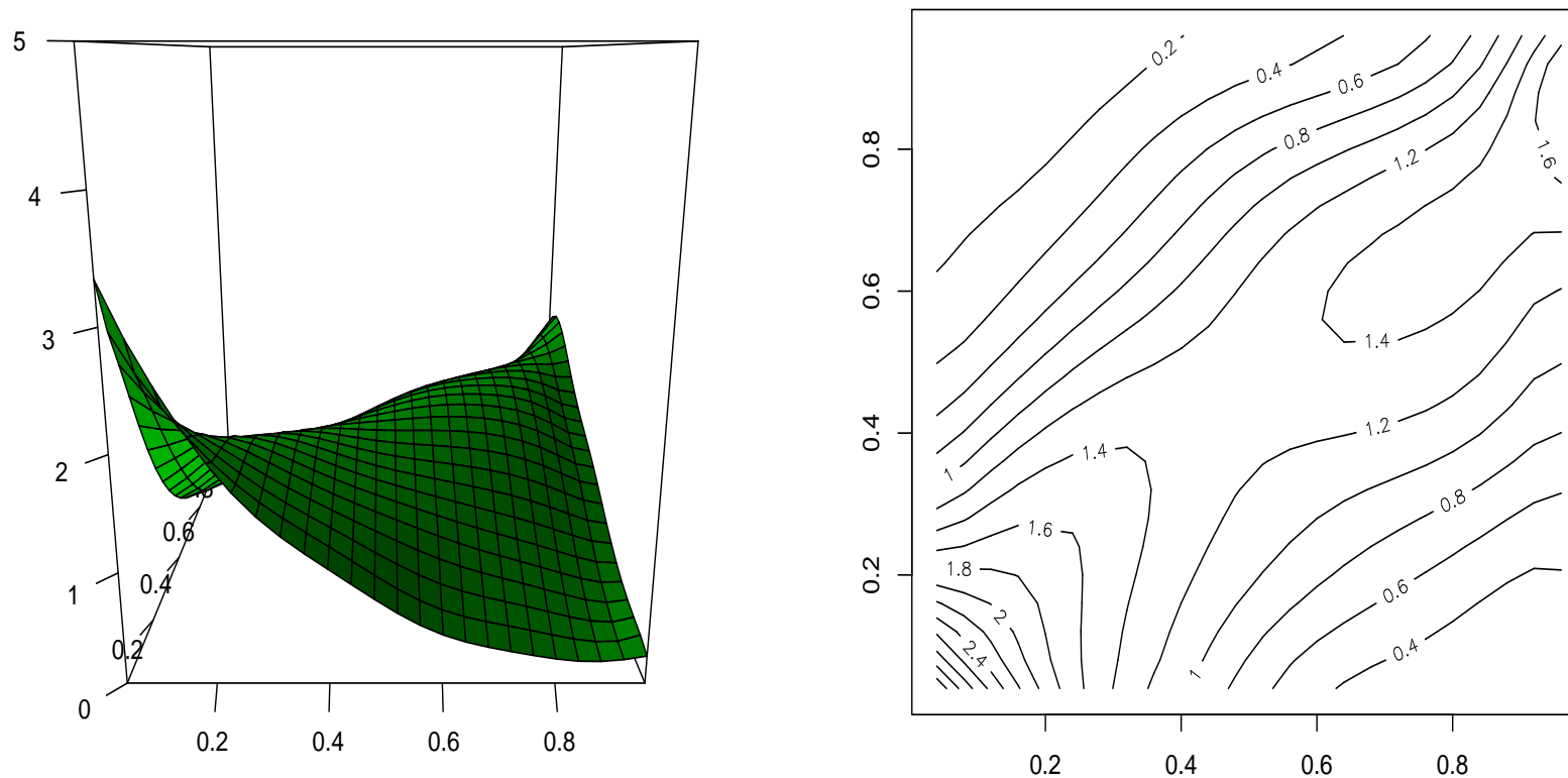
Estimation of Frank copula
