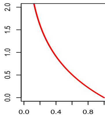
Archimedean generator
