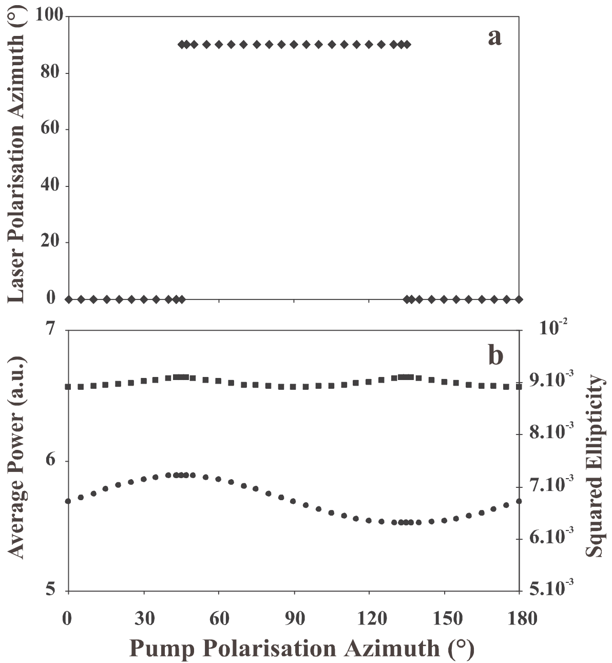
Figure 5 : Evolution (a) of the polarisation direction and (b) of the (■) average power and (●) squared ellipticity of the microchip laser versus the pump polarisation azimuth in the case of strong birefringence for \bar{\theta}_1 = 45^\circ . Numerical simulations with a birefringence corresponding to \Delta\nu = 6 GHz.
