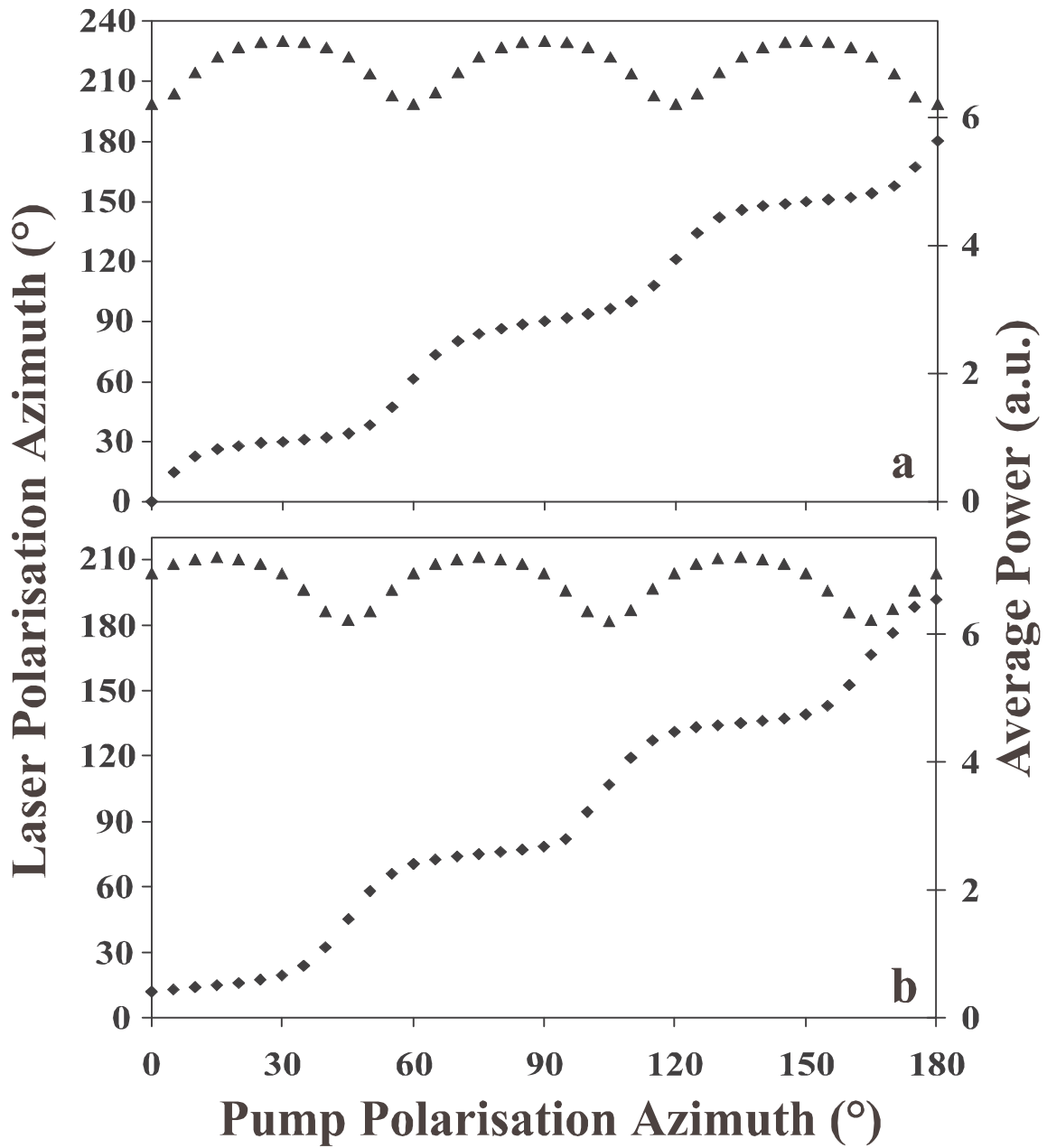
Figure 7 : Evolution ( \blacklozenge ) of the polarisation direction and ( \blacktriangle ) of the microchip laser average power versus the pump polarisation azimuth in the case of weak birefringence ( \Delta v = 0 ).
