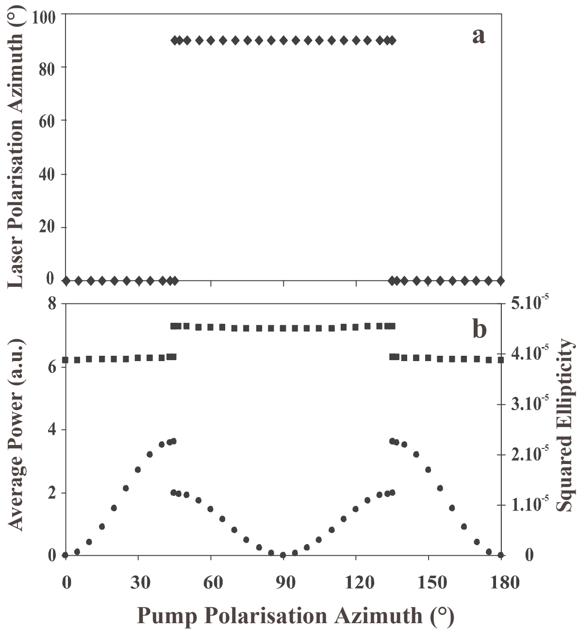
Figure 4 : Evolution (a) of the polarisation direction and (b) of the (■) average power and (●) squared ellipticity of the microchip laser the versus the pump polarisation azimuth in the case of strong birefringence. Numerical simulations with a birefringence corresponding to \Delta\nu = 6 GHz and one crystallographic axis aligned along one of the birefringence eigenaxes ( \bar{\theta}_1 = 0^\circ ).
