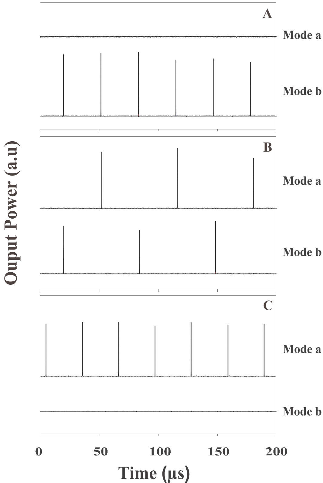
Figure 2 : Passive Q-switching pulses in the plateau (A and C, single polarisation) and in the transition region (B, alternating polarizations). Modes a and b correspond to linear polarisations along the cavity eigenmodes. The irregularities in the amplitude are due to the sampling technique.
