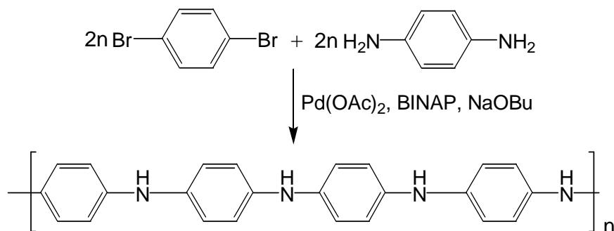
Fig. II.2.1 Synthesis of leucoemeraldine by polycondensation using 1,4-phenylenediamine and 1,4-dibromobenzene
