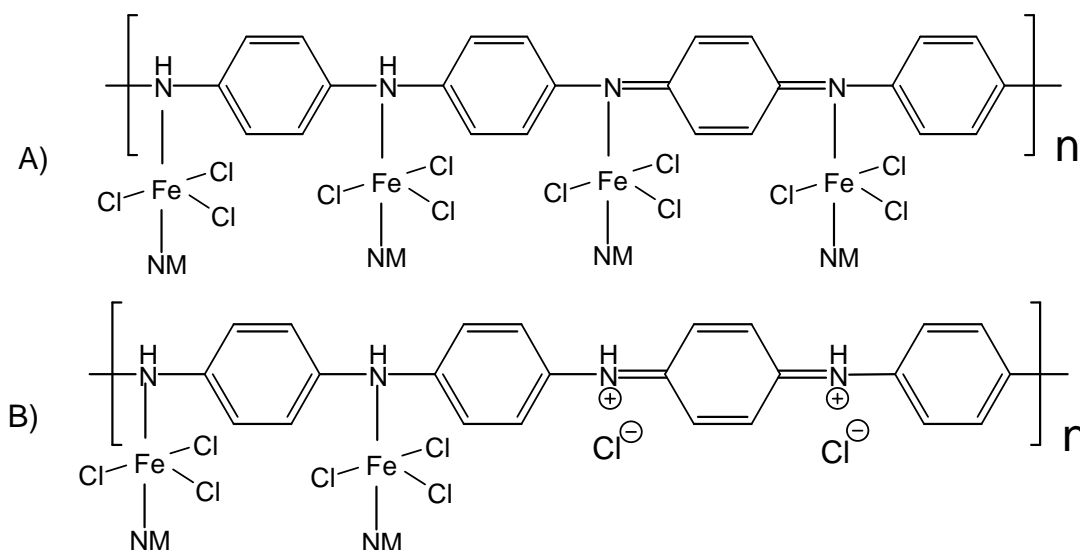
Fig. II.7.7 Emeraldine base (A), and emeraldine hydrochloride (B) doped with \text{FeCl}_3 in nitromethane (NM)
