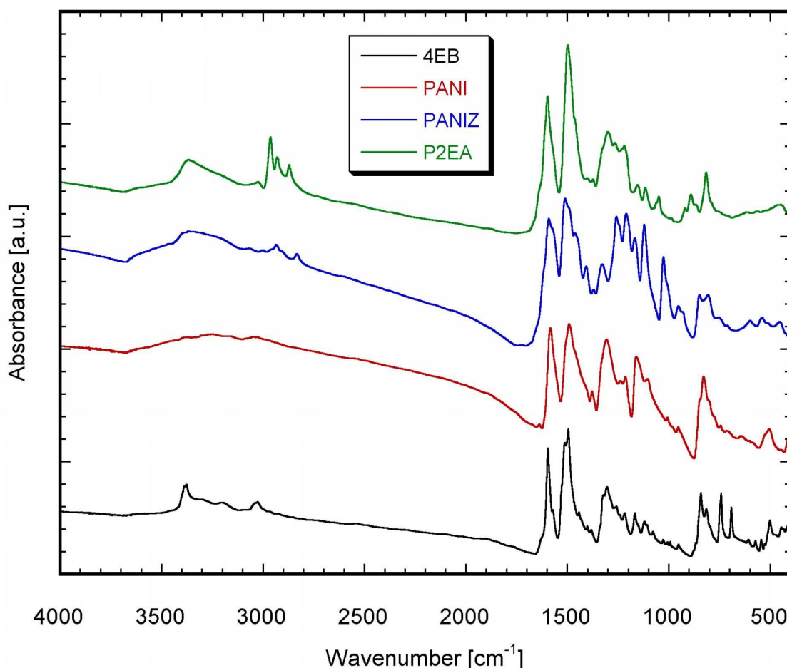
Fig. IV.1.5 IR spectra ( 4000\text{ cm}^{-1} - 400\text{ cm}^{-1} ) of polyaniline, polyanisidine, poly(2-ethylaniline) and the tetramer of aniline
