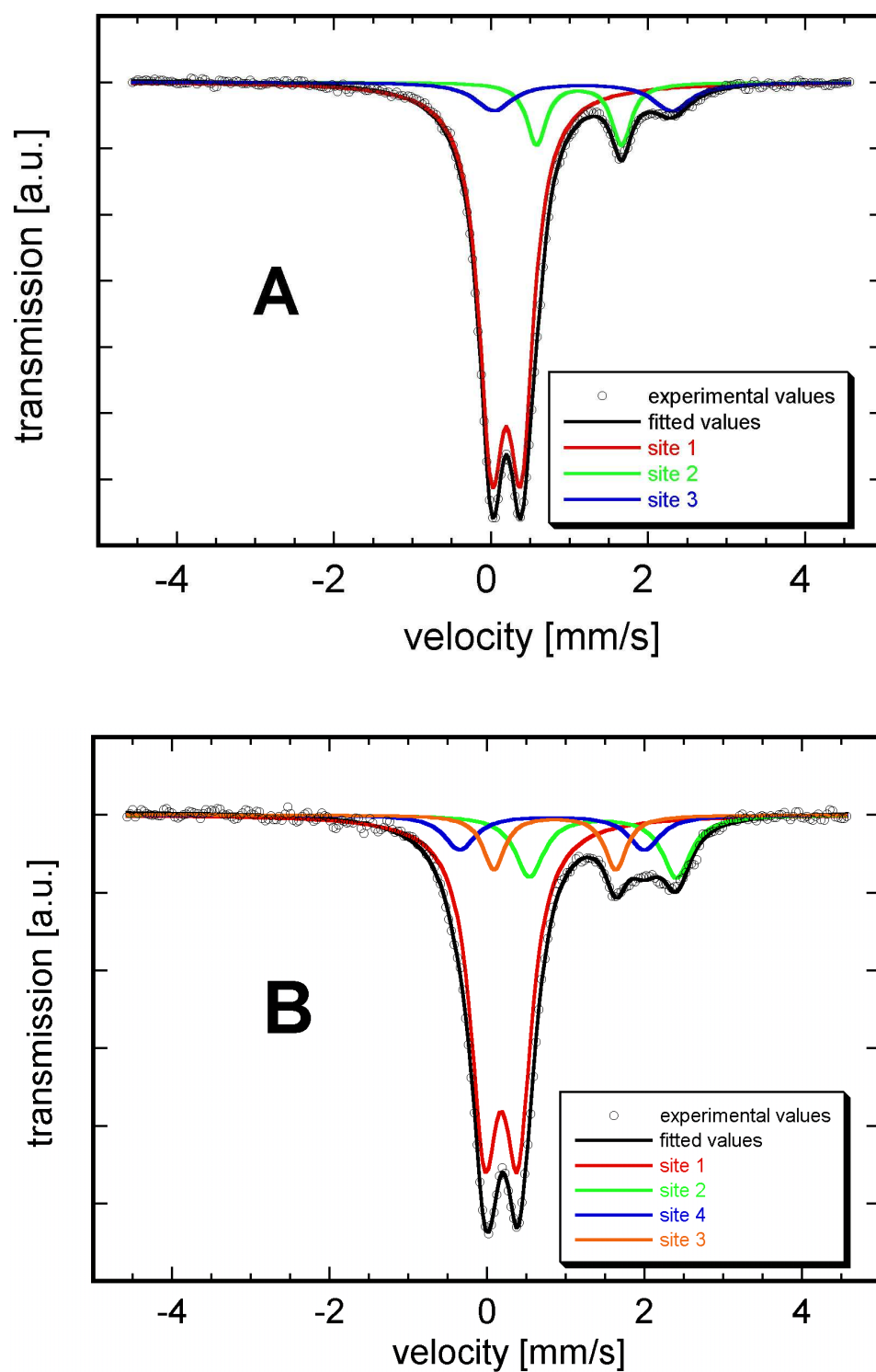
Fig. IV.3.8 Mössbauer spectra of A) polyanisidine, B) poly(2-ethylaniline), all compounds were treated with \text{FeCl}_3 and subsequently processed with triple excess of HFAA. Samples pumped for 40 hours, spectra registered at 77K.
