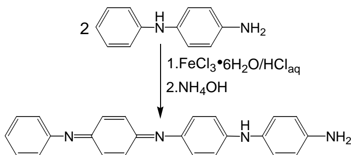
Fig. II.5.3 Oxidative synthesis of aniline Ph/ \text{NH}_2 tetramer
