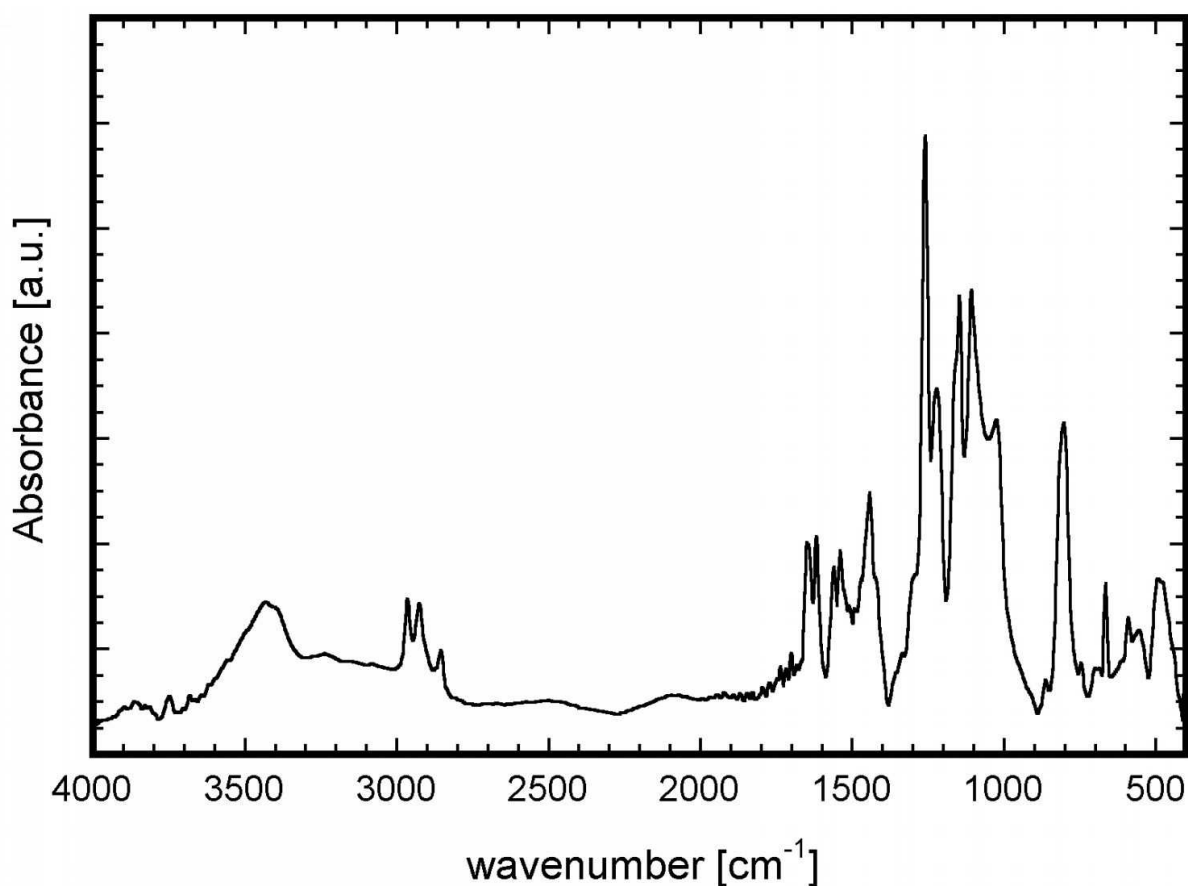
Fig. IV.3.7 Infrared spectrum of polyaniline doped with \text{FeCl}_3 (1:1) and subsequently treated with HFAA
