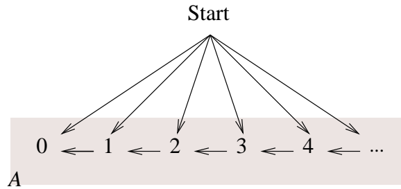
Figure 8.2: A transition system for which E_+(\llbracket \text{gfp}(f \mapsto \text{shift} f +_A 0) \rrbracket_t) < \llbracket \text{gfp}(f \mapsto \text{shift} f +_A 0) \rrbracket_{e_+} . While for any n there exists a trace that goes through A for n steps, there does not exist any trace going infinitely through A . On this system, greatest fixpoint analysis is inherently imprecise.
