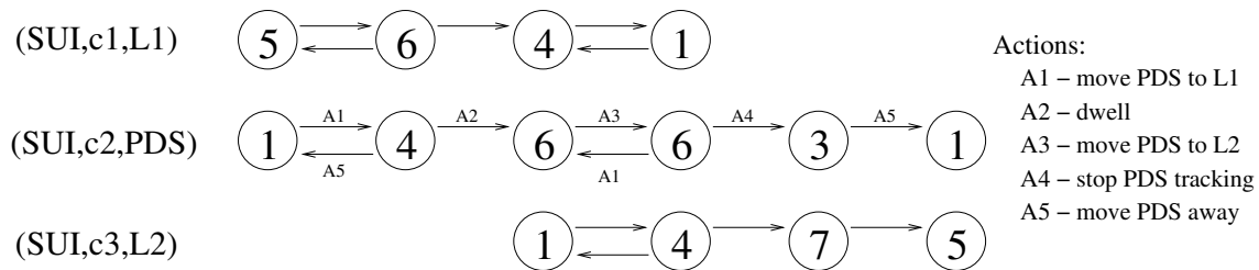
Figure 6.7: Coupling finite state automata for the menu-free PDS-based location control
