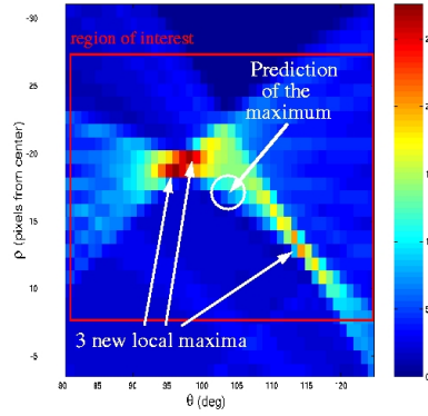
Figure 4.8: For one of the four maxima tracked: list of hypothetic new local maxima compared to its assumed position given by the prediction
