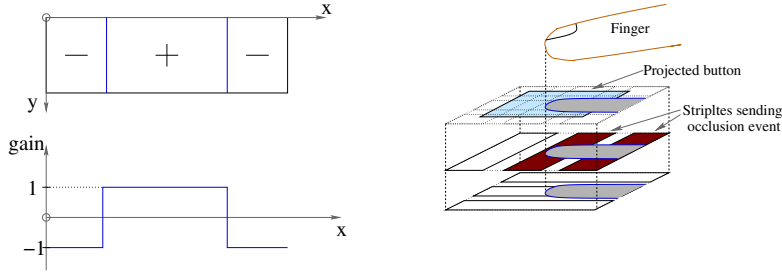
Figure 5.3: (a) Striplet gain function. (b) Button widget made of 6 striples.
