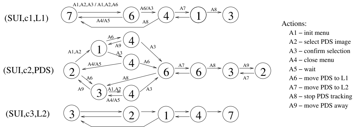
Figure 6.6: Coupling finite state automata for the PDS-based location control
