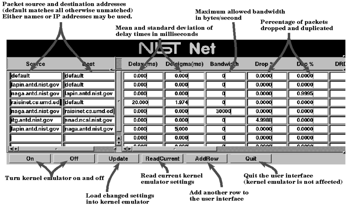
Figure 18: NistNet Interface
