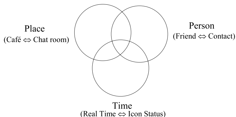
Figure 23: Synchronous interaction
