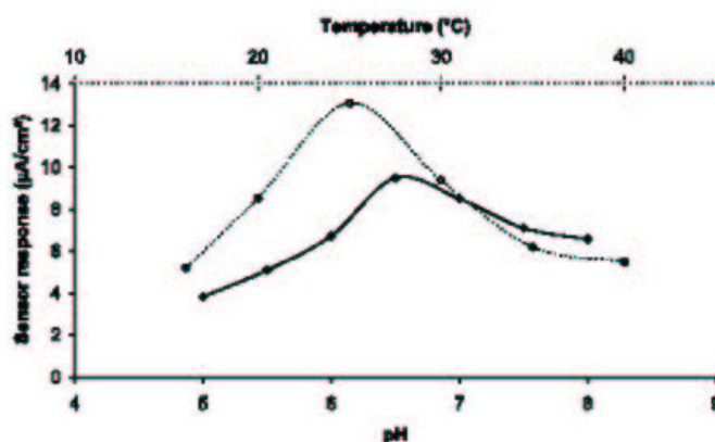
Fig. 4. Effect of temperature (---) and working pH (—) on PEDT/PPO electrode response to 5 \mu\text{M} catechol using preparation method A. Conditions: 0.1 M sodium phosphate buffer and 0.1 M KCl, 200 mV vs. SCE.
