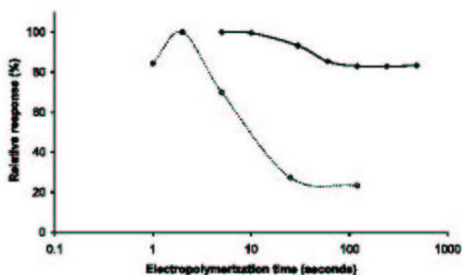
Fig. 3. Effect of electropolymerization time on PEDT/PPO electrode response to 5 \mu\text{M} catechol (—) using preparation method A and to 25 \mu\text{M} dopamine (---) using preparation method B. Conditions: 0.1 M, pH 6.5 sodium phosphate buffer and 0.1 M KCl, 25 °C, 200 mV vs. SCE.
