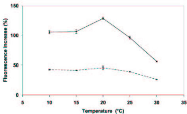
Fig. 5. Effect of temperature on the sensor response to 50 \mu\text{g l}^{-1} (----) and 1000 \mu\text{g l}^{-1} (—) of atrazine. Mean values from three membranes corresponding to three different continuous cultures were used to obtain the curves. Conditions: 10 mM, pH 7.0 phosphate buffer, 2 ml min -1 flow rate.
