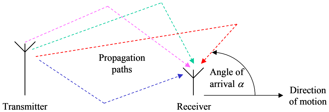
Figure 2-2: Sketch of signal arrival in a multi-path environment.
