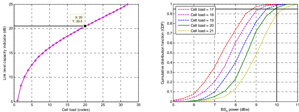
Figure 6-5: Link (left) and system (right) level approaches for capacity evaluation.
