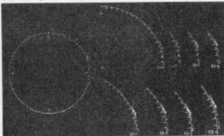
Figure 1. Evolution observed with HACOPIC (the H alpha coronagraph of the Pic du Midi observatory) : images taken on 1996-08-16 at respectively 06:05AM 06:12 06:16 06:32 06:37 06:47 06:59 07:17 (07:39 for the big image on the left hand side)
