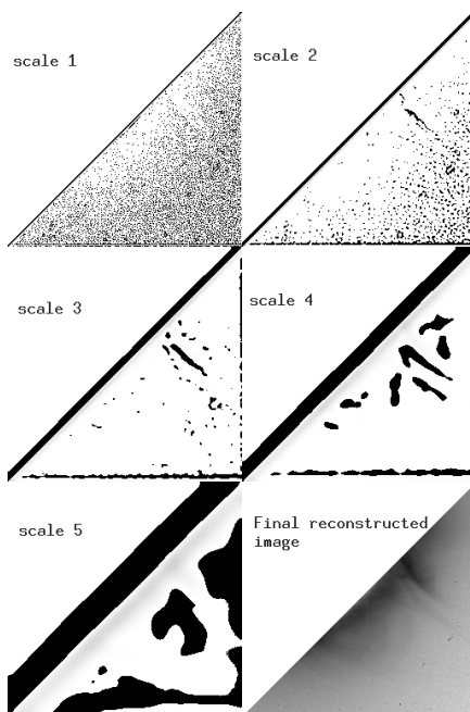
Figure 7. Wavelet reconstruction of the NOAA 8100, November 6th, 1997 : The 5 wavelet transforms planes and the rebuilt object (double Y shape)
