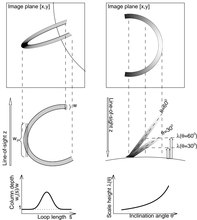
FIG. 9.—Left: The effect of the variable column depth w_z(s) measured parallel to the line of sight z is illustrated as a function of the loop length parameter s , for a loop with a constant diameter w . Right: The effect of the inclination angle \theta of the loop plane on the inferred density scale height \lambda(\theta) is shown. Both effects have to be accounted for the determination of the electron density n_e(s) along the loop.
