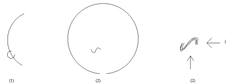
Figure 4. The 3D aspect of the NOAA 8027 deduced from the projection : (a) shape when the AR was at the limb : April 1st 1997, (b) AR on the disk
