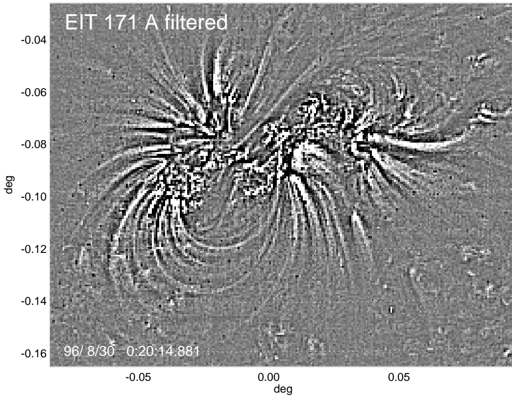
FIG. 1.— SOHO /EIT Fe IX/Fe X image of active region AR 7986, recorded on 1996 August 30, 0020:14 UT, at a wavelength of 171 Å, sensitive in the temperature range of T_e = 1.0\text{--}1.5 MK ( top ). The gray scales of the image is scaled logarithmically in flux, the contours correspond to increments of 100 DN (data numbers). The heliographic grid has a spacing of 5^\circ . The filtered image ( bottom ) was created by subtracting a smoothed image (using a boxcar of 3 \times 3 pixels) from the original image, in order to enhance the loop fine structure.
