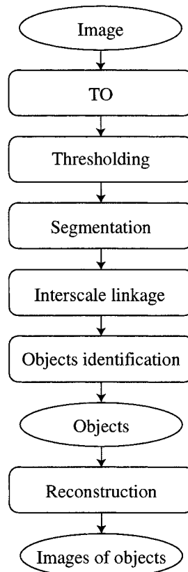
Figure 3. MVM algorithm.
