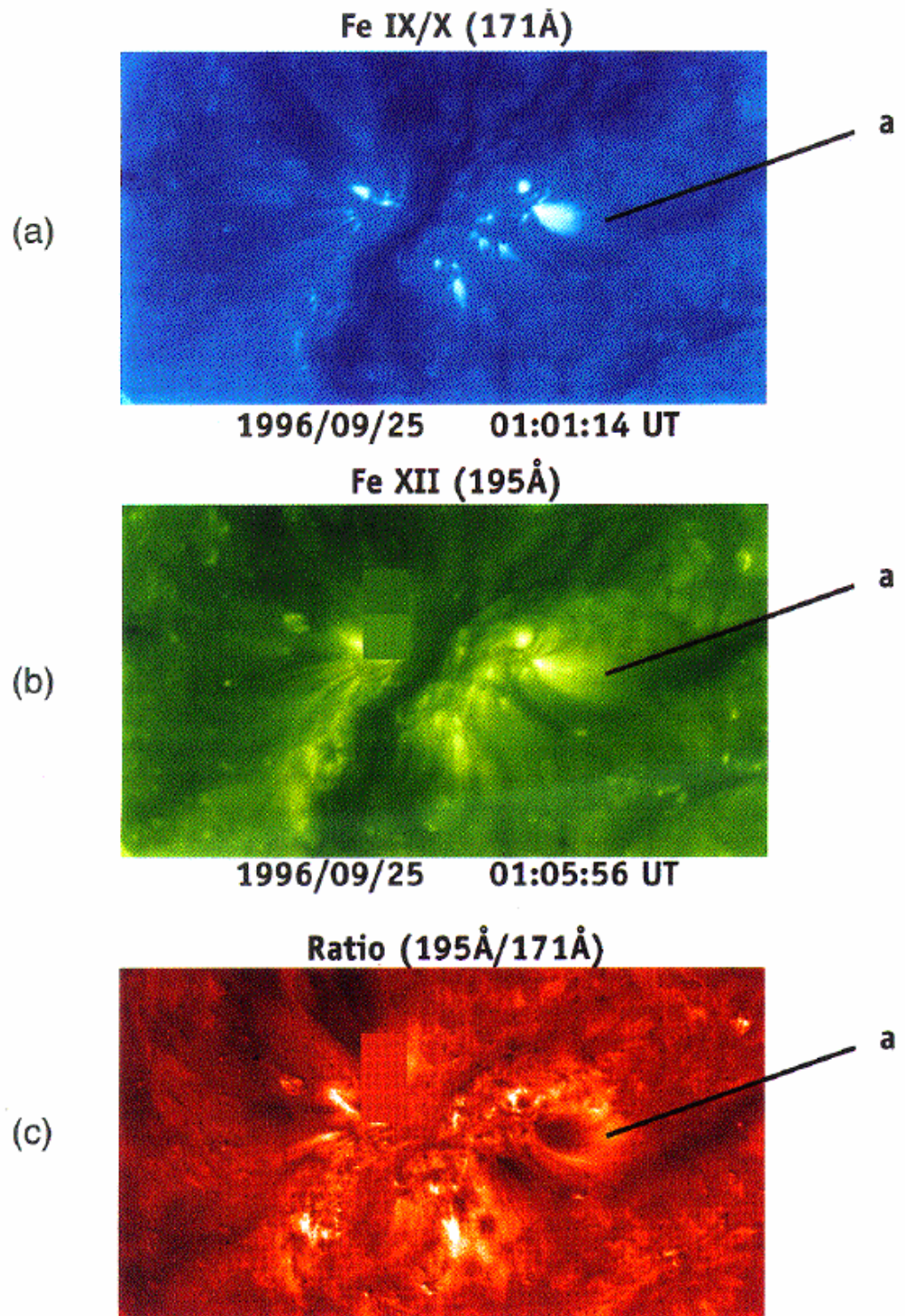
Figure 1. Observations of a decaying active region near the Central Meridian on 25 September 1996. (a) Fe IX/X emission; (b) Fe XII emission; (c) Ratio of the Fe XII and Fe IX/X images. The angular field of view of each image is 640 \times 1140 arc sec. A coronal loop feature selected for analysis is indicated. Two blocks of uniform color near the centers of frames (b) and (c) are fillers for data that are missing.
