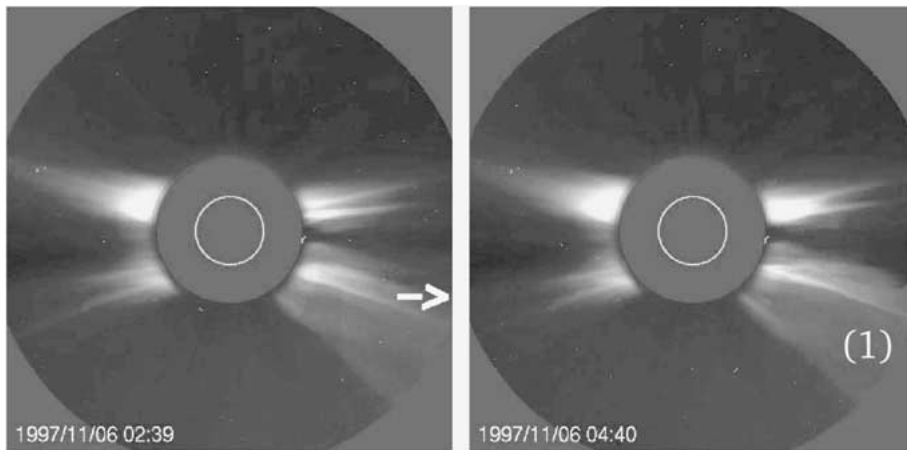
Figure 12. Coronagraphic LASCO C2 images taken on 6 November 1997 at 02:39 UT (left) and 04:40 UT (right). Outward materials follows the arrow. On the movie, we note that the escaping structure is twisted with an Y shape.
