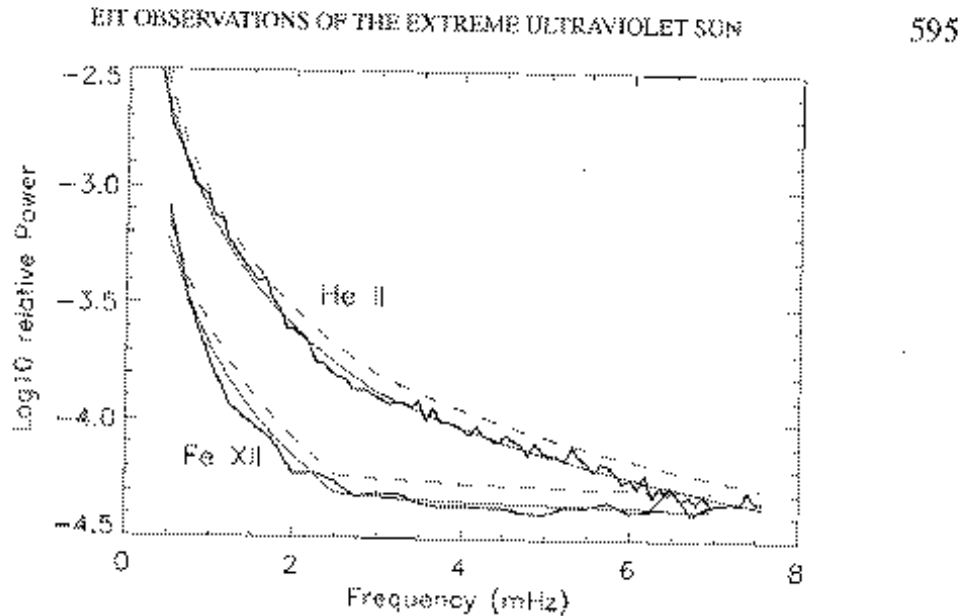
Figure 12. Average power spectra computed for the He II (304 Å) and Fe XII (195 Å) image sequences (full-field average). The thin lines represent the fitted f^{-3} profile, while the dashed lines show the 99.9 confidence levels.
