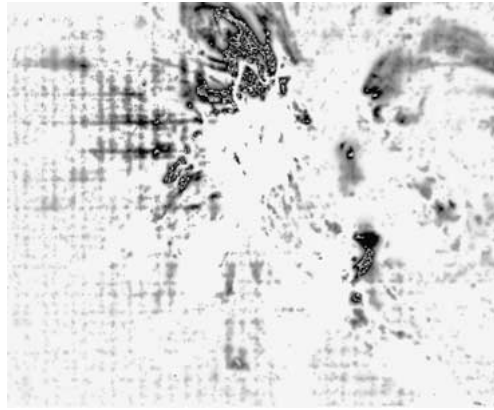
Figure 5. Magnification of the rebuilt wavelet image processed with the rough EIT image: The grid pattern appears clearly and hides some structures. Negative LUT.
