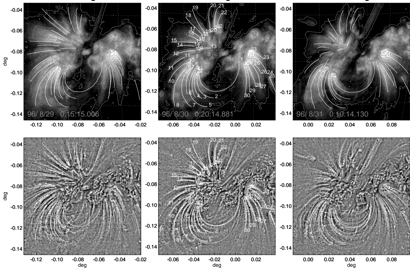
FIG. 4.—Projections of 30 stereoscopically reconstructed loop segments (numbered white curves) are shown overlaid on the SOHO /EIT 171 Å images ( top ) and the filtered images ( bottom ) of 1996 August 29 ( left ), 30 ( center ), and 31 ( right ). The 30 loop segments were traced from the filter image of August 30 ( bottom middle ), whereas the projections on the previous and following day were calculated from the inclination angles \mathcal{S} obtained from the dynamic stereoscopy method. Note that the overall magnetic field structure is almost invariant during the 3 days, but dynamic changes of the loops produce slight displacements between the calculated projections forward and backward in time and the actually observed fine structure.
