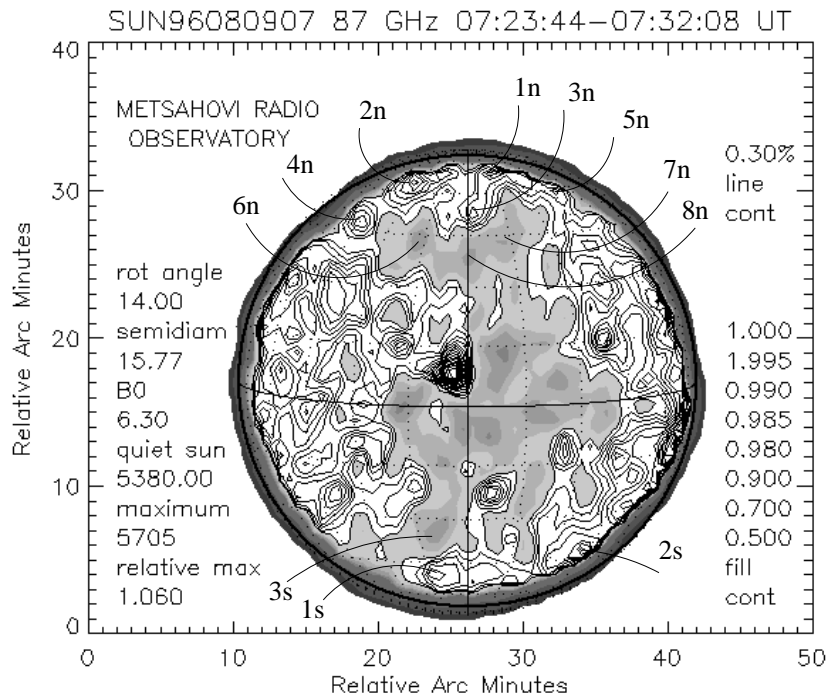
Fig. 8. Solar radio map at 87 GHz (3.5 mm) for August 09, 1996 at 07:23 – 07:32 UT. The greyscale contours (0.5, 0.7, 0.9, 0.98, 0.985, 0.99, and 0.995) represent levels below the quiet Sun. The quiet Sun (level 1.000) is plotted in white color, over which are the enhanced levels plotted in contour lines. The contour line level difference (0.3% of the quiet Sun in this case) is also the flux resolution
