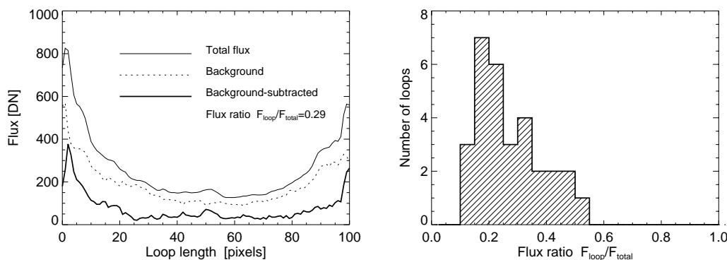
FIG. 7.—Loop-associated EUV flux [ F_{\text{loop}}(s) , thick line ], the total EUV flux [ F_{\text{total}}(s) , thin line ], and the background [ F_{\text{total}}(s) - F_{\text{flux}}(s) , dotted line ] measured along the loop is shown for loop 1 ( left ). A histogram of the relative fractions F_{\text{loop}}/F_{\text{total}} (integrated over the traced loop lengths) is shown from all 30 analyzed loops ( right ).
