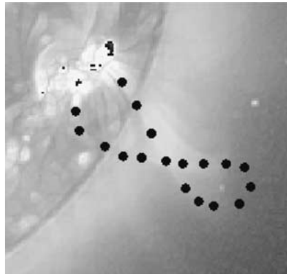
Figure 11. Aspect of NOAA 8100 with SOHO/EIT Fe XII (195 Å) on 5 November, 1997 at 23:02 UT. We emphasized the structure which is a twisted loop (as analyzed with a ‘stereoscopic’ method) (Portier-Fozzani, 1999).
