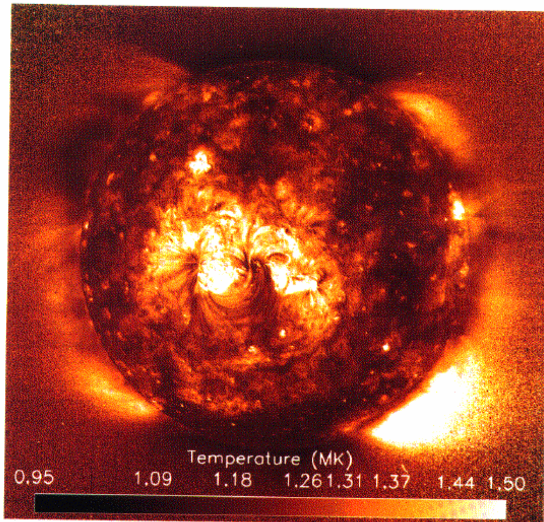
Figure 8. Temperature map derived from ratio of Fe XII and Fe IX, \lambda from 12 May 1996
