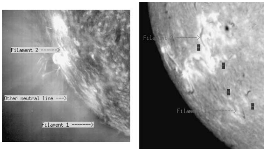
Figure 14. Aspect of the area NOAA 8194 and 8195 and their filaments with multi-wavelength observations on 8 April, 1998. Left : SOHO/EIT He II ( 304 \text{ \AA} ) at 17:00 UT. Right : Meudon spectroheliograph H\alpha .
