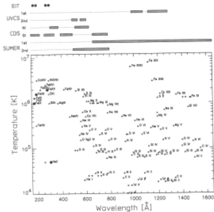
Figure II.12: Spectres des instruments UV de SOHO ([79])
