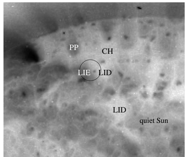
Fig. 1. Polar region on August 27, 1997, at 13:01:03 UT in Fe IX/X line (reversed colours). The circle has 1 arcmin radius and shows the size of the radio beam. Depending on the location, there is a possibility of having several EUV structures within the beam. This location was classified as a local intensity enhancement (LIE, in dark colour), although it is nearby a local intensity decrease area (LID, in white colour). The contrast in the image has been enhanced, to show more clearly all the tiny EUV structures
