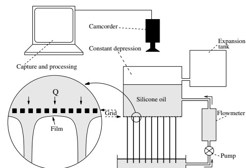
FIG. 1. Schematic representation of the experimental setup, with an enlargement of the grid and the film underneath.
