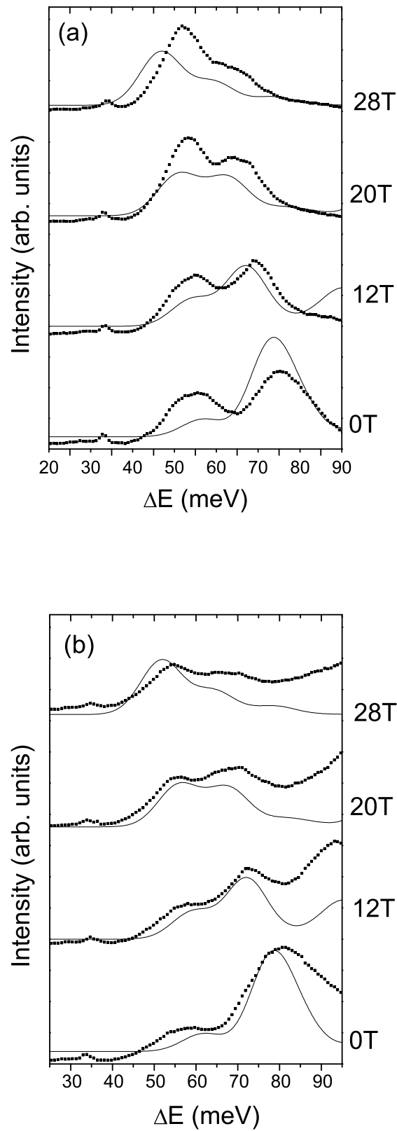
Figure 5.12: Experimental (full symbols) and calculated (solid lines) spectra for different magnetic fields. The experimental data was taken for E_{exc} = 1260 meV (a) and E_{exc} = 1293 meV (b), for sample P3. The parameters used in the calculation are given in the text.
