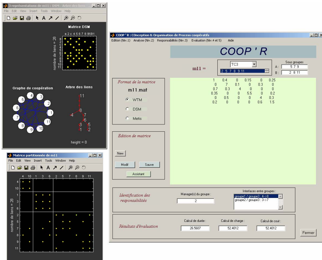
Figure 5.3 : L'outil COOP'R
