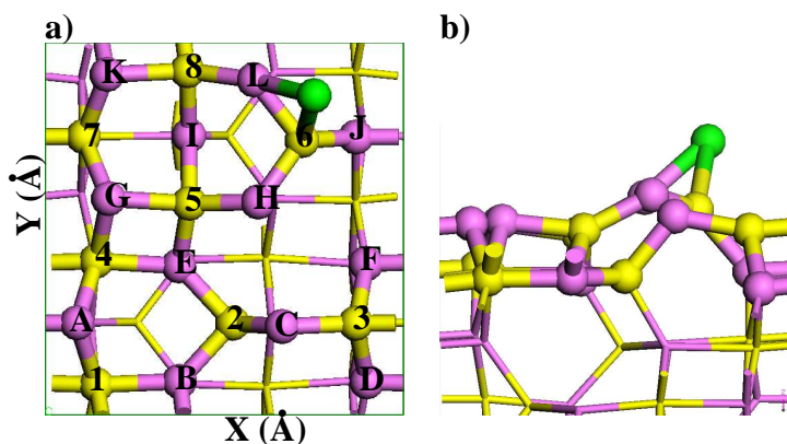
Figure 4.9: Pd adsorption on the dehydrated \gamma -Al 2 O 3 (110) surface at the \mu_2 O(L)-Al III (6) site: a) top view, b) side view. Eads = -1.86 eV. Yellow balls: Al, violet balls: O, green balls: Pd. The configuration involving O(H) is of course equivalent.
