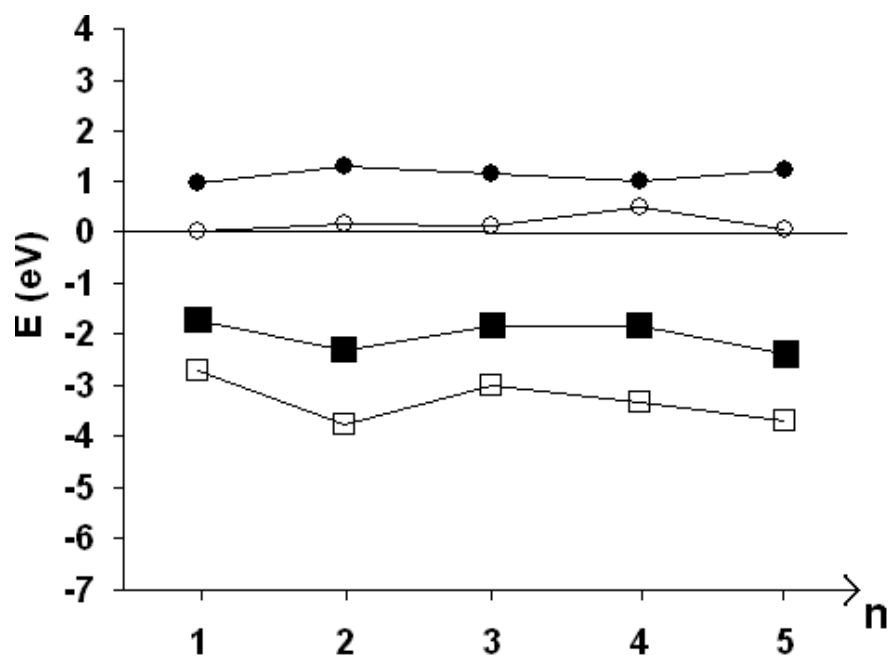
Figure 6.6: E_{ads} , E_{int} and deformation energies of Pd_n clusters on the hydrated \gamma\text{-Al}_2\text{O}_3(110) surface: ■ E_{ads} , □ E_{int} , ● E_{def. Surface} and ○ E_{def. Pd_n} .
