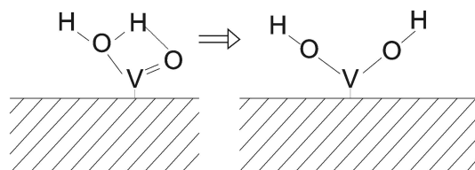
Figure 8.11: Model for the dissociative water adsorption on \text{O}=\text{V}_2\text{O}_3(0001) . Only the surface vanadium and the oxygen of the vanadyl are shown
