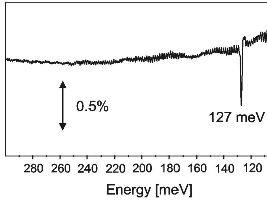
Figure 5.11: IRAS: spectrum for -V=O termination divided by spectrum for -V termination. The absorption peak corresponds to the V-O stretching vibration of the vanadyl groups
