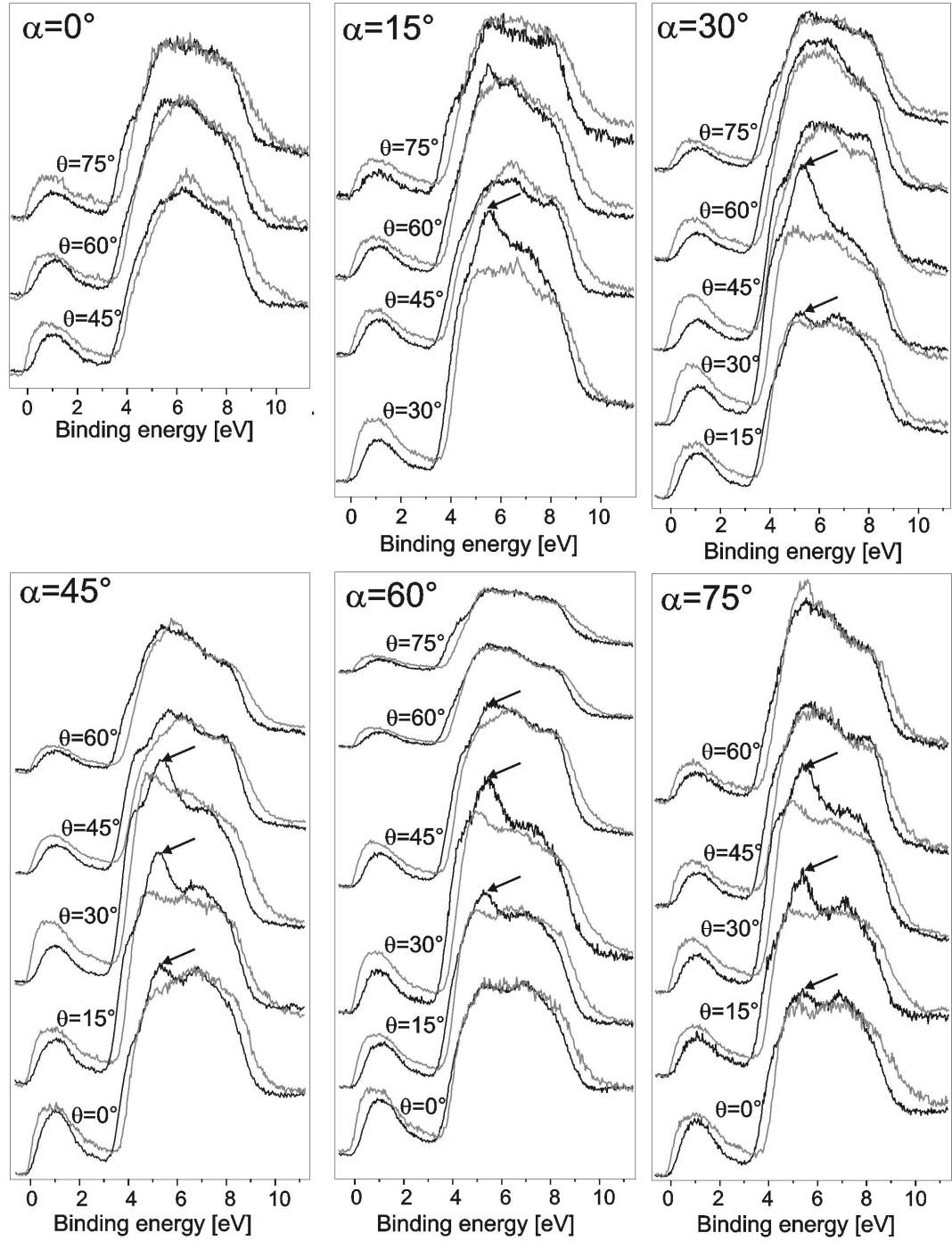
Figure 6.2: ARUPS on V_2O_3(0001)/Au(111) for the -V (grey) and -V=O (black) terminations - \alpha is the light angle of incidence and \theta the angle of detection
