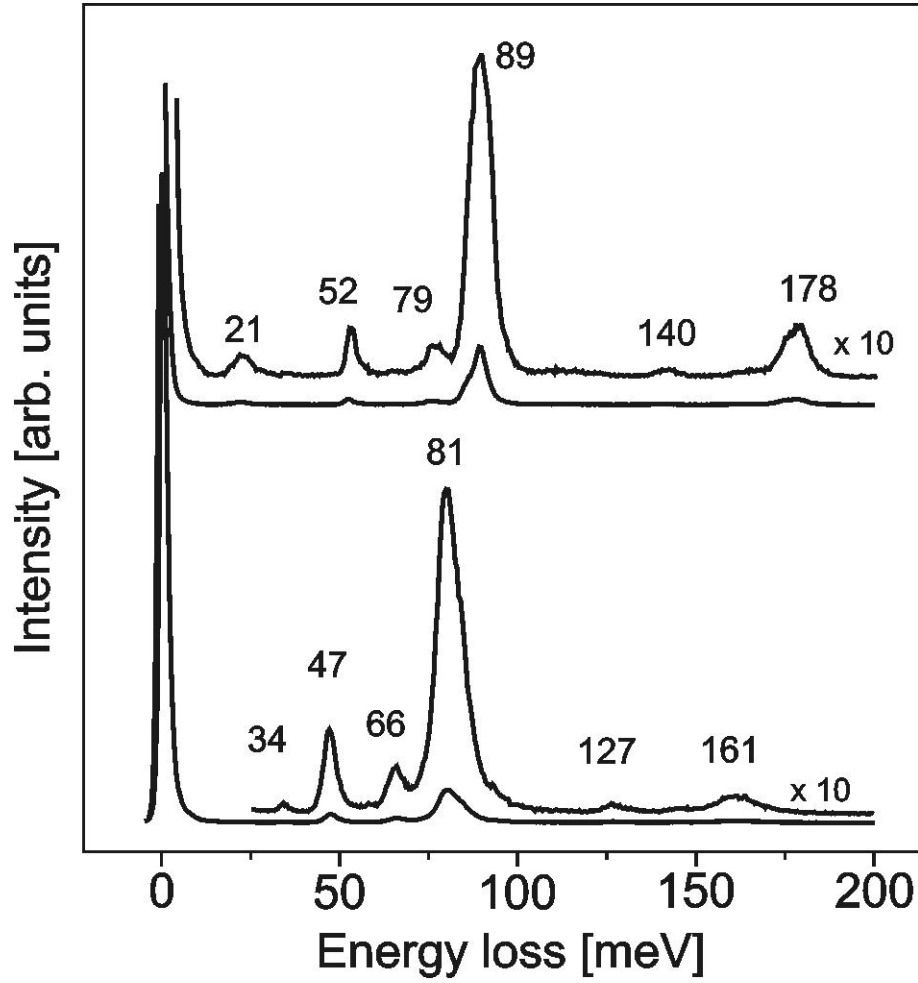
Figure 7.1: HREELS of Cr_2O_3(0001)/Cr(110) from [101] (top) and V-V_2O_3(0001)/W(110) (bottom)
