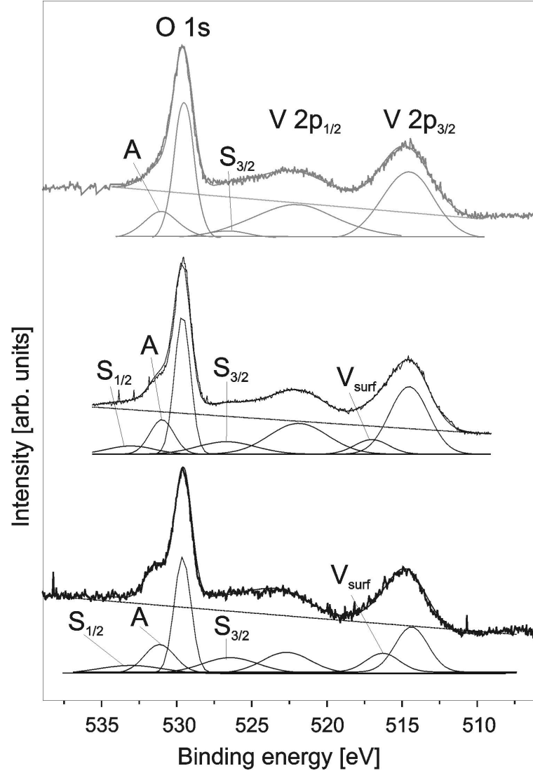
Figure 6.7: XPS of V_2O_3(0001)/Au(111) for -V termination at normal emission (grey, top) and -V=O termination (black) at normal emission (middle) and at emission angle 60^\circ (bottom)
