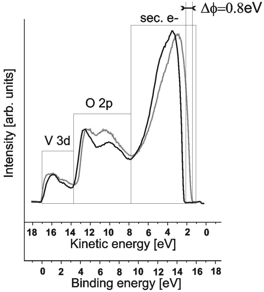
Figure 6.1: UPS (HeI) on \text{V}_2\text{O}_3(0001)/\text{Au}(111) for the -\text{V} (grey) and -\text{V}=\text{O} (black) terminations at normal emission. The difference of the low energy cutoff corresponds to the difference of the work function between the two terminations
