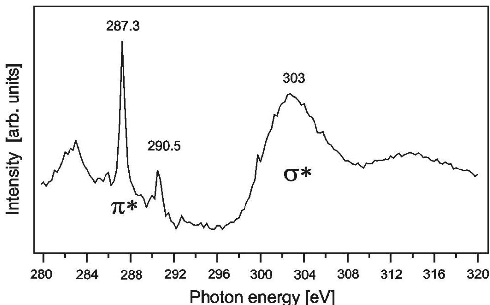
Figure 10.6: NEXAFS spectrum of 20 L CO/-V terminated \text{V}_2\text{O}_3(0001)/\text{Au}(111) taken in the Auger yield mode at 90 K and with light incident normal to the surface.
