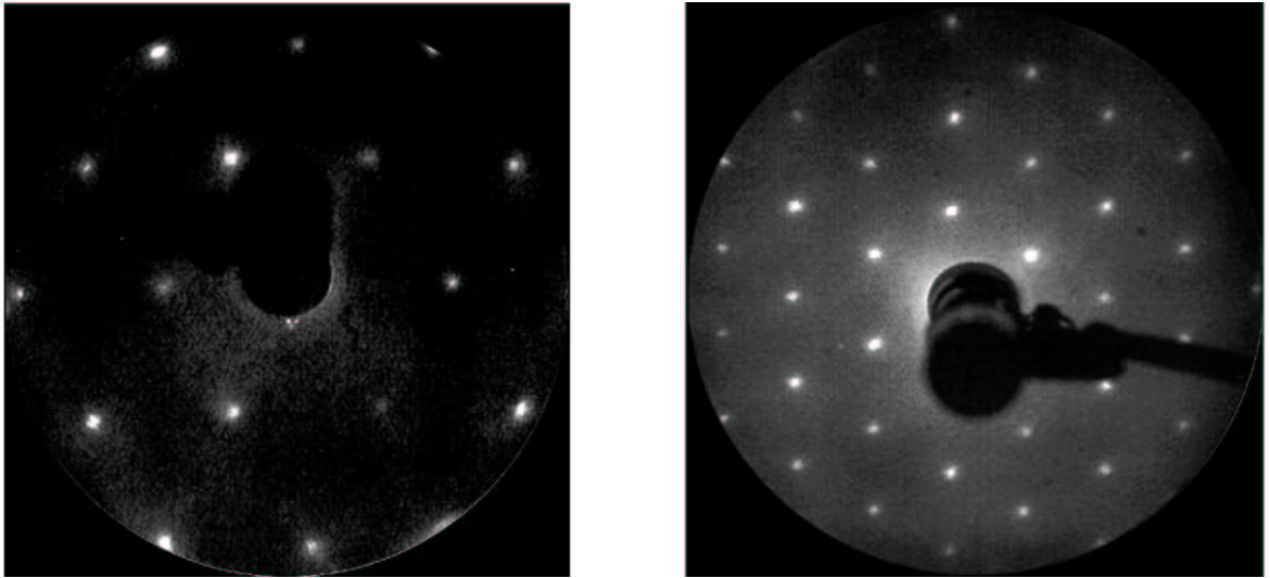
Figure 5.5: LEED pattern of the Au(111) substrate at 175 eV (left) and \text{V}_2\text{O}_3(0001)/\text{Au}(111) at 150 eV (right)
