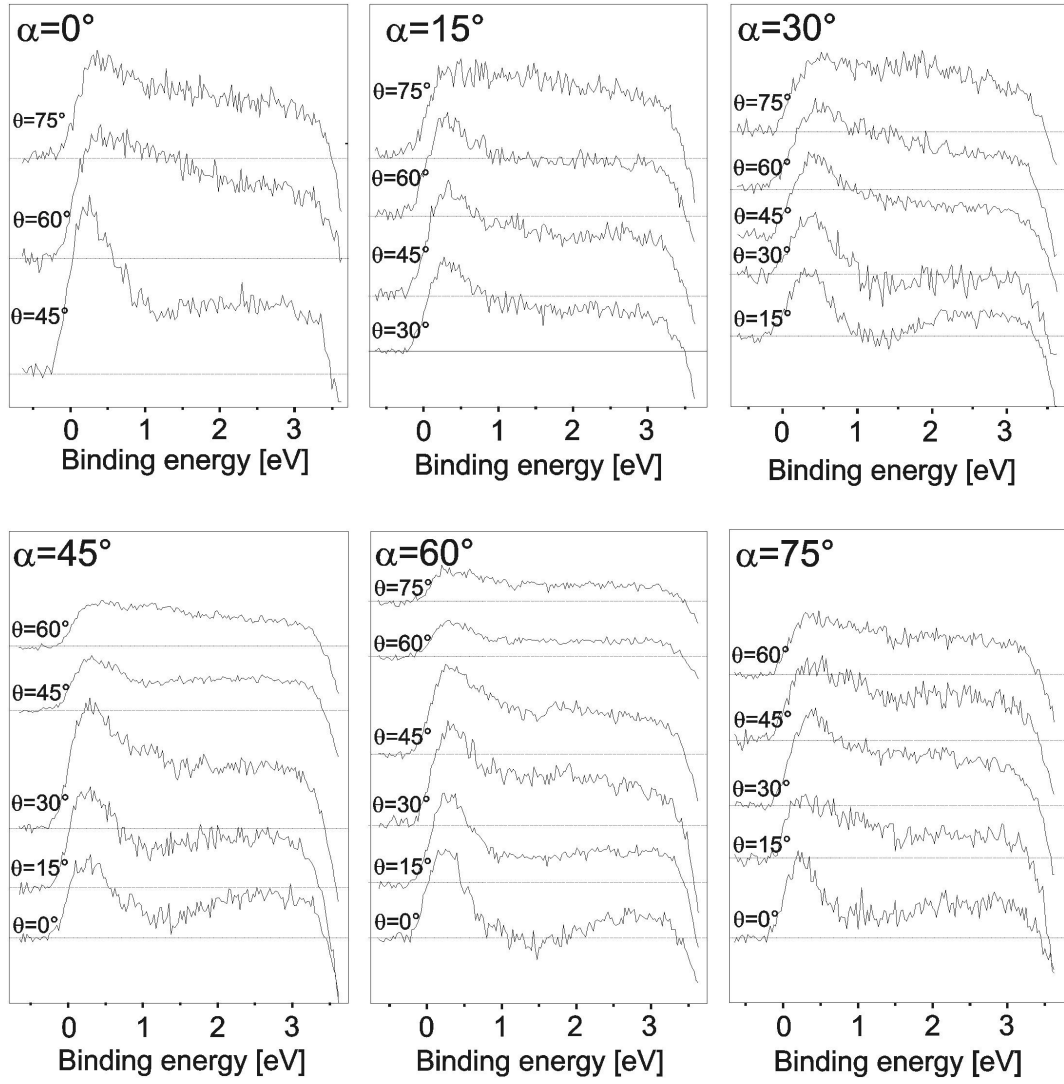
Figure 6.4: Difference spectra in the V 3d region. (-V surface) minus (-V=O surface)
