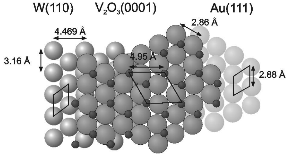
Figure 5.4: Lattice parameter for the epitaxial growth of \text{V}_2\text{O}_3(0001) on W(110) (left) and Au(111) (right)
