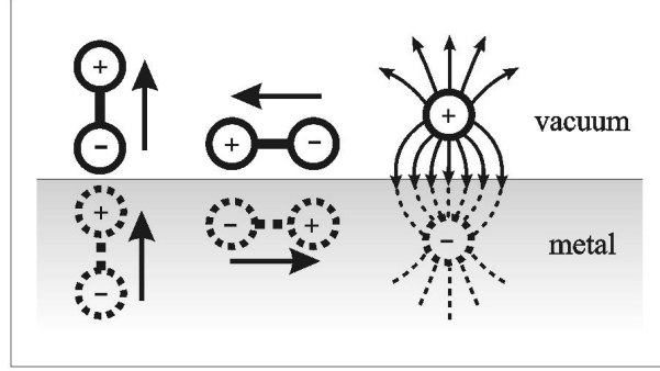
Figure 3.9: Schematic illustration of dipole screening on metal surfaces
