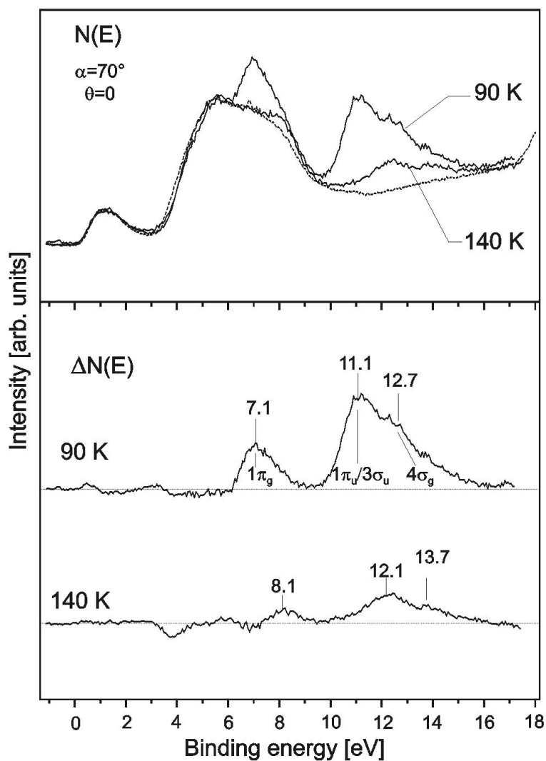
Figure 9.6: UPS HeII - Top: 20 L O 2 /V terminated V 2 O 3 (0001)/Au(111) (dashed line) and 20 L CO 2 on this O 2 precovered surface at the temperatures indicated. Bottom: corresponding difference spectra. \alpha is the angle of incidence of light and \theta is the detection angle
