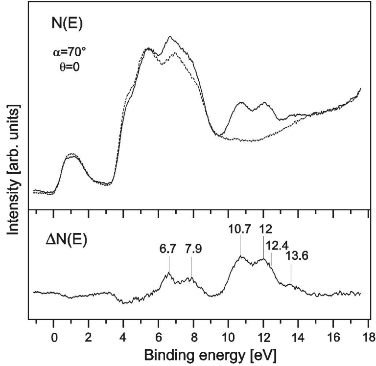
Figure 9.7: UPS HeII - Top: clean -V=O terminated V_2O_3(0001)/Au(111) after 30 min. heating to 650 K without electron bombardment (dashed line) and 20 L CO_2 on this surface (solid line) at 90 K. Bottom: corresponding difference spectra. \alpha is the angle of incidence of light and \theta is the detection angle
