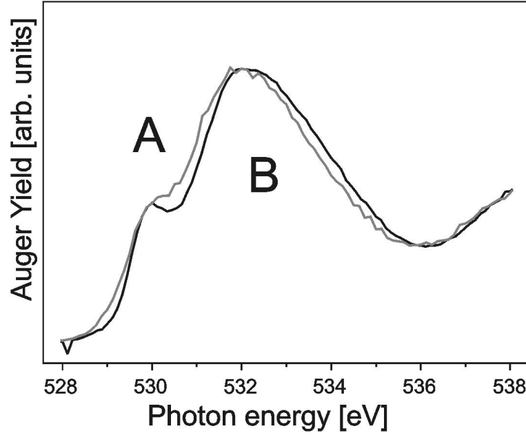
Figure 6.8: NEXAFS - O K-edge for \text{V}_2\text{O}_3(0001)/\text{Au}(111) for -V (grey) and -V=O (black) surface terminations
