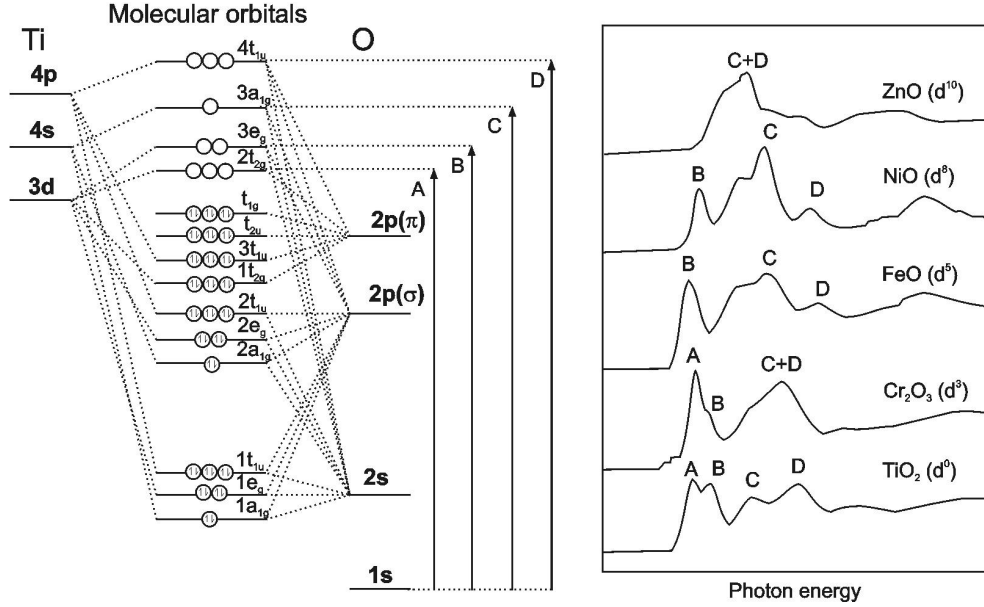
Figure 3.7: Schematics of molecular orbitals of a \text{TiO}_6^{8-} cluster modelling \text{TiO}_2 in an octahedral symmetry (left) and oxygen K-edge NEXAF spectra of several 3d transition metal oxides from [35] (right)
