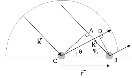
Figure 3.2: Bragg interpretation of diffraction: \delta = AB - CD = r(\cos \varphi - \cos \theta) = n\lambda
