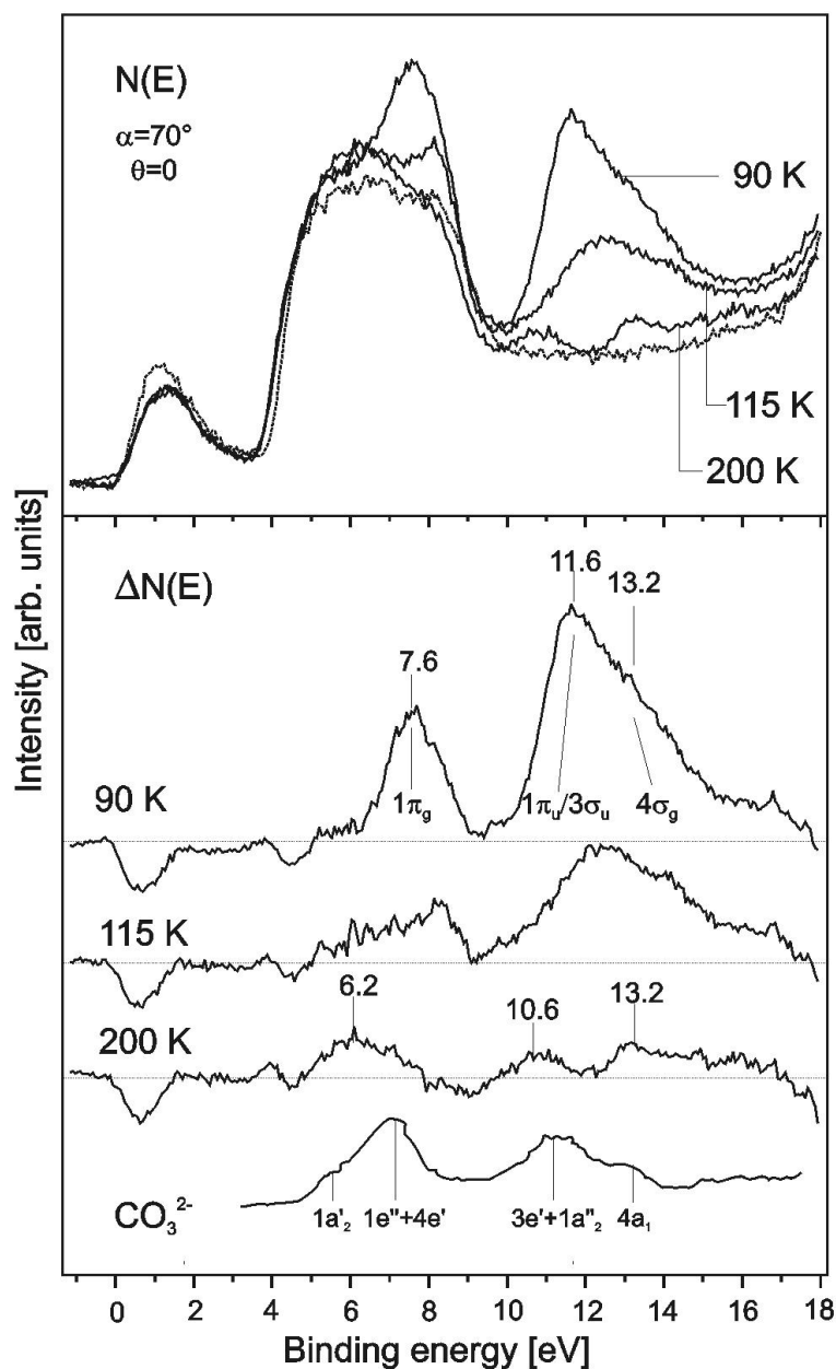
Figure 9.4: He II UP spectra - Top: clean (dashed line) and 20 L \text{CO}_2 -V terminated \text{V}_2\text{O}_3(0001)/\text{Au}(111) (solid line) at the temperatures indicated. Bottom: corresponding difference spectra. \alpha is the angle of incidence of light and \theta is the detection angle
