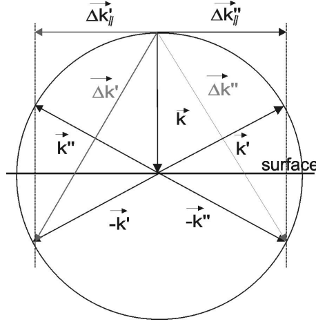
Figure 3.3: Diffraction by LEED
