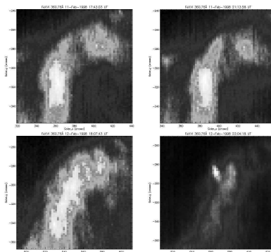
Figure 8. Evolution of the S-shaped structure in Fe XVI at 360\text{\AA} (fov : 122'' \times 119'' ): 11 February at 17:43 UT (top left), 11 February at 21:14 UT (top right), 12 February at 18:07 UT (bottom left), 12 February at 22:04 UT (bottom right).
