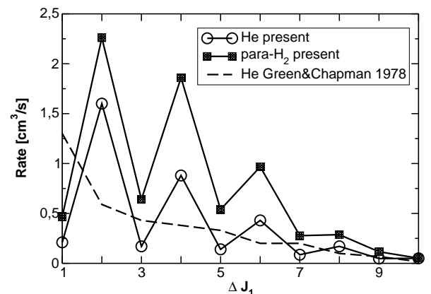
Fig. 3. HC 3 N–He and HC 3 N–H 2 collisions. Quantum close coupling excitation rates, from J_1 = 0 , at 20 K. Dashed lines, QCT HC 3 N–He calculations (Green & Chapman 1978); full lines, present calculations for He and H 2 .
