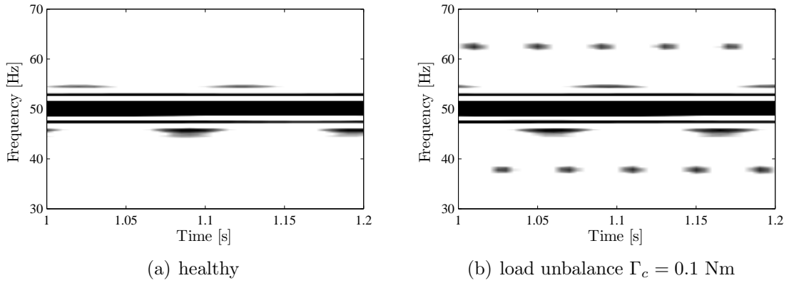
Figure 5.30: PWD of stator current in healthy case and with load unbalance ( \Gamma_c = 0.1 Nm), 50% load.
