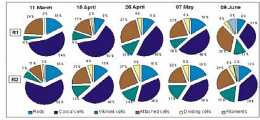
Figure 4 : Seasonal evolution of the main bacterial morphotypes from March to June 2002.
