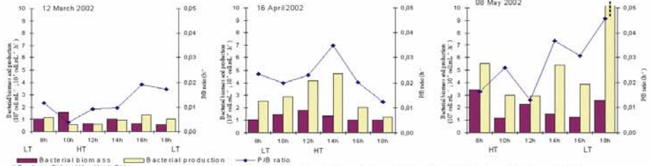
Figure 2 : Daily evolution of bacterial dynamics from March to May 2002. (Data from the inshore point PC)
