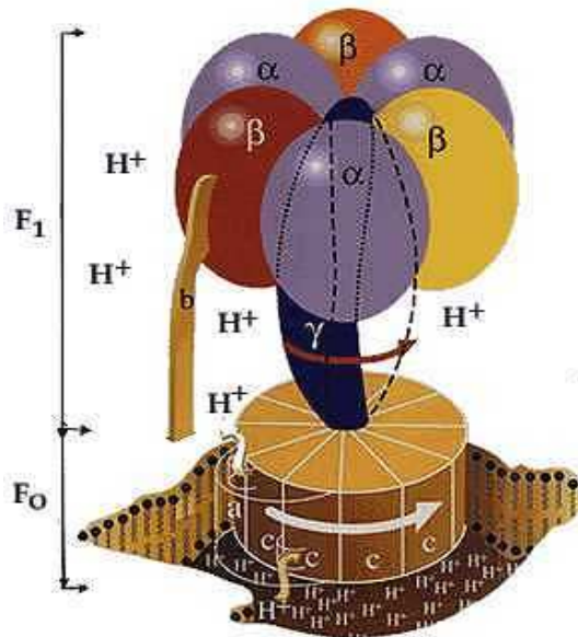
Figure 11 : Structure de la MgATP synthase.
