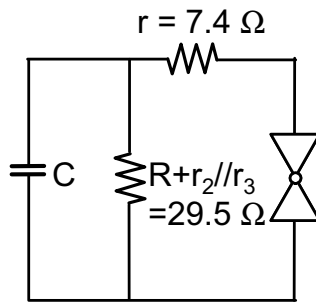
Figure 22: Simplified environment seen from the contact.
