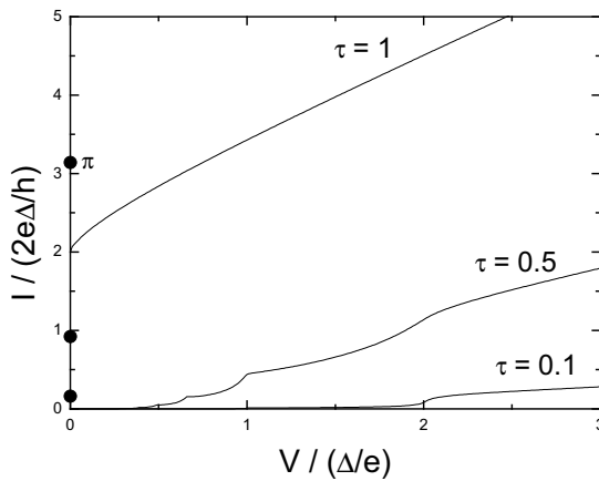
Figure 14: MAR current (lines) and critical current (dots) in channels of various transmissions under perfect voltage bias V .
