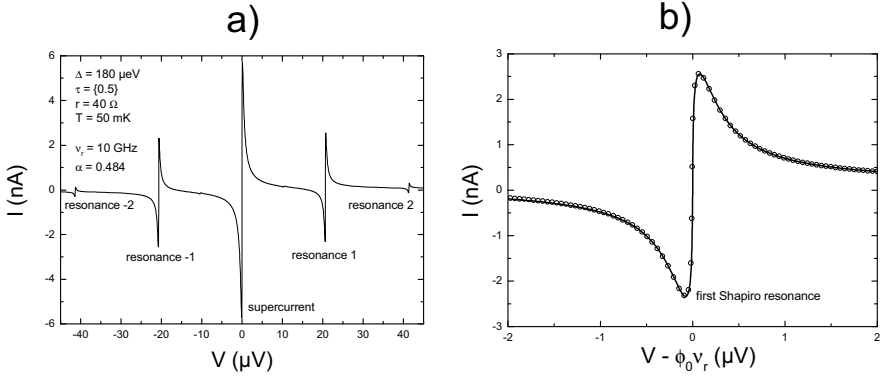
Figure 12: Calculated IV characteristic of a single channel contact ( \tau=0.5 ) in presence of microwave ( \nu_r=10 GHz, \alpha=0.484 ). a): large scale IV calculated within the Fokker-Planck approach. The Shapiro resonances 1 and 2 are visible. b): Zoom on the first Shapiro resonance to compare the predictions of the mapping approach (solid line) with the predictions of the Fokker-Planck calculation (open dots). \phi_0 = h/(2e) is the flux quantum.
