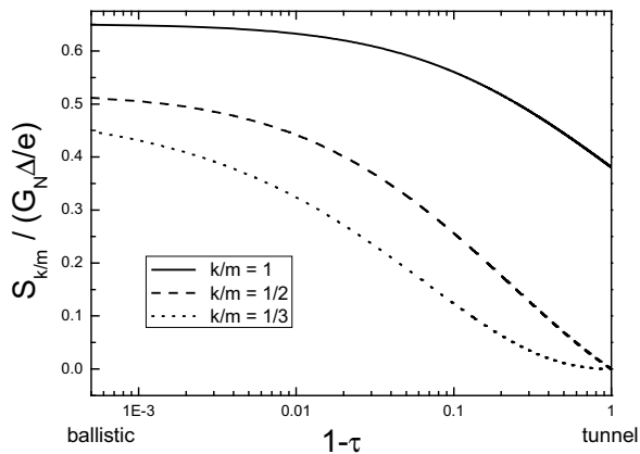
Figure 6: Amplitude of the Shapiro resonances k/m=1, 1/2, 1/3 as a function of the channel transmission, calculated within the adiabatic approximation for \alpha=0.25 . Note the horizontal axis: data are plotted as a function of the reflection coefficient ( 1-\tau ) on a logarithmic scale to highlight the high transmissions. G_N = (2e^2/h)\tau is the normal state conductance of the channel.
