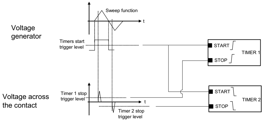
Figure 31: Schematic representation of the setup for measuring the switching current.
