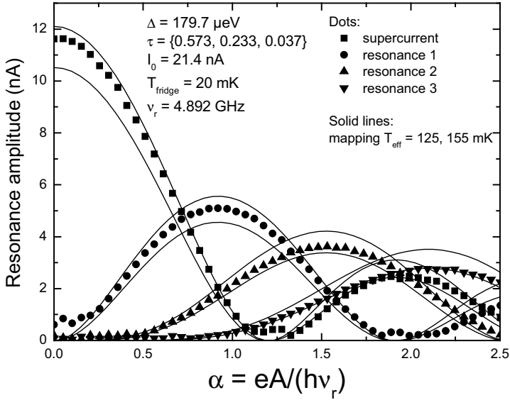
Figure 28: Dependence of the Shapiro resonance amplitudes with the microwave power. Squares: supercurrent. Circles: first resonance. Up-triangles: second resonance. Down-triangles: third resonance. The upper (resp. lower) solid lines are the theoretical predictions at 125 mK (resp. 155 mK).
