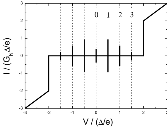
Figure 4: Integer Shapiro resonances p/q=1, 2, 3 and supercurrent peak p/q=0 in a tunnel junction ( \alpha=1 and \omega_p=\Delta/\hbar ). G_N is the normal state conductance of the tunnel junction.
