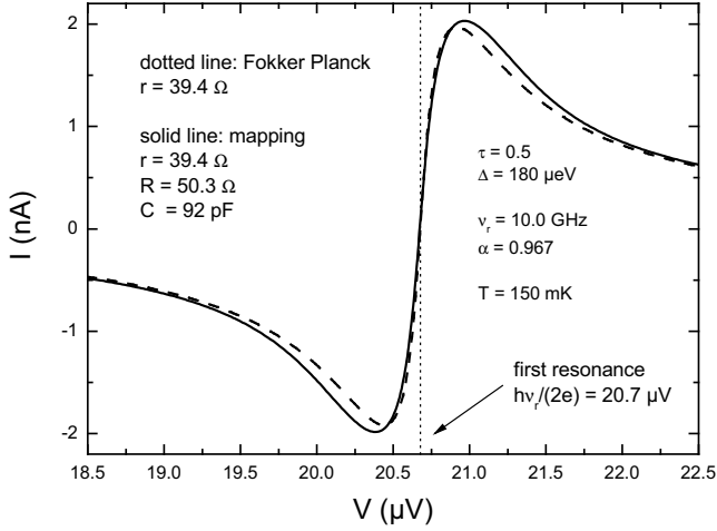
Figure 26: Comparison of two theoretical predictions for the first Shapiro resonance of a \tau=0.5 single channel contact. Dashed line: predictions of the Fokker-Planck treatment of the dynamics of the phase in an ohmic environment ( r = 39.4 \Omega ). Solid line: predictions of the mapping approach for the environment of Figure 25.
