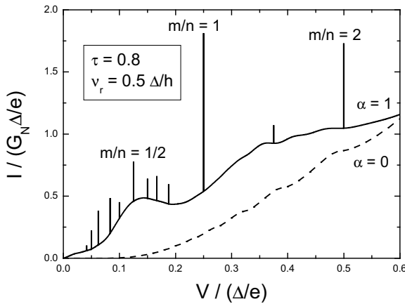
Figure 15: dc IV characteristic of a single channel contact ( \tau=0.8 ). The dashed line is the IV without microwave ( \alpha=eA/(h\nu_r)=0 ). The solid line is the IV with \alpha=1 . G_N=(2e^2/h)\tau is the normal state conductance of the contact (reproduced from [7]).
