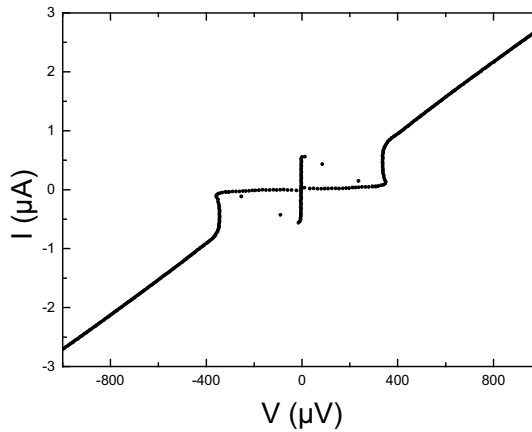
Figure 4: IV characteristic of an atomic contact SQUID.
