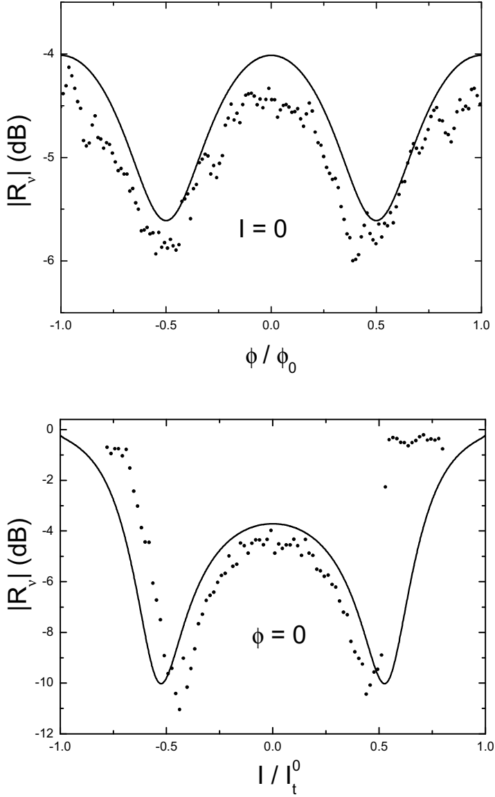
Figure 9: Modulus of the reflection coefficient R_v for a contact with mesoscopic pin code \tau = \{0.475, 0.138, 0.019\} . The fridge temperature was 20 mK. Lower graph: modulus as a function of the dc bias current I at \phi = 0 . Upper graph: modulus as a function of the external magnetic flux \phi threading the loop at I = 0 . Dots: experimental data. The full lines are the zero temperature theoretical predictions of equation (10).
