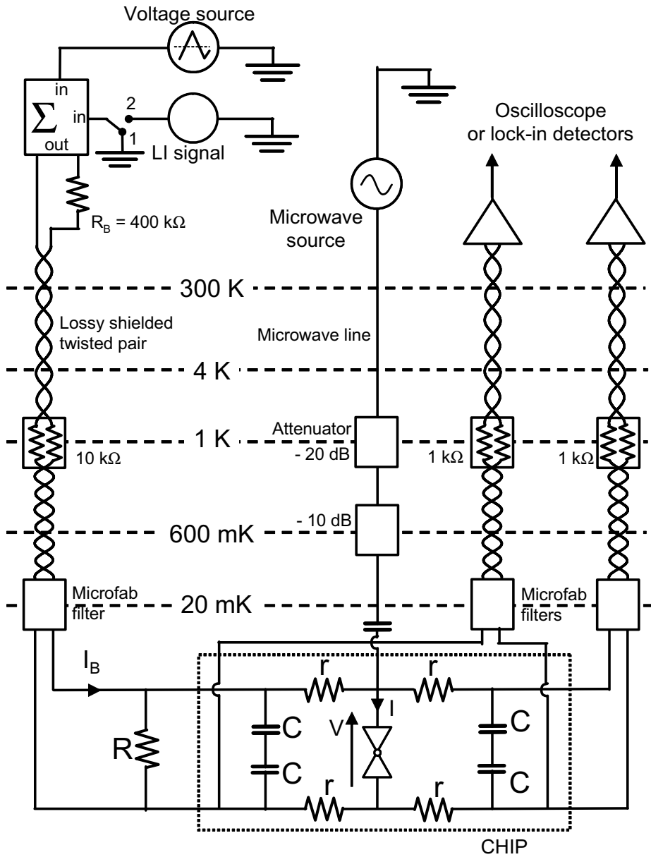
Figure 15: Detailed wiring of the experimental setup for measuring I - V characteristics both in the supercurrent peak and in the ac Josephson currents experiments with a FET amplifier to measure the current. The box \Sigma represents a bipolar summing amplifier.
