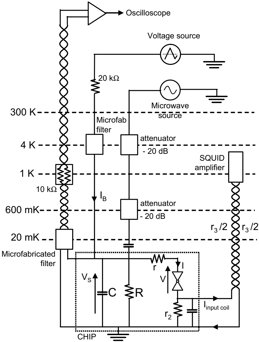
Figure 18: Experimental setup used for the measurement of Shapiro resonances with a SQUID as an ammeter. For biasing the sample, a coaxial line with a lossy part between 4 K and 20 mK is used. A microfabricated filter (dc resistance \sim 1 \text{ k}\Omega ) has been placed at 4 K, a refrigerator stage with sufficient cooling power to absorb the heat produced by Joule effect. The voltage V_S is measured with a lossy shielded twisted pair line to avoid thermoelectric voltages.
