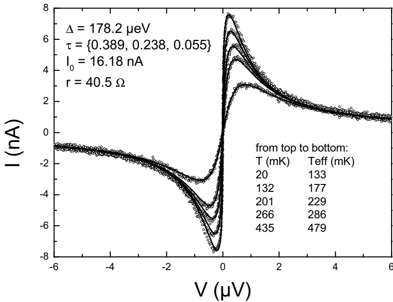
Figure 26: Supercurrent peaks of contact #5 and corresponding fits with the Ivanchenko Zil'berman result at different temperatures. The fridge temperature T and the corresponding fit temperature T_{\text{eff}} are indicated on the graph for each curve.
