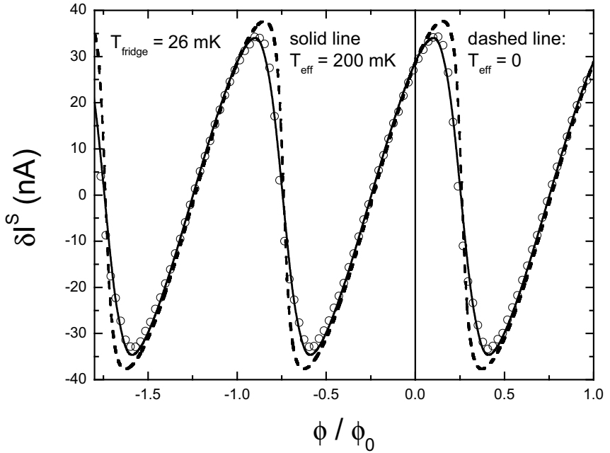
Figure 9: Modulation \delta I^S of the SQUID mean switching current as a function of the external flux \phi threading the loop. Dots are experimental results. The measurements were performed at 26 mK. Lines are theoretical predictions calculated from the independently measured mesoscopic pin code of the contact ( \tau = \{0.983\} ). The dashed line is the zero temperature prediction. The solid line is the prediction at an effective noise temperature of 200 mK.
