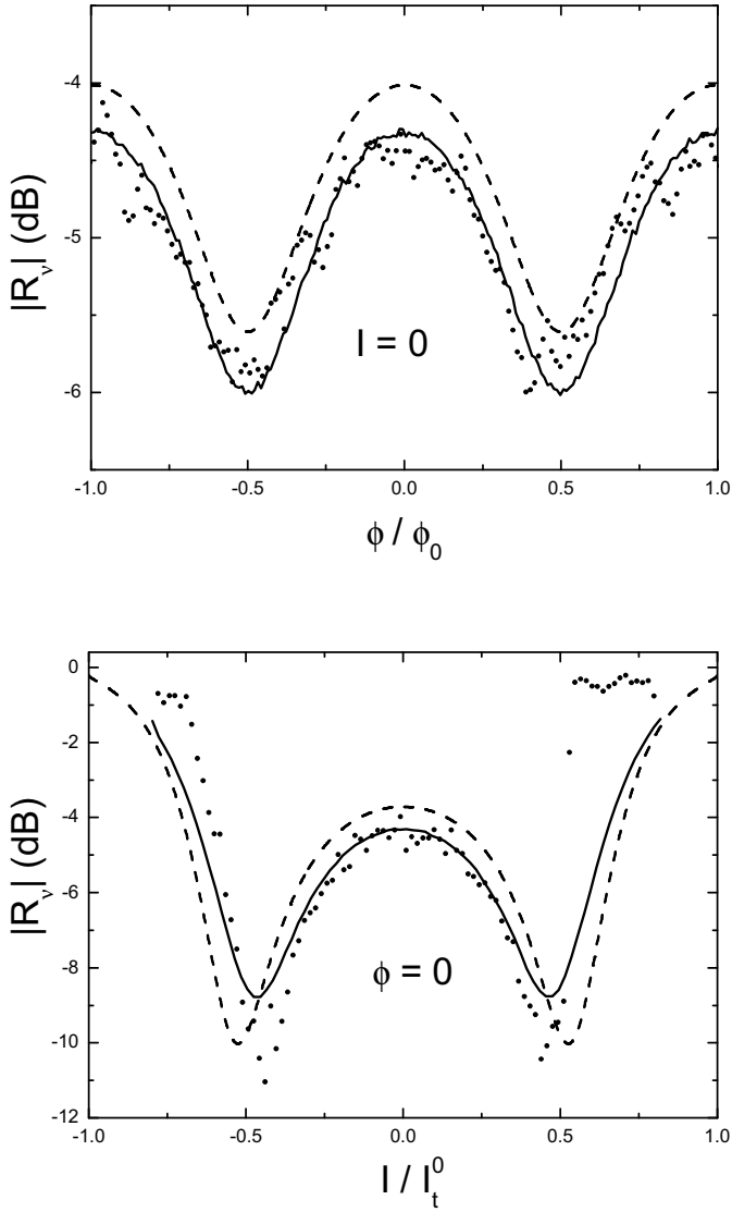
Figure 17: Modulus of the reflection coefficient R_v for a contact with mesoscopic pin code \tau = \{0.475, 0.138, 0.019\} . The fridge temperature was 20 mK. Lower graph: modulus as a function of the dc bias current I at \phi = 0 . Upper graph: modulus as a function of the external magnetic flux \phi threading the loop at I = 0 . Dots: experimental results. Dashed lines: zero temperature prediction of the linear approximation presented in section 3.2. Solid lines: zero temperature prediction of the numerical simulation of the phase dynamics.
