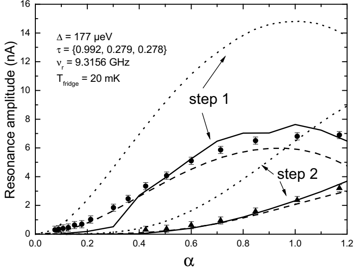
Figure 30: Power dependence of Shapiro resonances 1 and 2 for a contact containing a highly transmitting channel. Closed circles: experimental data. Dotted lines: adiabatic approximation (see section 2.1). Dashed lines: empiric calculation (see section 3.1.1). Solid lines: full microscopic calculation (see section 3.1.2.). In the three theoretical predictions, the effects of the temperature and of the environment are taken into account via the mapping approach (see section 2.2.1 & 3.2) with an effective noise temperature of 200 mK. The experiment was performed at the fridge base temperature (20 mK).
