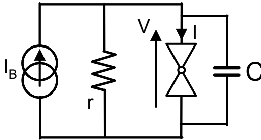
Figure 6: Electromagnetic environment of the RCSJ model.
