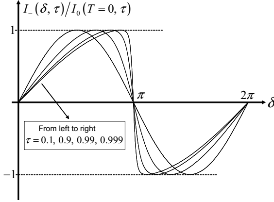
Figure 1: Current phase relation of the Andreev ground state for different transmissions ( \tau=0.1, 0.9, 0.99, 0.999 ) of the channel. The current phase relations have been normalized to their respective zero temperature critical currents I_0(T=0, \tau) (see below).
