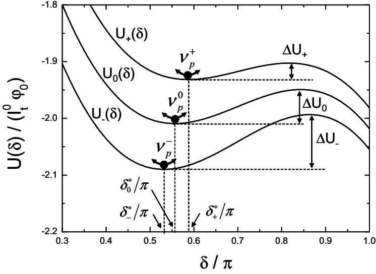
Figure 14: The three tilted washboard potentials U_{\pm}(\delta, I = 0.9I_t^0, \phi = 0.1\phi_0) and U_0(\delta, I = 0.9I_t^0, \phi = 0.1\phi_0) .
