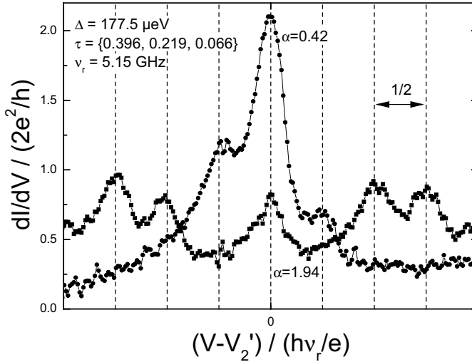
Figure 36: Measured differential conductance around V_2' = 0.98 \times 2\Delta / (2e) of an atomic contact for two different values of the microwave power. The satellite peaks correspond to a single Andreev reflection assisted by one, two or three photon(s).
