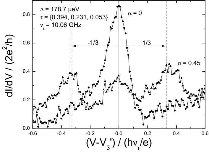
Figure 37: Measured differential conductance around V_3' = 0.98 \times 2\Delta / (3e) of an atomic contact for two different values of the microwave power. The satellite peaks correspond to a charge transfer process involving two Andreev reflections, each one assisted by a single photon.
