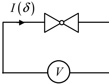
Figure 1: Atomic contact (double triangle symbol) with a perfect voltage bias V .
