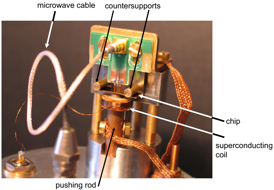
Figure 3: Photograph of the bending mechanism. The chip is placed between two counter-supports (small horizontal cylinders, 14 mm apart from each other) and a pushing-rod. Spring probes pressed on millimetric pads on the chip connect the sample through a 50 \Omega line to the external signals. A small superconducting coil (400 turns of niobium wire of 0.2 mm in diameter) has been added on the pushing rod to apply a magnetic field on the sample.
