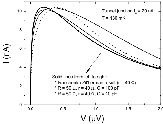
Figure 18: IV characteristics of a tunnel junction embedded in a r + ((r + R) // C) environment for different values of the capacitor C (The “+” symbolizes the series combination of two elements, whereas the “//” represents the parallel combination.). The dotted line is the prediction of the single frequency model for C = 10 pF.
