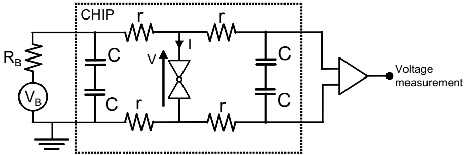
Figure 29: Experimental setup for the current bias mode.
