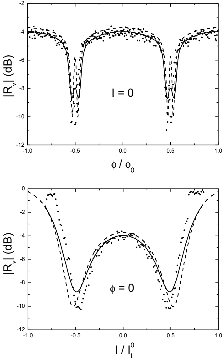
Figure 18: Modulus of the reflection coefficient for a contact with mesoscopic pin code \tau = \{0.983\} . The fridge temperature was 26 mK. Lower graph: modulus as a function of the dc bias current I at \phi = 0 . Upper graph: modulus as a function of the external magnetic flux \phi threading the loop at I = 0 . Dots: experimental results. Dashed lines: zero temperature prediction of the linear approximation presented in section 3.2. Solid lines: zero temperature prediction of the numerical simulation of the phase dynamics.
