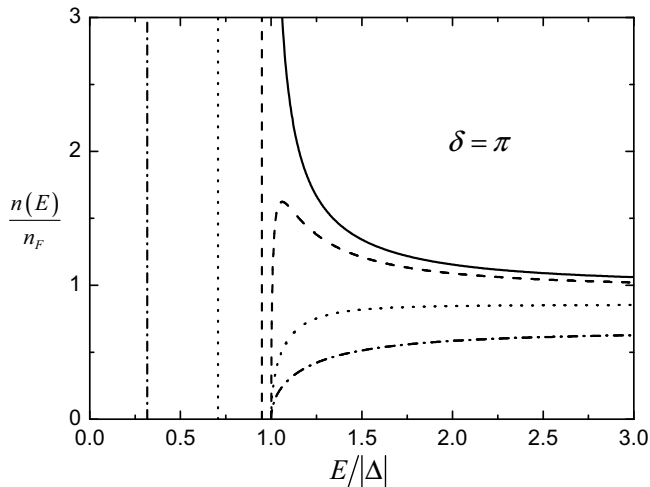
Figure 6: Local density of states at the constriction for four different values of the transmission: \tau=0 (solid line), \tau=0.1 (dashed line), \tau=0.5 (dotted line), \tau=0.9 (dashed-dotted line). The case \tau=0 corresponds to having two uncoupled superconductors and one therefore recovers the previously calculated BCS density of states. The vertical lines corresponds to the Andreev levels of energy E_{\pm} . The curves have been sketched for a phase difference \delta=\pi across the weak link. For clarity only the energy range E > 0 is represented. The local density of states for E < 0 is obtained by symmetry with respect to the E=0 vertical line.
