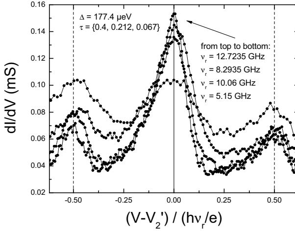
Figure 38: Differential conductance of an atomic contact around V_2' = 0.98 \times 2\Delta / (2e) at different microwave frequencies. The distance of the first satellite to the center peak scales linearly with the radiation frequency \nu_r . The normalization factor h\nu_r/e of the horizontal axis is different for each one of the four curves.
