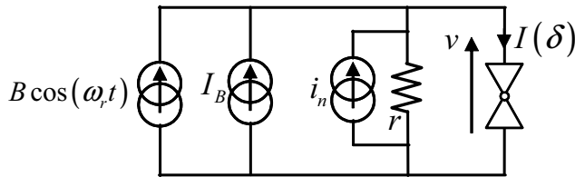
Figure 11: Atomic contact embedded in a dissipative environment. This representation is the Norton equivalent of the circuit of Figure 9 with B = A/r , I_B = V_B/r and i_n = e_n/r .
