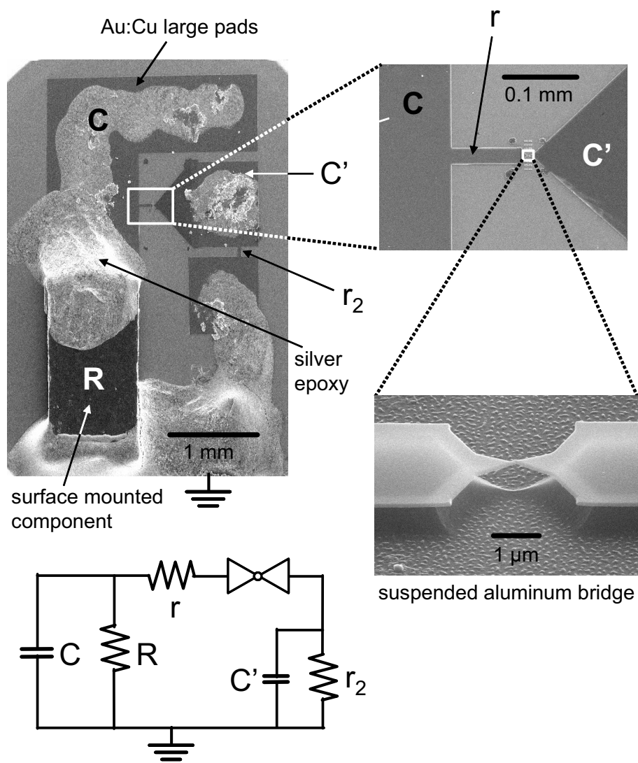
discrete elements equivalent circuit
