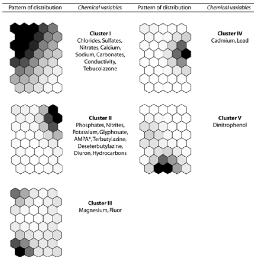
Fig. 5 : Gradient analysis of the distribution pattern of each chemical variable on the trained SOM, with visualization in shading scale (dark = high values, light = low values). The mean value of each variable was calculated in each output neuron of the above trained SOM. Each variable map is to compare to the trained map in Fig. 4.
