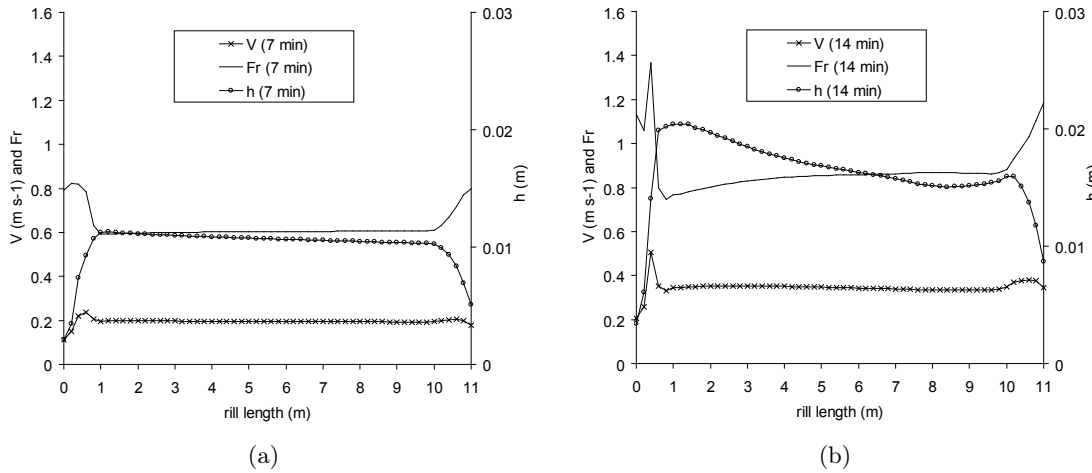
FIG. 4.9: Calculated longitudinal velocity, Froude number, and water depth along the rill length for the Bonifay ( D_s = 200\ \mu m and \rho_s = 2650\ kg\ m^{-3} ) and the formula of Low, at respectively 7 min and 14 min after the beginning of the simulation
