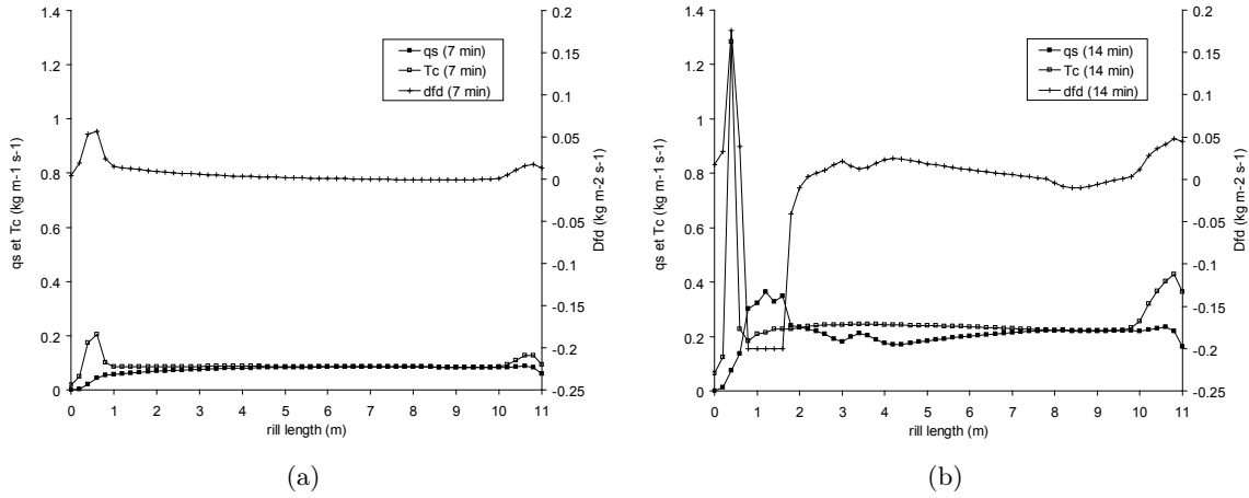
FIG. 4.8: Calculated sediment load ( q_s ), sediment transport capacity ( T_c ) and detachment or deposition rate ( D_{fd} ) along the rill length for the Bonifay ( D_s = 200\ \mu m and \rho_s = 2650\ kg\ m^{-3} ) and the formula of Low, at respectively 7 min and 14 min after the beginning of the simulation
