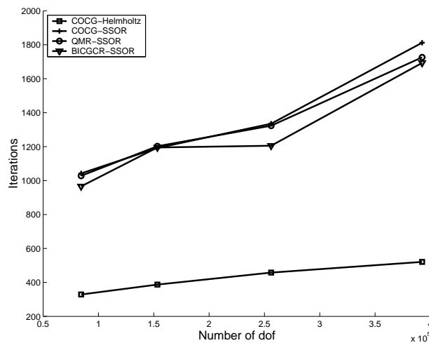
Figure B.3: Number of iterations against the number of dof.
