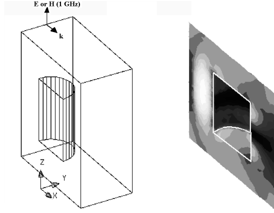
Figure B.8: An incident plane wave on a 3D PEC cylinder, \mathbf{H} -formulation.
