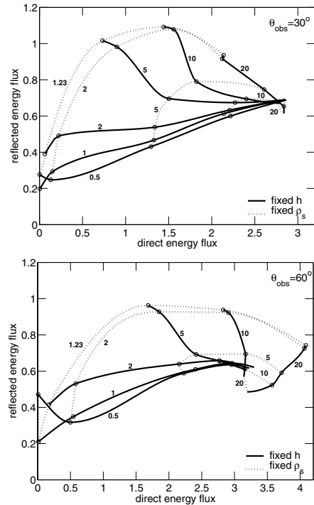
Fig. 16. The total reflected energy flux as a function of the total direct energy flux, both are in the energy range 1–30 keV, for an observation inclination 30^\circ (top panel) and 60^\circ (bottom panel) with different source height and radius. The thin lines represent the fixed source radius and the thick lines indicate the same source height. These lines are interpolated from the results calculated from the model GR as shown at the intersection points.
