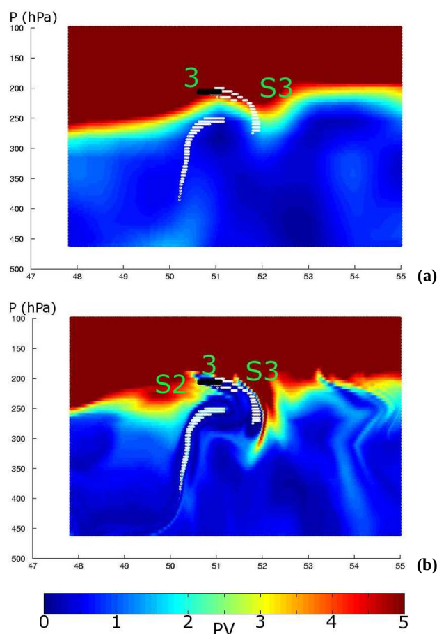
Fig. 13. Potential Vorticity (p.u., colorbar) in a vertical cross section intercepting air parcels of groups S2, 3 and S3 (see location on Fig. 9): (a) with spatial and temporal interpolation of ECMWF fields, (b) with the RDF technique (integration time 18 h). Abscissa is latitude in degrees. The black points stand for air parcels of group 3. White shaded regions show air parcels that come from the lower troposphere (pressure larger than 800 hPa) 30 h ago.
