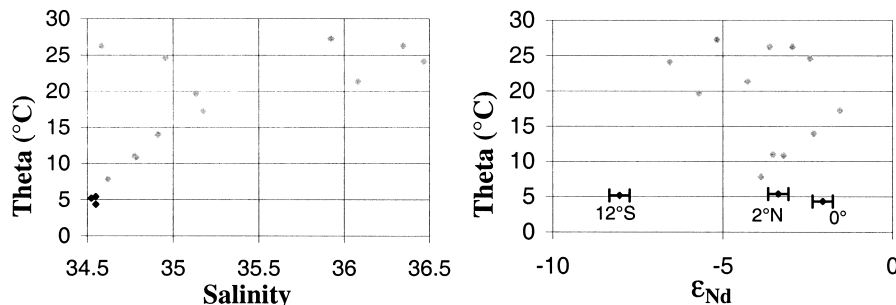
Fig. 3. \theta -S and \theta - \epsilon_{Nd} diagrams of the analyzed samples. Black symbols represent AAIW samples. On the \theta -S diagram AAIW show very similar characteristics, whereas they are clearly distinguishable on the \theta - \epsilon_{Nd} diagram.
