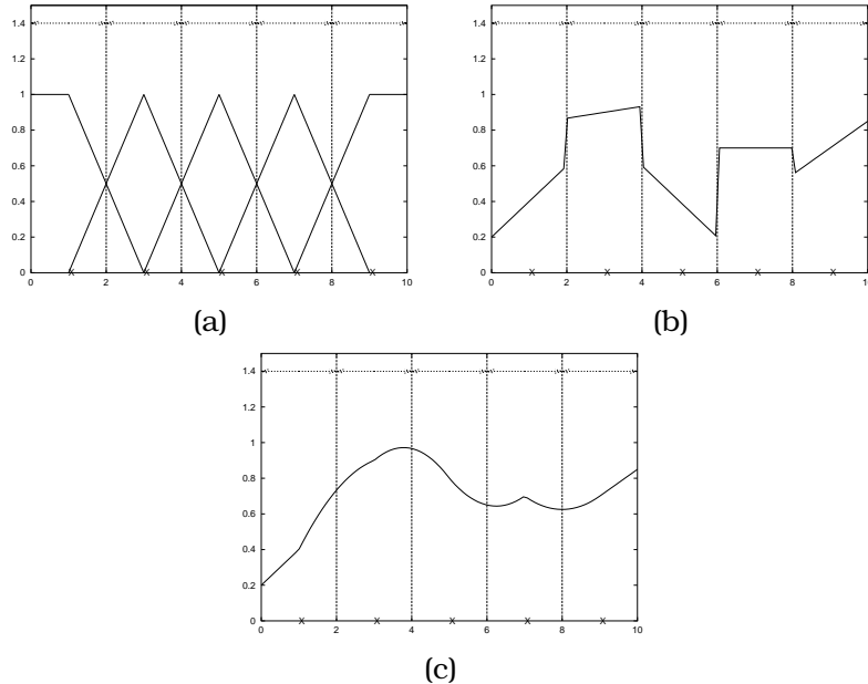
Figure 3.20: An example of the effect of the add mutation operator when applied to the first individual defined in figure 3.14.
