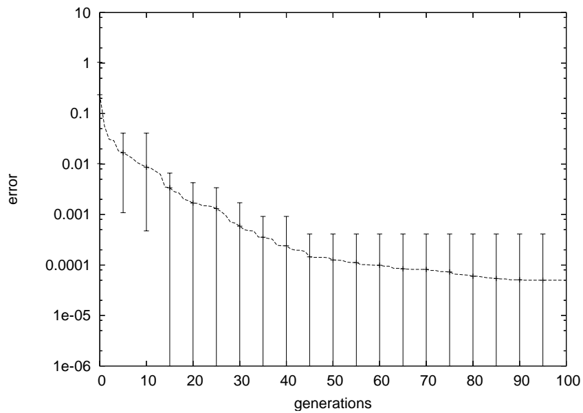
Figure 4.9: Last section of the best fitness plotted with error bars (in logarithmic scale) against the number of generations, averaged in 10 runs of the experiment with a priori knowledge.
