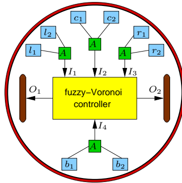
Figure 4.19: Diagram that represents the conceptual integration of the Fuzzy Voronoi controller in a Khepera robot. The inputs I_1 , I_2 , I_3 e I_4 correspond respectively to the average of pairs of input sensors. The outputs O_1 y O_2 provide directly the control signals to be applied to the motors.
