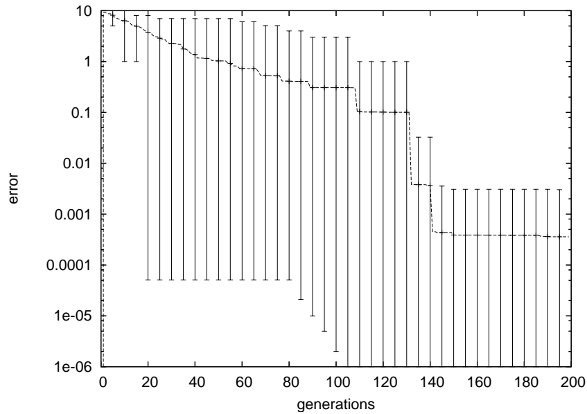
Figure 4.15: Last section of the best fitness plotted with error bars (in logarithmic scale) against the number of generations in 10 runs of the experiment with a priori knowledge.
