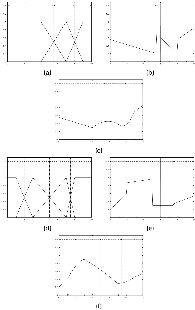
Figure 3.18: The first and the second child of the Voronoi crossover between the individuals defined in figure 3.14. The graphic (a) shows the Voronoi regions and the base functions, (b) the local approximators and (c) the complete approximation of the first child. The graphs (d), (e) and (f) correspond to the second child. The hyperplane is represented with the wider line at x = 6 .
