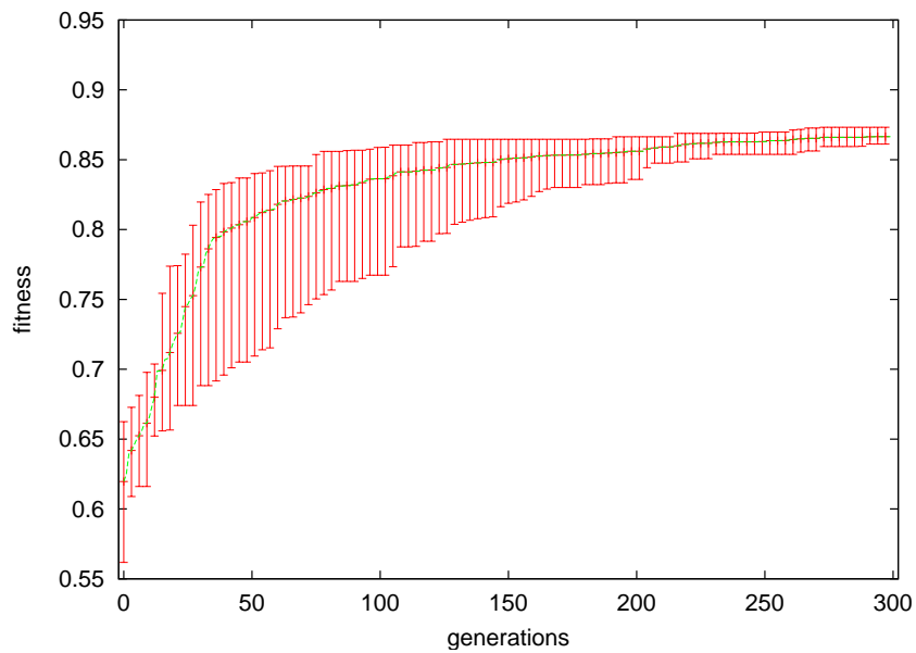
Figure 4.21: Best fitness plotted against the number of generations, averaged over 5 runs, together with error bars.
