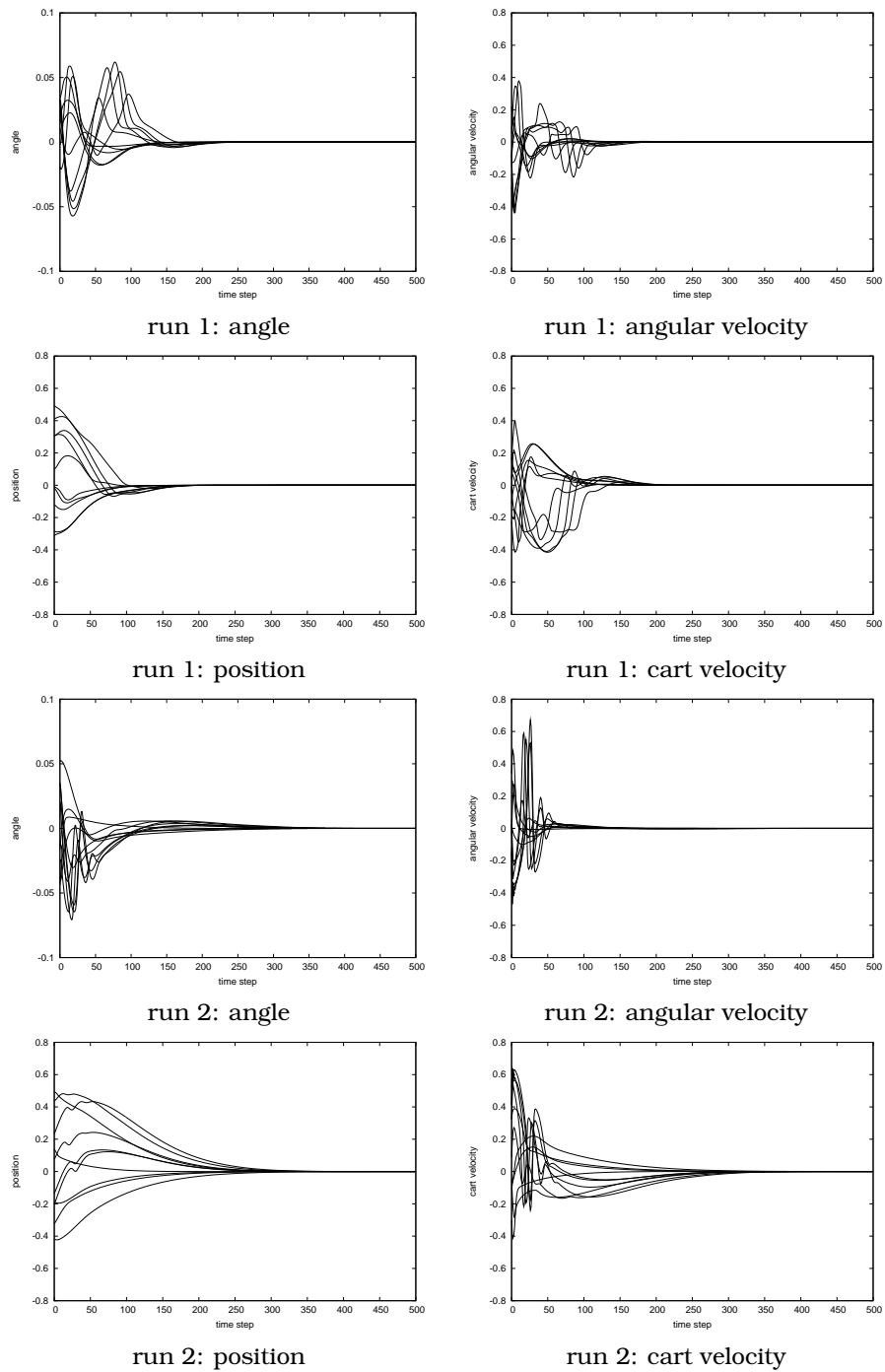
Figure 4.16: Evaluation of the cart-pole system ( \mathbb{R}^4 ) in 10 random experiments with the best controller obtained in 2 different runs of the evolutionary algorithm without a priori knowledge.
