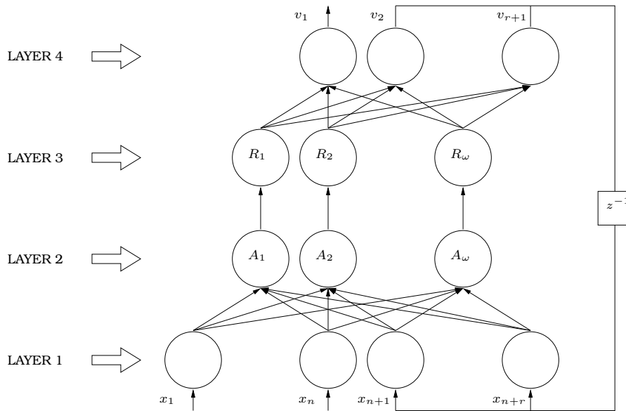
Figure 5.1: The structure of the recurrent Voronoi-based fuzzy system
