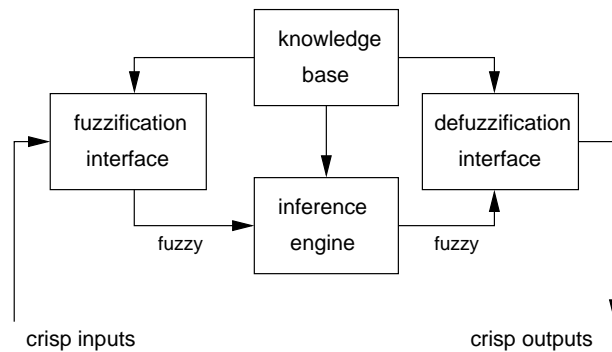
Figure 2.5: The main components of a fuzzy system.
