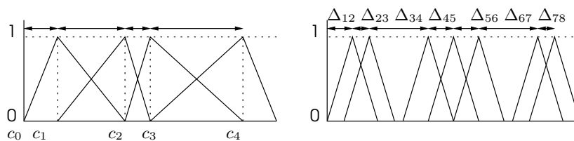
Figure 2.14: The partition of input (left) and output (right) fuzzy variables in the model proposed by Hoffmann. Only the centers c_i of the input fuzzy membership functions and the distance \Delta_{ij} between adjacent output fuzzy membership functions need to be encoded.
