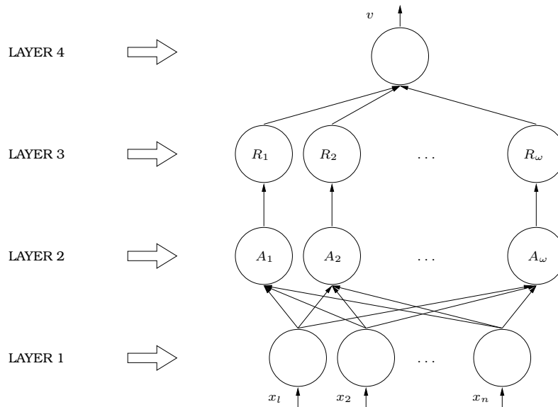
Figure 4.1: The structure of the Voronoi-based fuzzy system
