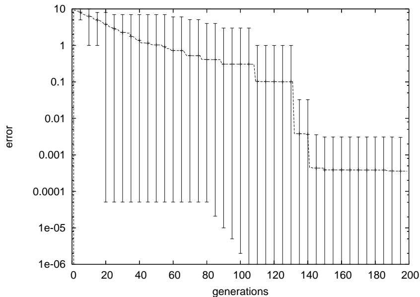
Figure 4.14: Last section of the best fitness plotted with error bars (in logarithmic scale) against the number of generations in 10 runs of the experiment without a priori knowledge.
