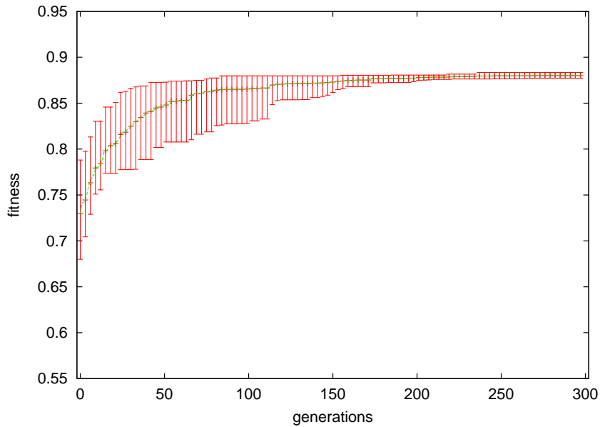
Figure 4.26: Best fitness plotted against the number of generations, averaged over 5 runs, together with error bars.
