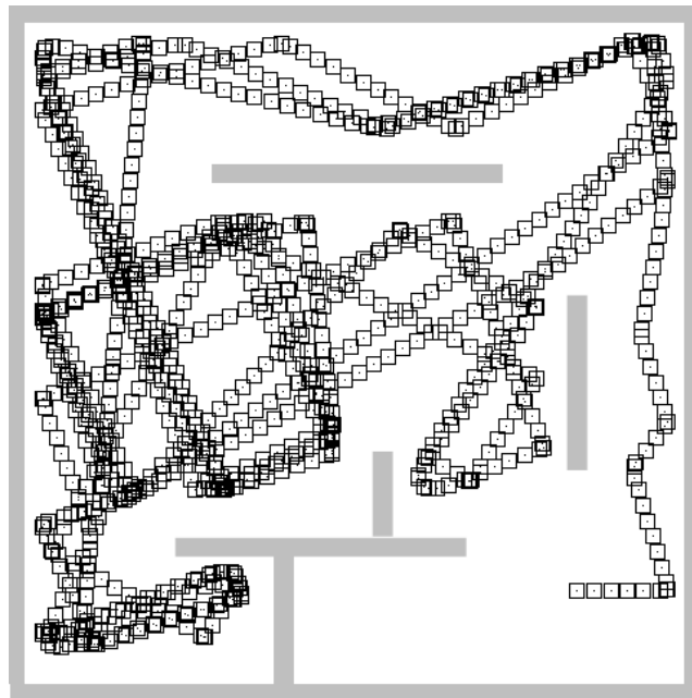
Figure 4.22: Performance of the best controller obtained after evolution without a priori knowledge.
