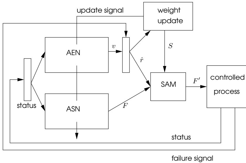
Figure 2.13: The architecture of the GARIC model.
