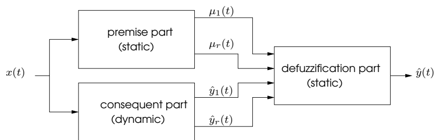
Figure 2.18: The general representation of the DFNN model.
