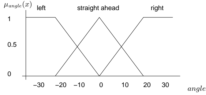
Figure 2.4: An example of a linguistic variable defined with three linguistic terms. The linguistic variable angle , which corresponds to the system variable robot's target angle , is defined with three linguistic terms: left , straight ahead and right . These linguistic terms define three concepts through three fuzzy sets.
