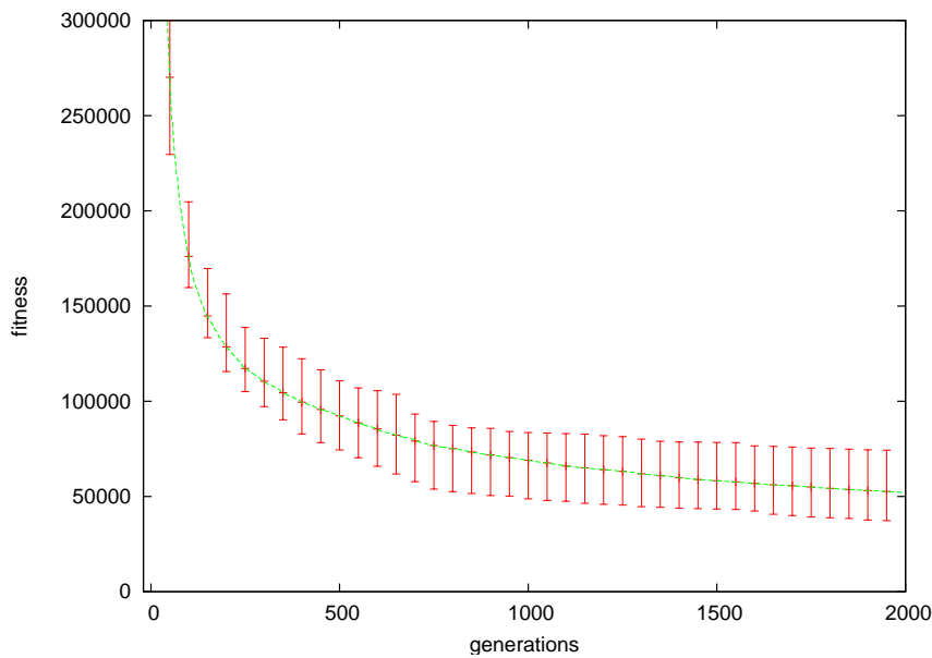
Figure 3.22: Best fitness in 120 runs of the experiment plotted with error-bars against the number of generations with different values of crossover and mutation probabilities.
