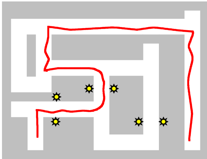
Figure 5.12: Performance of the best controller evolved with a priori knowledge when applied to the control of a robot in a scenario not used during evolution.
