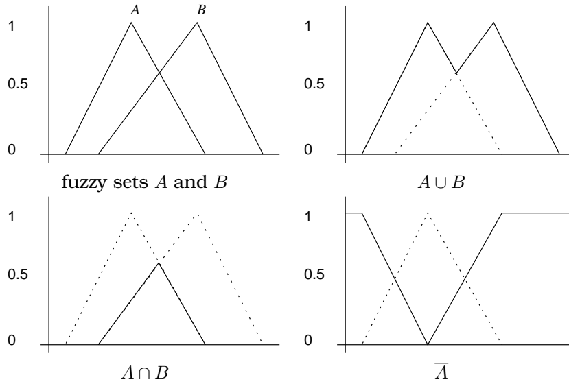
Figure 2.3: Example of the basic operations on fuzzy sets.
