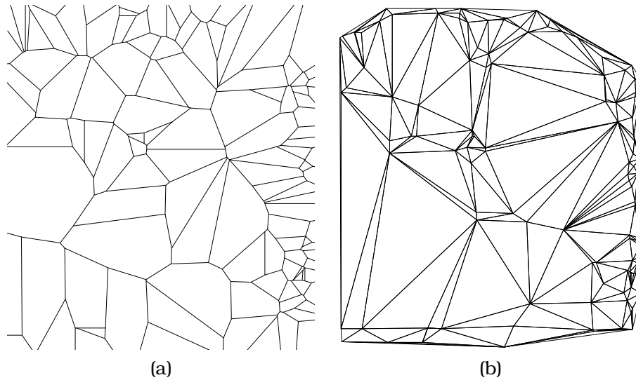
Figure 3.29: The (a) Voronoi partition and the (b) Delaunay triangulation defined by the best approximator obtained with the Voronoi approximation method.
