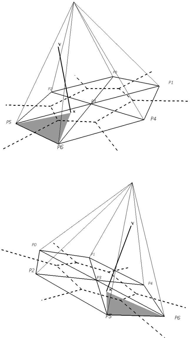
Figure 3.7: An example of the computation of a 2-dimensions Voronoi shape function presented in two different views. The dotted lines represent the Voronoi diagram defined for the points P_0, \dots, P_6 . The continuous lines in the same plane define the Delaunay triangulation. The shape function \phi_3(x) is represented graphically by the altitude of the pyramid. The colored triangle shows the computation of the value V = \phi_3(x) for a given x , represented as the relative area of the shadowed triangle.
