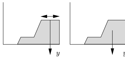
Figure 2.7: An example of the output produced by the mean of maximum (left) and the center of gravity (right) methods when applied to the fuzzy set obtained as the output of the inference process in the example of figure 2.6.
