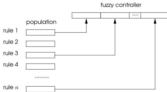
Figure 2.15: The SEFC model. A fuzzy system is built for evaluation by randomly selecting a set of rules from the population.
