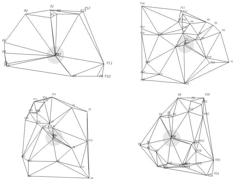
Figure 4.13: Delaunay triangulations of four approximations performed with wrong a priori knowledge. The dark circle is centered at the Voronoi site defined by the wrong rule
