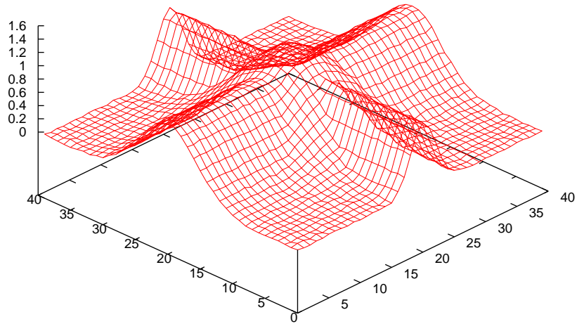
Figure 3.30: Target function for the second experiment.
