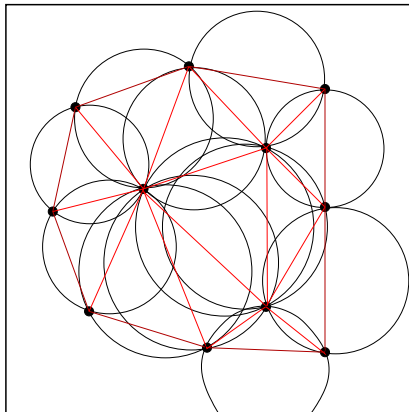
Figure 3.4: The circumcircles defined by the Delaunay triangulation exemplified in figure 3.3. Note that the circumcircles defined by each three groups of points do not include other points, except the three points that define them
