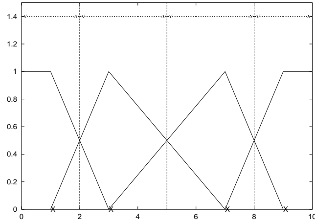
Figure 3.6: An example of the triangular shape functions defined for a set of N = 4 points in \mathbb{R} . The points are indicated with a cross over the x -axis, the vertical lines define the boundaries of the Voronoi regions and the top arrows indicate the span of each one.
