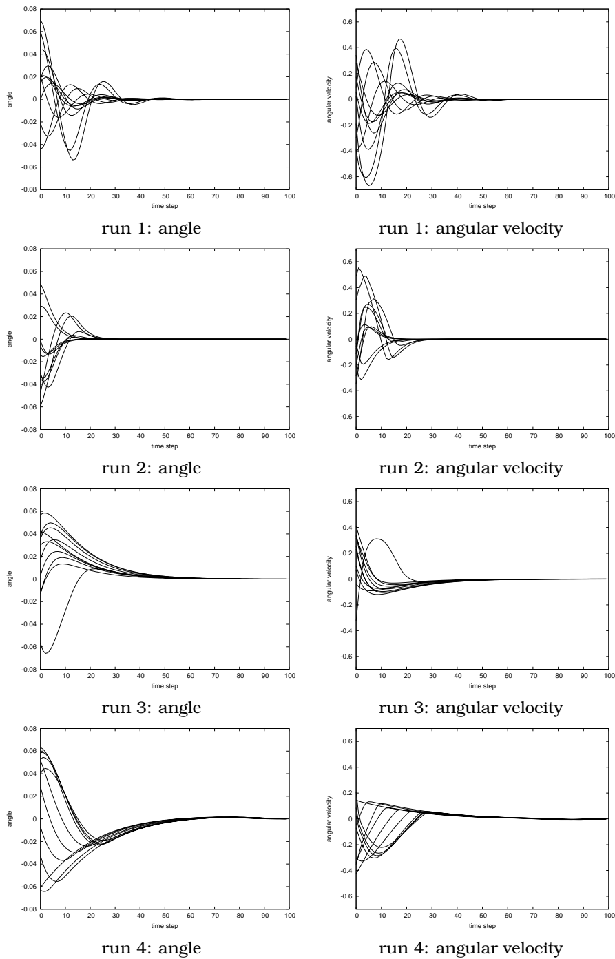
Figure 4.10: Evaluation of the cart-pole system ( \mathbb{R}^2 ) in 10 random experiments with the best controller obtained in 4 different runs of the evolutionary algorithm without a priori knowledge.
