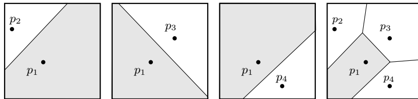
Figure 3.2: An example of a Voronoi cell defined in terms of half plane intersections for a set of 4 sites P = \{p_1, p_2, p_3, p_4\} . The first three diagrams correspond to the half planes h(p_1, p_2), h(p_1, p_3) and h(p_1, p_4) that contain p_1 respectively. The fourth diagram shows the full Voronoi diagram, including the cell V(p_1) defined as half planes intersections.
