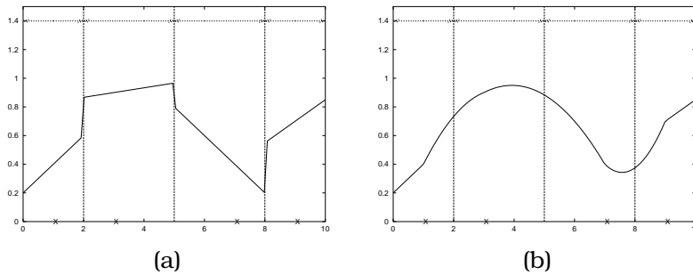
Figure 3.9: The approximation defined by the local approximators in each Voronoi region (plot a) and the complete Voronoi approximation (plot b) for the example in \mathbb{R}(d = 1) .
