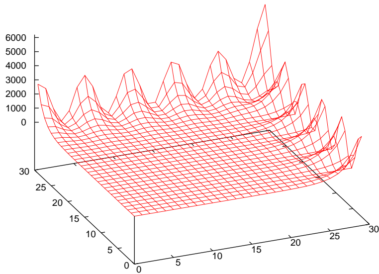
Figure 3.27: Target function for the first experiment.
