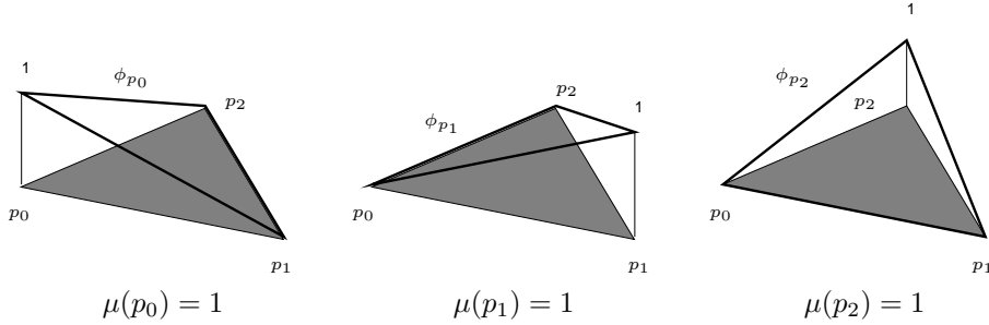
Figure 4.3: The three shape functions defined over a Delaunay triangle in \mathbb{R}^2 .
