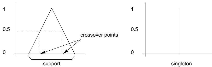
Figure 2.2: Example of the support, the crossover point and the singleton concepts
