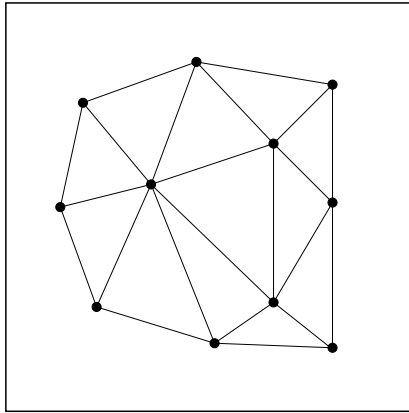
Figure 3.3: An example of a Delaunay triangulation. The set of points that defines the triangulation is the same set P used in figure 3.1.
