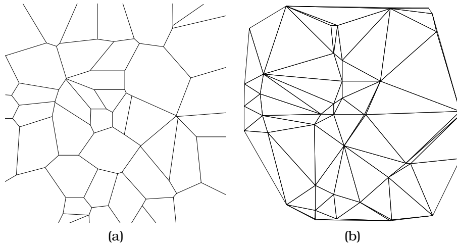
Figure 3.32: The (a) Voronoi partition and the (b) Delaunay triangulation defined by the best approximator obtained with the Voronoi approximation method.
