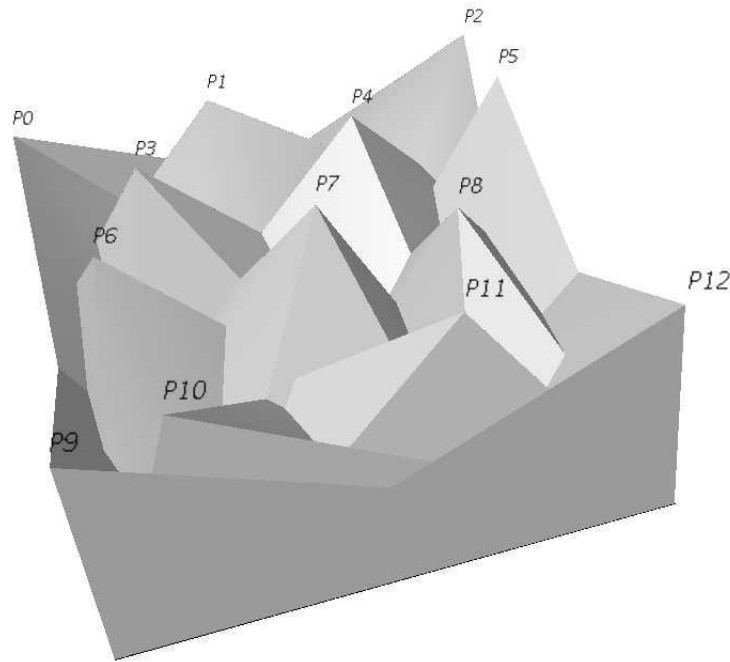
Figure 4.2: The membership functions defined by the same set of point used in the example of section 3.2.1.
