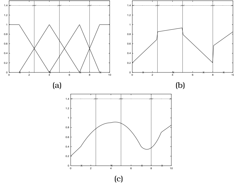
Figure 3.19: An example of the effect of the perturbation mutation operator when applied to the first individual defined in figure 3.14.
