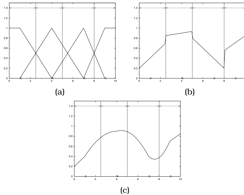
Figure 3.19: An example of the effect of the perturbation mutation operator when applied to the first individual defined in figure 3.14.
