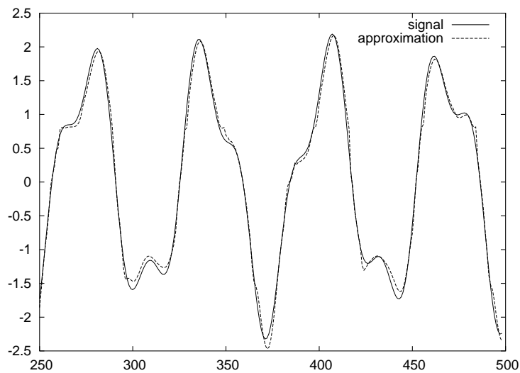
Figure 5.4: The best approximation in the system identification problem (dotted line) and the corresponding test signal (continuous line).
