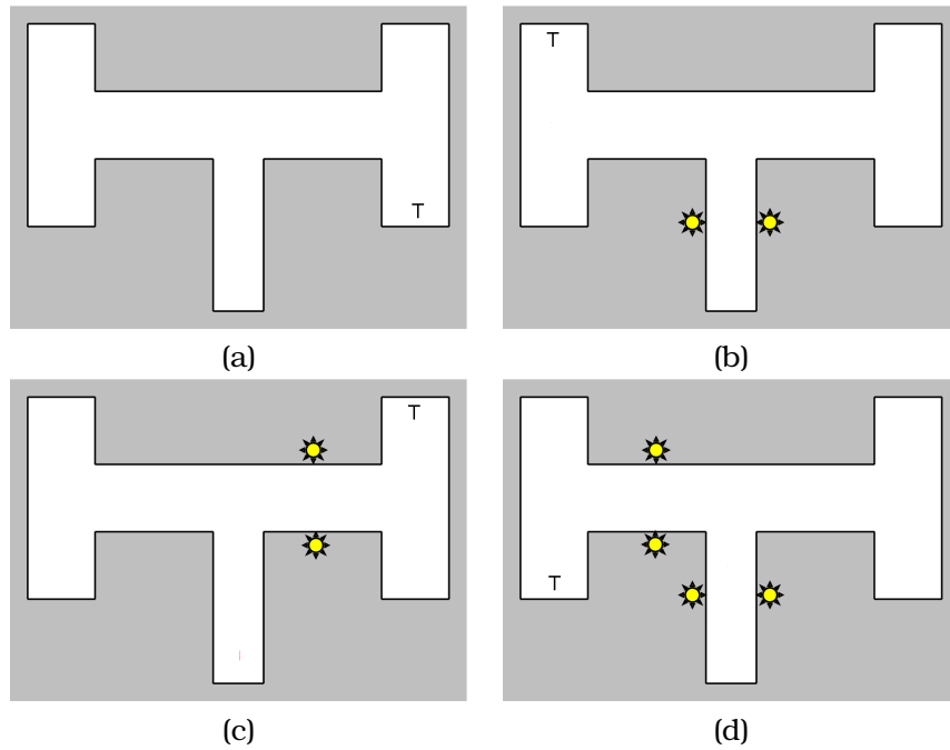
Figure 5.5: The four scenarios used to evaluate the performance of the controllers, where the target position is indicated by a T and the light sources with stars. In scenario (a) the robot has to run right in both intersections, in (b) the robot has to turn left first and then right, in (c) the robot has to turn right and then left and in (d) to the left in both intersections.
