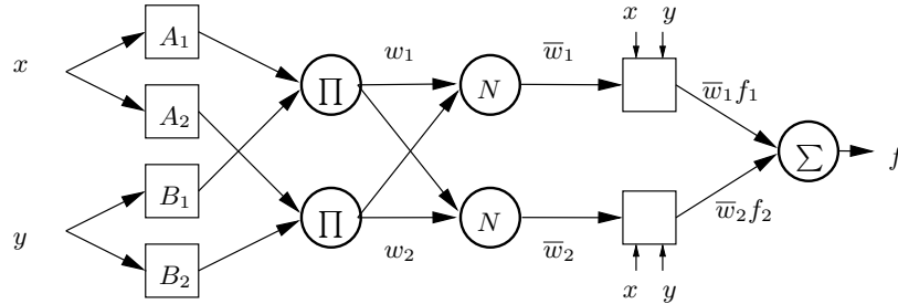
Figure 2.12: An ANFIS network defined with two inputs ( x and y ), one output ( f ) with two linguistic terms defined for each input variable ( A_1, A_2 and B_1, B_2 respectively) and two fuzzy rules.
