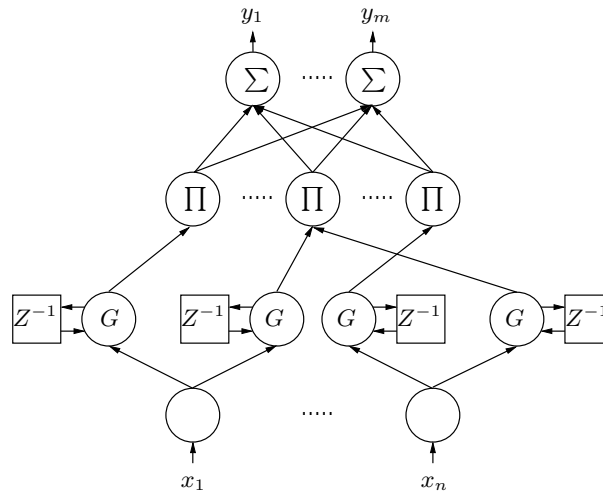
Figure 2.16: The structure of the RFNN model.
