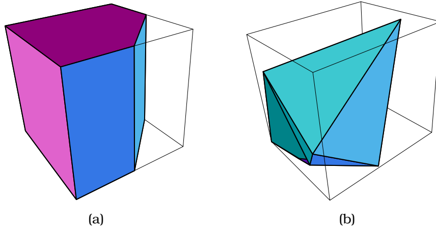
Figure 4.27: The (a) original area of application of the first a priori rule and the (b) modified area of application of the same rule at the end of the evolution. The graphics corresponds to projections of the four dimension areas of applications into the three dimension space by dropping the last coordinate.
