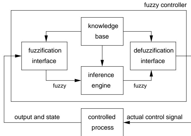
Figure 2.11: The execution model of a fuzzy controller.
