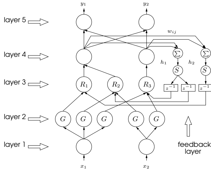
Figure 2.17: The structure of the RSONFIN model.
