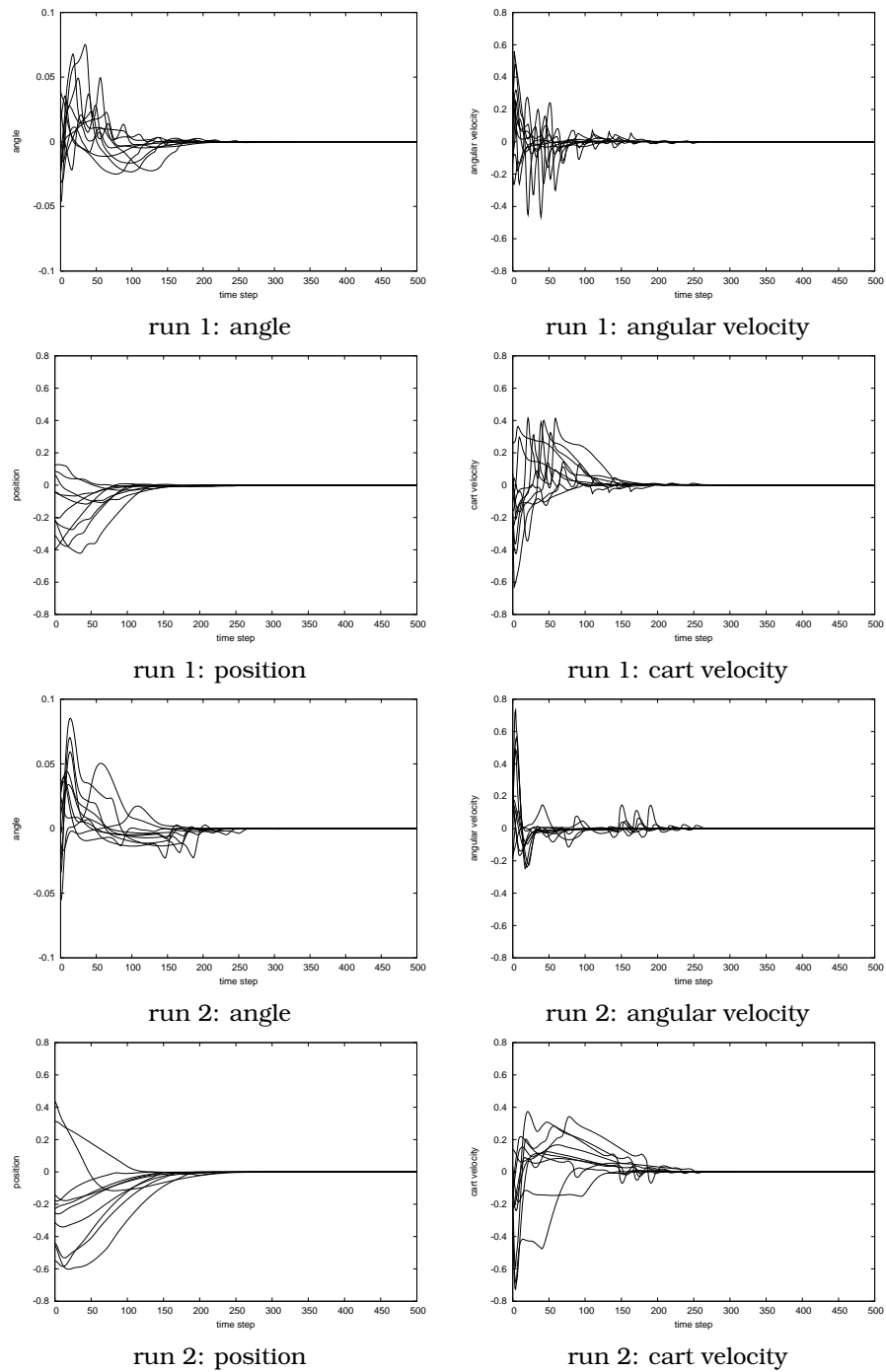
Figure 4.17: Evaluation of the cart-pole system ( \mathbb{R}^4 ) in 10 random experiments with the best controller obtained in 2 different runs of the evolutionary algorithm with a priori knowledge.
