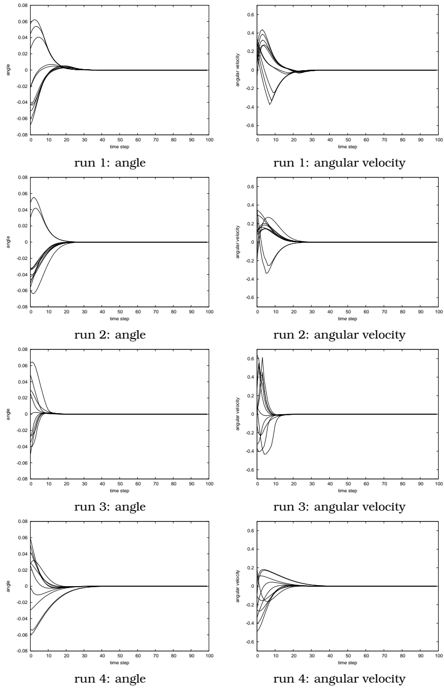
Figure 4.11: Evaluation of the cart-pole system ( \mathbb{R}^2 ) in 10 random experiments with the best controller obtained in 4 different runs of the evolutionary algorithm with a priori knowledge.
