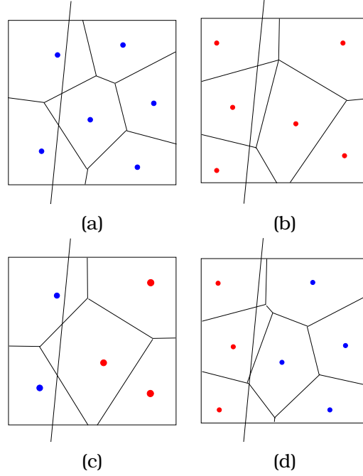
Figure 3.16: An example the effect of the Voronoi crossover in \mathbb{R}^2 . The graphs (a) and (b) show the Voronoi diagrams defined by the parents and the graphs (c) and (d) the Voronoi diagrams defined by the children.
