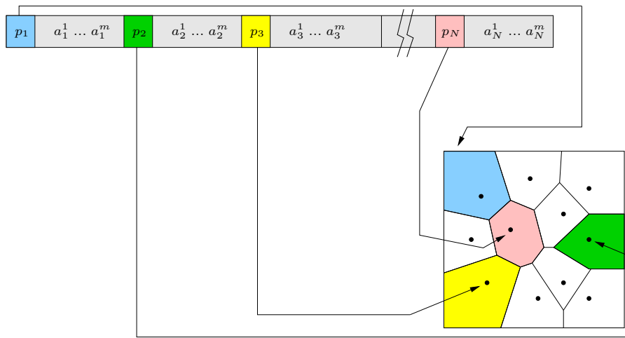
Figure 4.4: An example of the representation for a Voronoi-based fuzzy system individual defined in \mathbb{R}^2 with m outputs.
