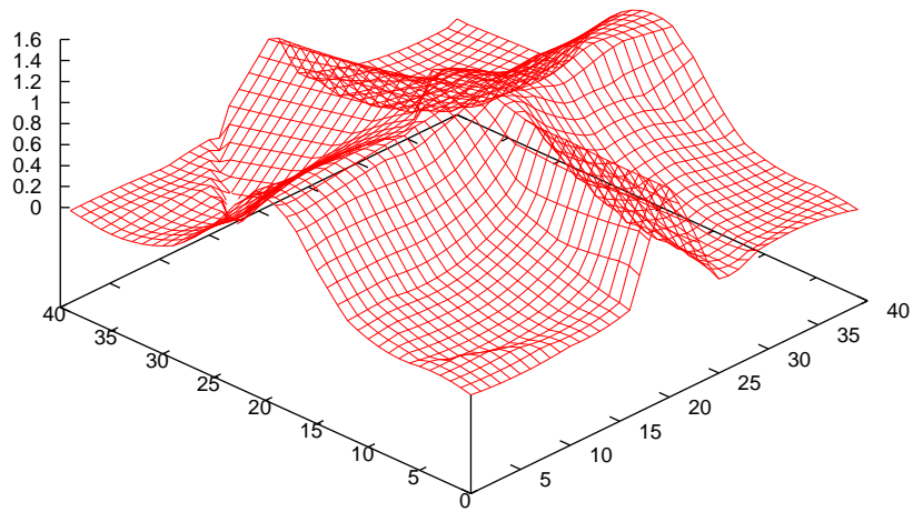
Figure 3.31: Best approximation obtained with the Voronoi approximation method.
