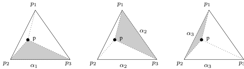
Figure 3.5: An example of the computation of the barycentric coordinates for a given point p in a triangle defined by the points p_1 , p_2 and p_3 . The relative area of the gray triangle corresponds to the value of the barycentric coordinate.
