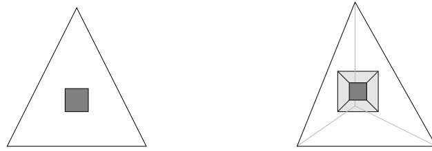
Figure 3.8: An example of the external hypertriangles used to avoid open Voronoi regions in 2D (left) and 3D (right). The dark gray area identifies the input space
