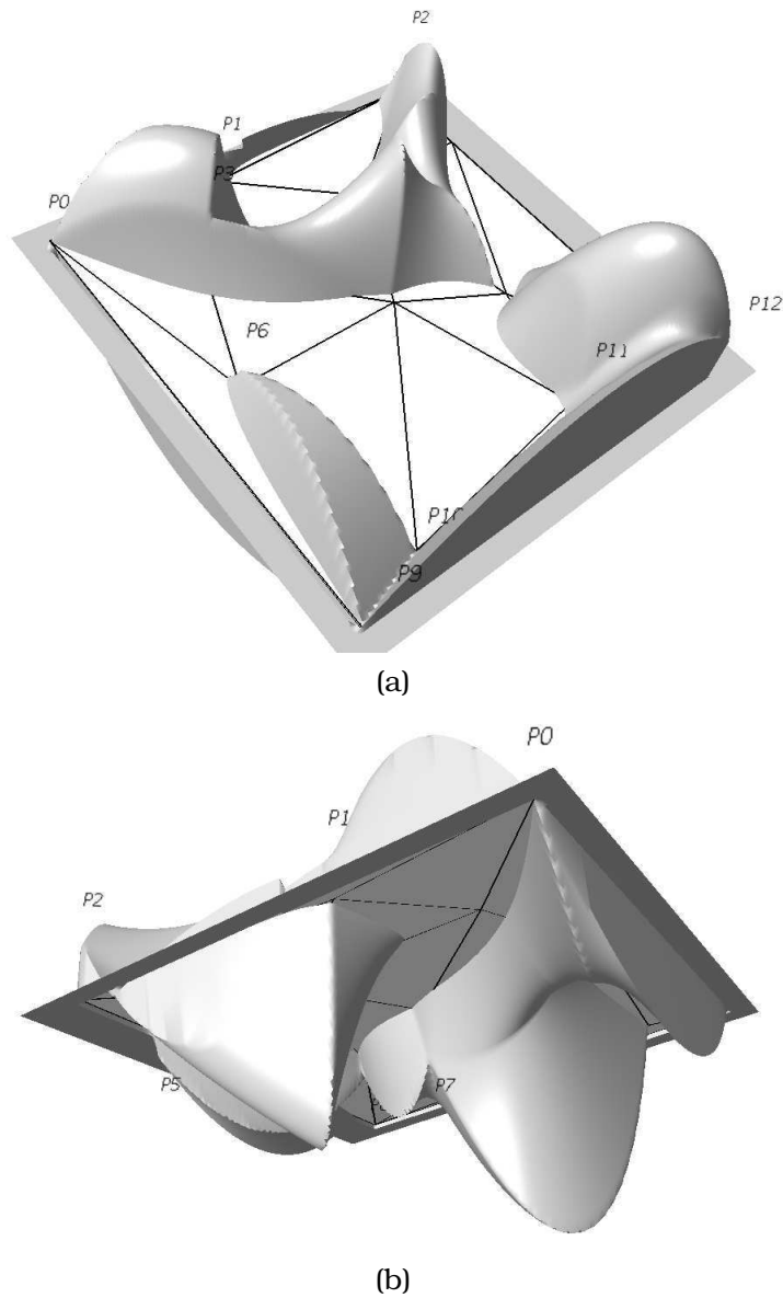
Figure 3.12: The complete Voronoi approximation in a view (a) from the top and (b) from the bottom. When comparing with the plots of figure 3.11 consider that a different view angle has been selected in order to improve visualization.
