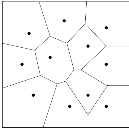
Figure 3.1: An example of a Voronoi diagram for a set of points P in \mathbb{R}^2 .
