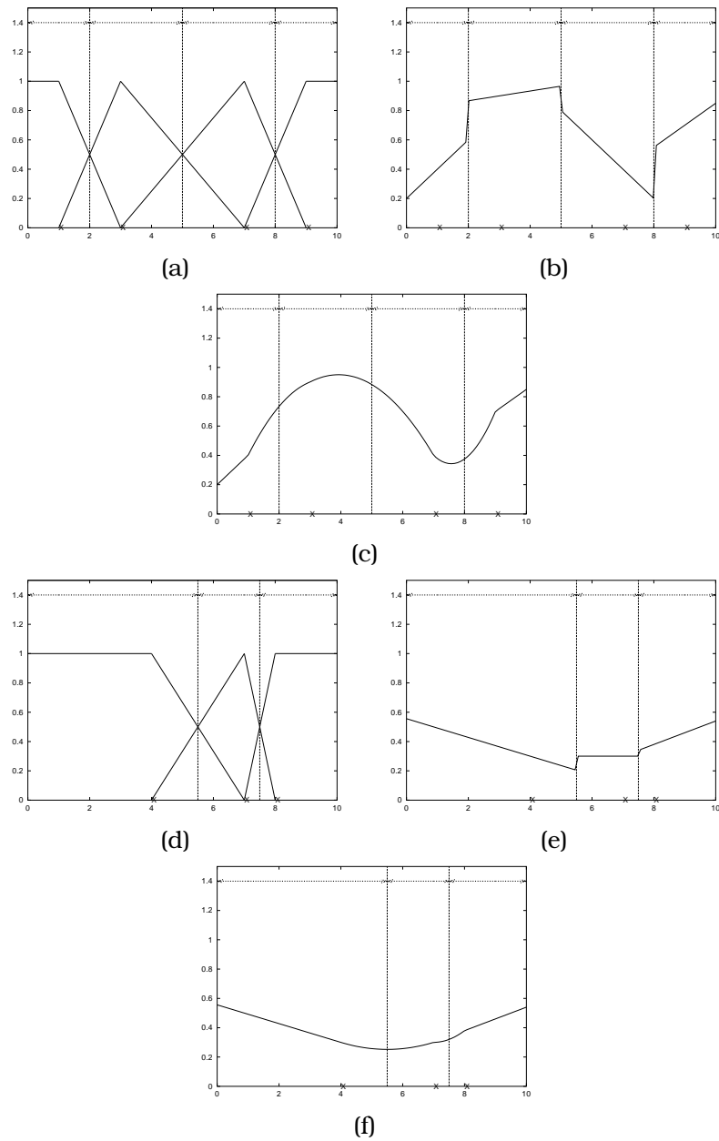
Figure 3.15: A graphical representation of the individuals defined in figure 3.14. The graph (a) shows the Voronoi regions and the shape functions, (b) the corresponding local linear approximators and (c) the complete approximation for the first individual. The graphs (d), (e) and (f) correspond to the second individual.
