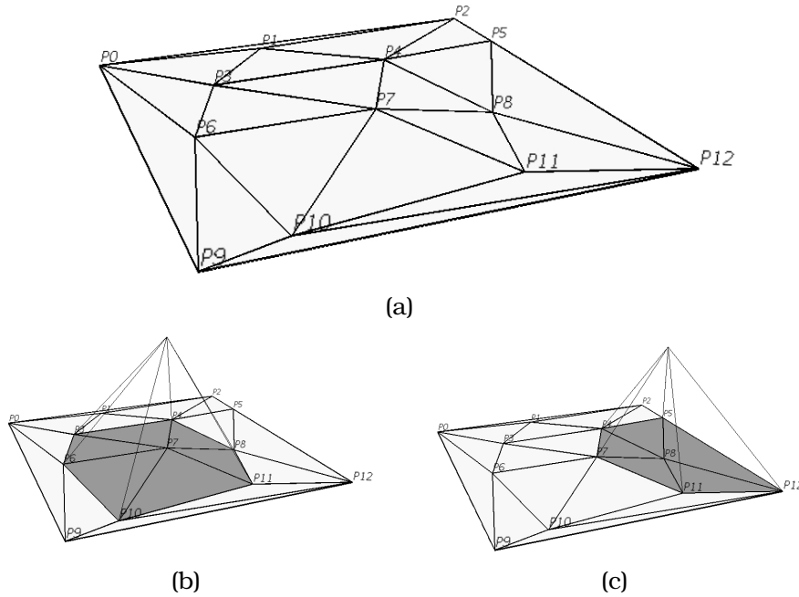
Figure 3.10: Graphic plots of (a) the Delaunay triangulation defined by the points, (b) the shape function defined by p_7 and (c) the shape function defined by p_8 .
