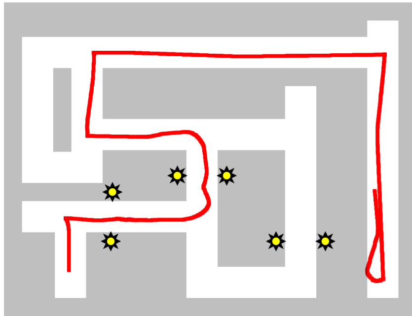
Figure 5.11: Performance of the best controller evolved without a priori knowledge when applied to the control of a robot in a scenario not used during evolution.
