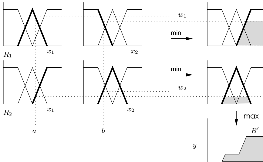
Figure 2.6: The max-min inference method as usually applied in Mamdani fuzzy systems. The figure shows a fuzzy system with two input variables and one output variable, all of them defined with three linguistic terms. The rule base contains two rules R_1 and R_2 , which involve in their definition the antecedent linguistic terms defined with a wide continuous line. The dotted lines show the membership values for the input values a and b . The minimum values are denoted by w_1 and w_2 . The computed fuzzy set B' is shown in gray color.
