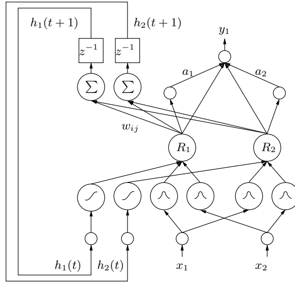
Figure 2.19: The general representation of the TRFN model.
