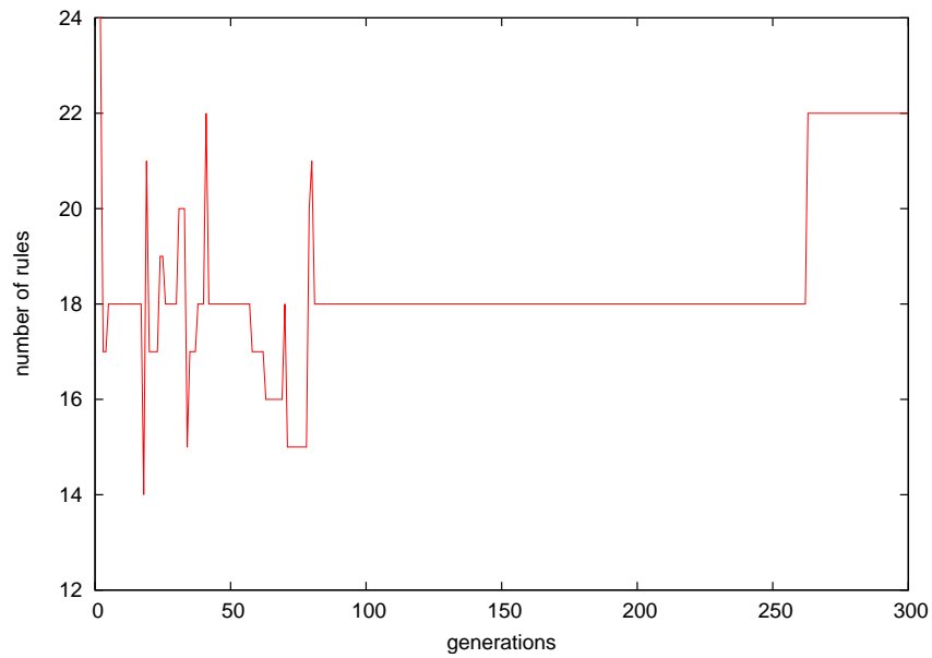
Figure 4.24: Number of rules of the best individual in each generation of the evolutionary process.
