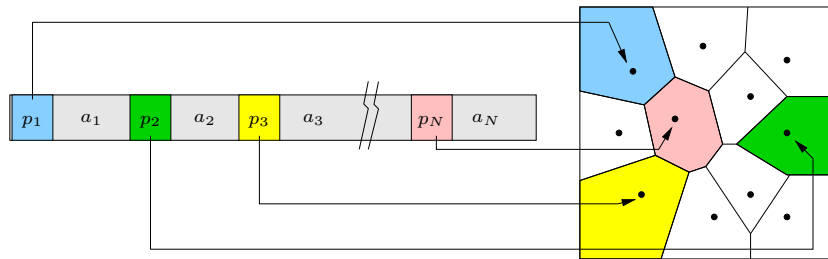
Figure 3.13: An example of the representation for an individual defined in \mathbb{R}^2 .
