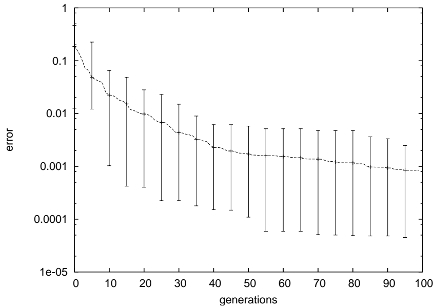
Figure 4.8: Last section of the best fitness plotted with error bars (in logarithmic scale) against the number of generations, averaged in 10 runs of the experiment without a priori knowledge.
