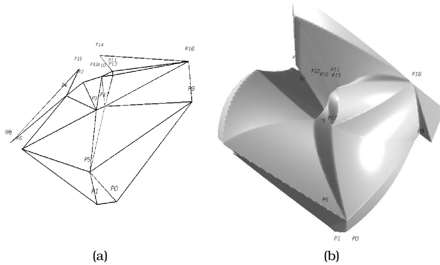
Figure 4.12: Example of the control function defined by a Voronoi-based fuzzy controller obtained by evolution. The plot on the left (a) shows the Delaunay triangulation and the plot on the right (b) the corresponding approximation. The value defined by the a priori rule is located in the center of the plots.
