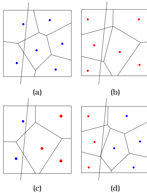
Figure 3.16: An example the effect of the Voronoi crossover in \mathbb{R}^2 . The graphs (a) and (b) show the Voronoi diagrams defined by the parents and the graphs (c) and (d) the Voronoi diagrams defined by the children.
