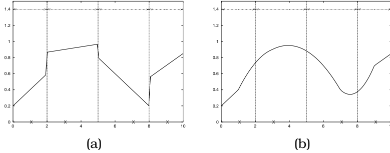
Figure 3.9: The approximation defined by the local approximators in each Voronoi region (plot a) and the complete Voronoi approximation (plot b) for the example in \mathbb{R}(d = 1) .
