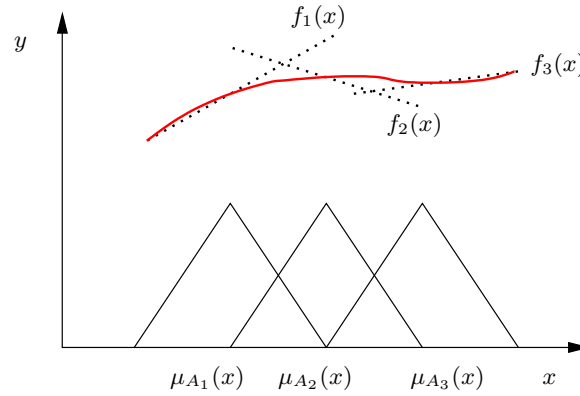
Figure 2.8: The inference method as usually applied in Takagi-Sugeno fuzzy systems. The figure shows a fuzzy system with one input variable x and one output variable y . The rule base contains three rules R_1 , R_2 and R_3 which involve in their definition the linguistic terms A_1 , A_2 and A_3 and the linear functions f_1 , f_2 and f_3 respectively. The output of the fuzzy system corresponds to the value defined by the linear combination of the consequent functions, weighted by their firing strength.
