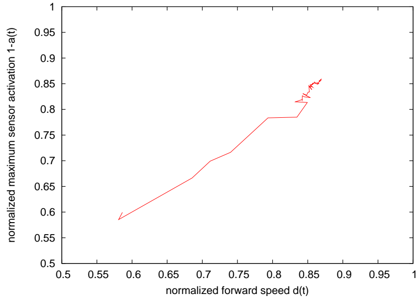
Figure 4.23: Relation between the terms d(t) and (1 - a(t)) for the best individual along the generations of the evolutionary process.
