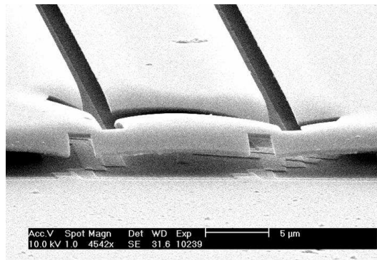
Fig. 8.2. Scanning electron microscope image at 45^\circ of a sample coated by a bilayer LOR30B/PMMA covered with metal, after development, metal deposit and before lift-off. One clearly sees the wide undercut in the LOR30B resist, creating wide hanging PMMA structure, and allowing metallic evaporation at large angles.
