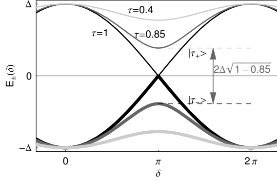
Fig. 5.2. Energy spectrum of the Andreev bound states for three values of the transmission \tau of the single channel of the conductor. The minimum gap between Andreev bound states is obtained at \delta = \pi and is given by 2\Delta\sqrt{1-\tau} .
