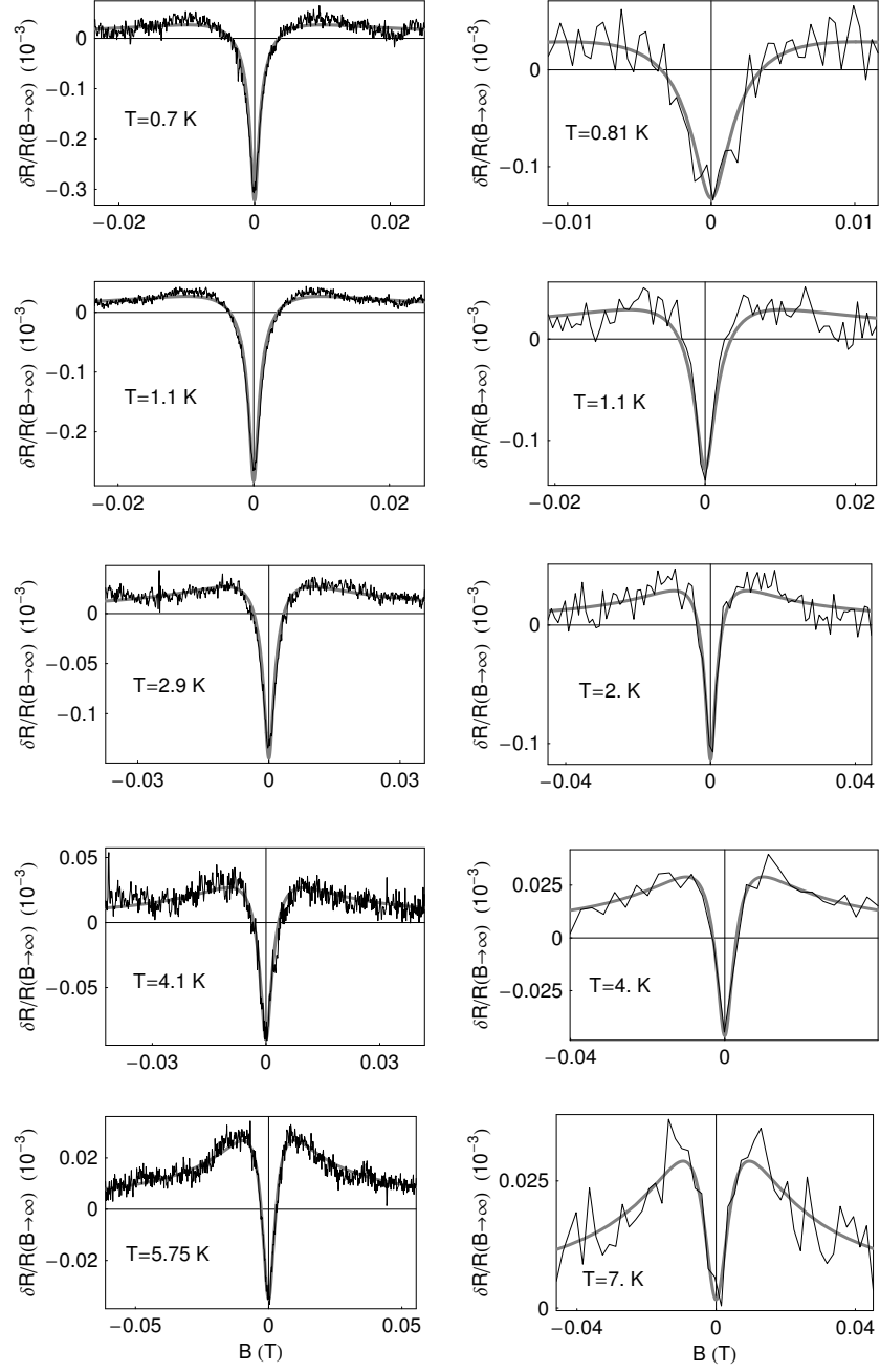
Fig. 2.8. Magnetoresistance (thin lines) of the bare wire (left column) and implanted wire (right column) for 0.5 \text{ K} < T < 7 \text{ K} . Thick grayed lines are plotted using theory of weak localization Eq. (2.17) with \tau_{\text{so}} = 10 \text{ ps} and using \tau_{\varphi} as a fit parameter.
