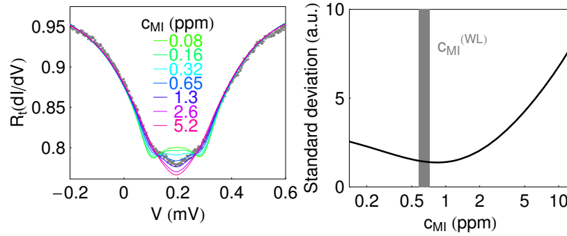
Fig. 3.28. Left panel-dots: differential conductance dI/dV(V) of the tunnel junction for the implanted wire for U = 0.2 mV and B = 0.9 T. Left panel-lines: calculations using various values of c_{\text{MI}} and for \kappa_{ee} = 0.05 \text{ ns}^{-1} \text{ meV}^{-1/2} . Right panel: sum of all the standard deviations to the experimental curves corresponding to the implanted wire (gray dots of the right panels of Fig. 3.29) as a function of the used concentration c_{\text{MI}} . The result from weak localization experiments Table 2.3 is shown as a gray band.
