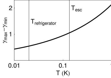
Fig. 5.22. Resolution of the measurement of the current phase relation in the switching experiment as a function of temperature. The base refrigerator temperature is T_0 = 20 \text{ mK} and the actual environment temperature as measured in a switching experiment (see Table. 5.3) is T_{\text{esc}} \approx 135 \text{ mK} .
