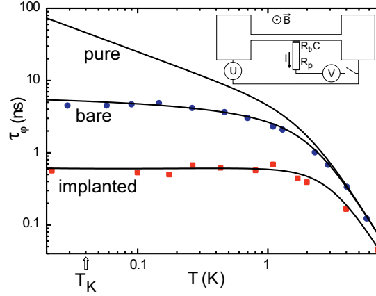
Fig. 3.26. (Color online) Symbols: measured phase coherence time in the two wires. Solid lines: best fits with Eq. (3.96), obtained with c_b = 0.10 \pm 0.01 \text{ ppm} (bare wire) and c_i = 0.95 \pm 0.1 \text{ ppm} (implanted wire). The upper line is the prediction without spin-flip scattering ( c = 0 ). Inset: layout of the circuit. The switch is open for magnetoresistance measurements, closed for energy exchange measurements.
