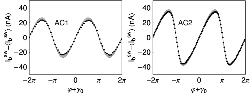
Fig. 1.4. Dots: Measured switching current I_b^{\text{sw}} depending on the reduced flux \varphi = \phi/\phi_0 in the loop for two atomic contacts denoted by AC1 and AC2. Data have been shifted from their average value \langle I_b^{\text{sw}} \rangle which corresponds to the switching current of the Josephson junction alone. Grayed bands: Theoretical prediction for the same current at finite temperature using current-phase relation Eq. (1.4) with the PIN \{\tau_i\} deduced from the I-V characteristics (see Fig. 5.23). The width of the band comes from the uncertainty in the measurement of the PIN. The PIN of AC1 is \{\tau_i\} = \{0.62 \pm 0.01; 0.12 \pm 0.015; 0.115 \pm 0.01; 0.11 \pm 0.01; 0.11 \pm 0.01\} and for AC2, \{\tau_i\} = \{0.957 \pm 0.01; 0.185 \pm 0.05\} .
