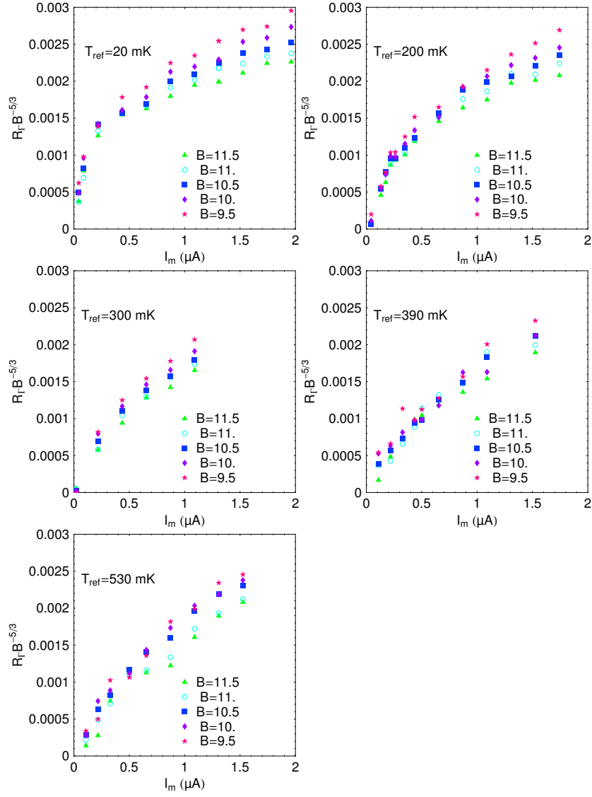
Fig. 7.22. Each panel corresponds to a single temperature of the refrigerator indicated on the top left corner. The dots are the measured offset R_T times B^{-5/3} as a function of the current \langle I_m \rangle obtained for a bias current sI_0 such that B(s) is given by the value indicated by the color of the dot.
