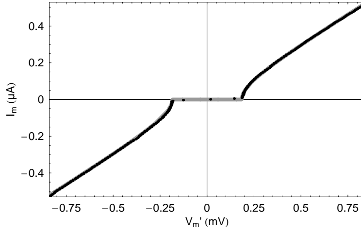
Fig. 7.4. Dots: Measured current-voltage characteristics of the NIS junction at a refrigerator temperature of T_{\text{refrigerator}} = 20 \, \text{mK} . Line: Theoretical curve using Eq. (3.17) at zero temperature with a tunnel resistance of R_t = 1.57 \, \text{k}\Omega and a superconducting gap \Delta = 185.5 \, \mu\text{eV} .
