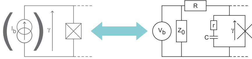
Fig. 5.11. Model of the circuit used to bias the superconducting loop of Fig. 5.7. The characteristic impedance of the transmission lines is Z_0 = 50 \, \Omega . The capacitance C depends on the actual geometry and typically C \approx 30 \, \text{pF} . The resistance r is the sheet resistance of the electrodes that form the external capacitor r \approx 0.1 - 1 \, \Omega .
