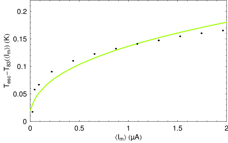
Fig. 7.15. Comparison between the experimental dots of the right panel of Fig. 7.14 and the expression (7.19) using \Sigma = 10^9 \text{ W.m}^{-3}\text{K}^{-5} and \Omega = 5 \times 10^3 \mu\text{m}^3 .
