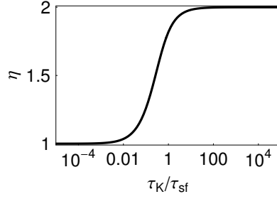
Fig. 2.12. Calculation of the ratio \eta = \tau_{\text{sf}}/\tau_{\varphi}^{(\text{e-}\downarrow, \text{S})} depending on the ratio \tau_{\text{Kor}}/\tau_{\text{sf}} .
