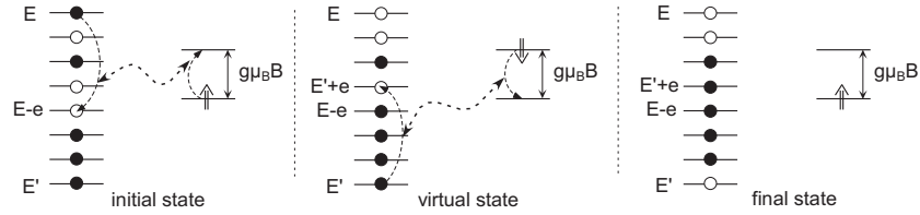
Direct interaction between an electron and a magnetic impurity (first order process)
