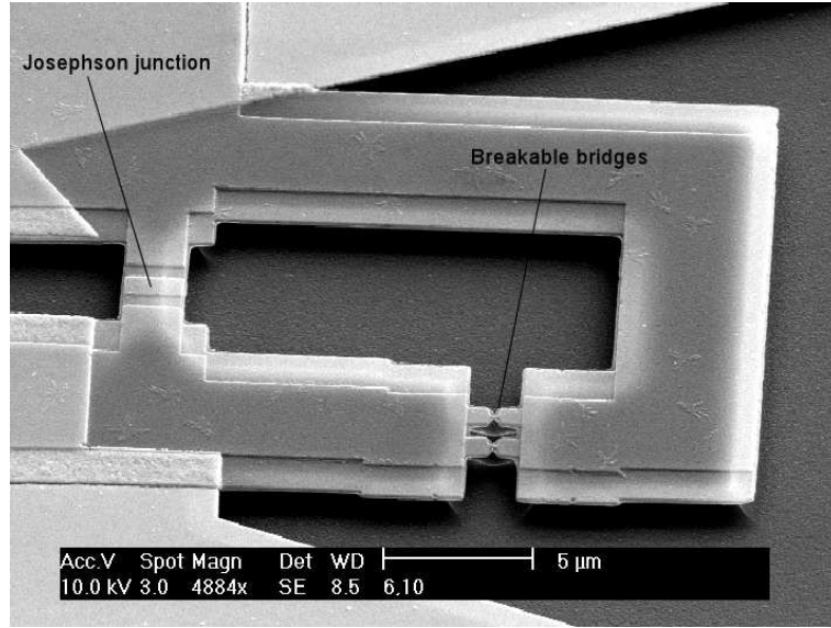
Fig. 5.12. Scanning Electron Microscope picture of the loop schemed on Fig. 5.7. The sample was covered with a thin layer of gold in order to improve the contrast. The picture is taken at an angle of 45^\circ so that it is clear that the polyimide layer has been etched underneath the bridges. The fact that two bridges are present instead of one is a result of the double-angle evaporation technique used for fabricating the Josephson junction, and is of no importance as only one of them forms an atomic contact just before breakage.
