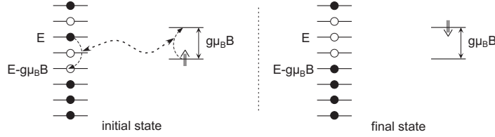
Fig. 3.24. Scheme of the processes involving magnetic impurities and allowing exchange of energy between electrons [37]. On each panel, the left ladder represents the electronic states and the right part schemes the two states of the magnetic impurity lifted by the Zeeman energy. In case the field is zero, both states are degenerate and only the second order process (top) can lead to energy exchange between electrons (figure taken from Ref. [41]).
