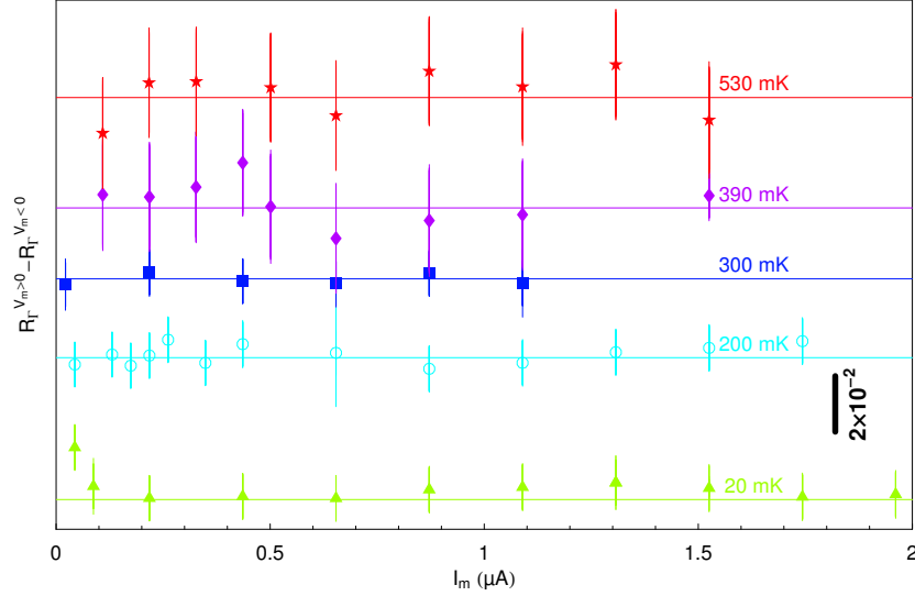
Fig. 7.18. For several refrigerator temperatures, the average difference between the offsets R_L calculated using both methods V_m > 0 and \pm V_b or V_m < 0 and \mp V_b is plotted as a function of the current \langle I_m \rangle . The data were shifted for clarity and the zero corresponding to each temperature is indicated by a line. The error bar is calculated using Eq. (7.27).
