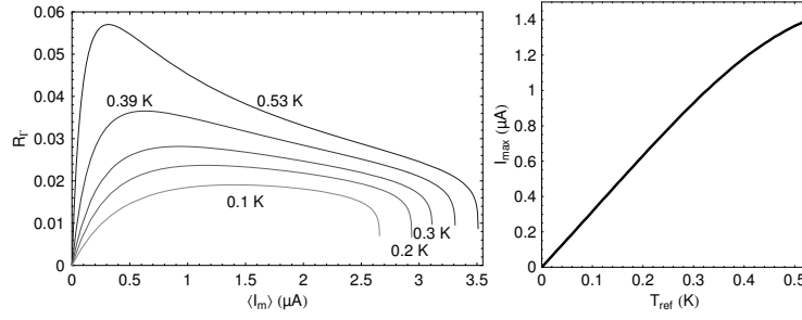
Fig. 7.20. Left panel: theoretical curves for various values of the temperatures of the environment ( T_1 = T_2 ) using Eqs. (7.36,7.17) for a value of s leading to a constant switching rate corresponding to the lowest experimentally accessed rate \Gamma = 5.7 kHz. Right panel: calculated average current \langle I_m \rangle at which the asymmetry R_T is maximal with our experimental parameters as a function of the temperature of the environment.
