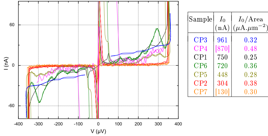
Fig. 5.17. Sub-gap structure of the measured current-voltage characteristics I_{JJ}(V) for the Josephson junction of the seven samples CP1 to CP7. The table recalls some parameters shown in Table. 5.1 (Color online)
