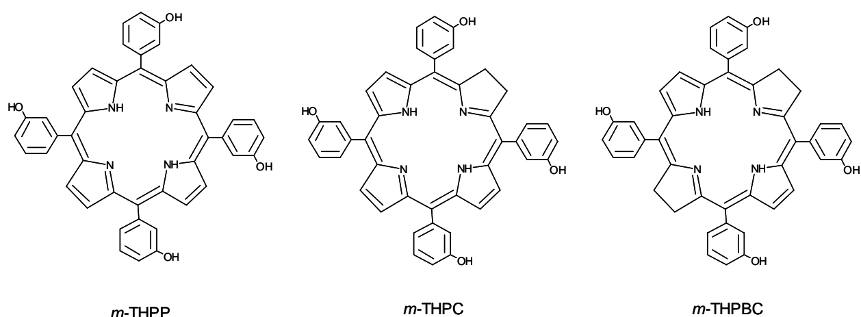
Figure 2.5. : Molecular structures of mTHPP, mTHPC and mTHPBC.
