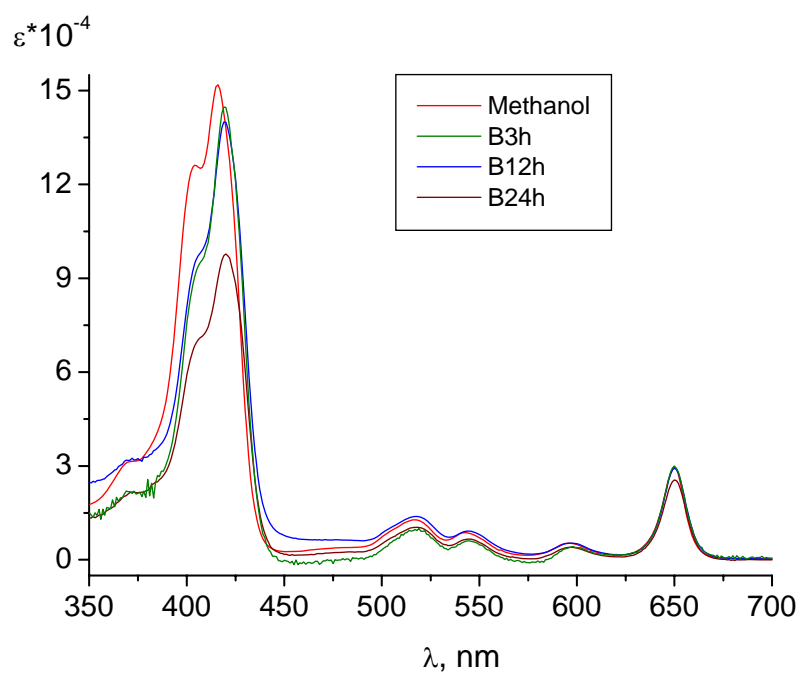
Fig. 2 mTHPC (7.5 \mu\text{M} ) reconstructed absorption spectra in the suspensions of MCF-7 cells at different incubation times and in methanol. Incubation 3 h, 12 h and 24 h at 37 ^{\circ}\text{C} , C_{\text{cells}} = 5.6 \cdot 10^5 cells/mL.
