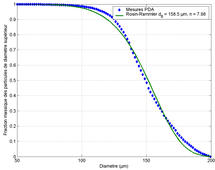
FIG. 4.10 – Particules 100 – 200 \mu\text{m}
