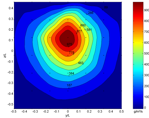
FIG. 5.39 – Particules 50–100 \mu\text{m} , 1000 \text{tr}.\text{min}^{-1}
