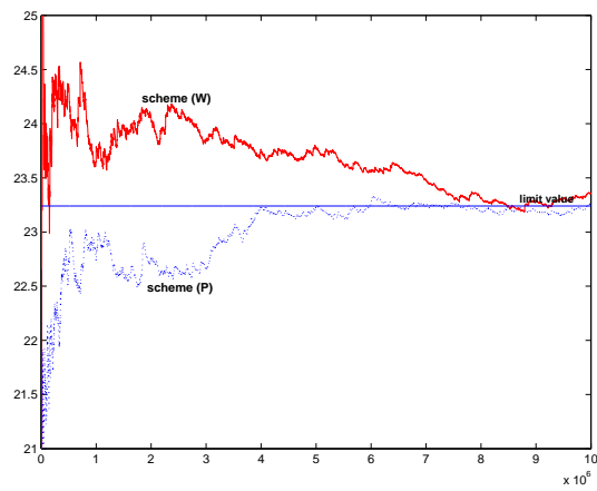
Figure 4.5 : n \mapsto \bar{v}_n(\phi) , \alpha = 1
