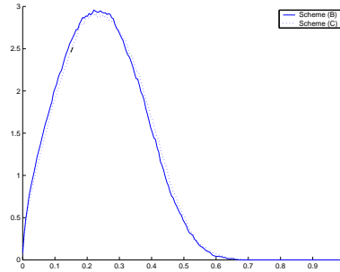
Figure 3.7 : Approximated density, N = 10^6
