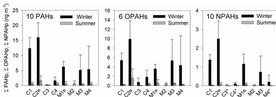
Fig. 2. Average \Sigma PAHp, \Sigma OPAHp and \Sigma NPAHp during winter 2002-2003 and summer 2003 field campaign according to the sampling site (see the Results and discussion section for details). The errors bars show the standard deviation from the weekly average concentration.
