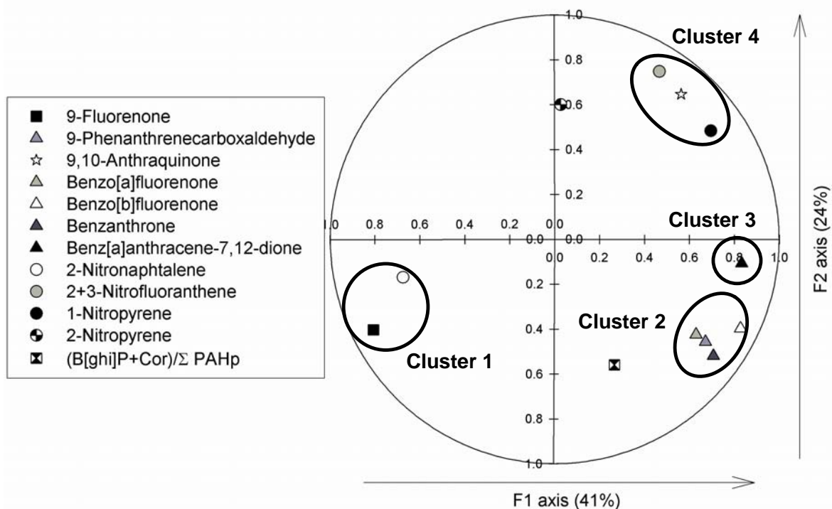
Fig. 4. Correlation circle of normalized single OPAH concentrations (filter + PUF) with normalized 2-NN, 2+3-NF, 1-NP, 2-NP concentrations (filter + PUF) and with (B[ghi]P+Cor)/ \Sigma PAHp ratio (all sampling sites, n=40).
