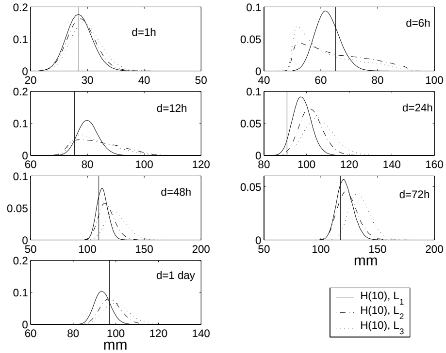
Figure 8: Posterior distributions of the quantiles H_d(10) for d=1 h, 6 h, 12 h, 24 h, 48 h, 72 h and d=1 day (with the last 40 000 simulations of the MCMC algorithm). The vertical lines are
