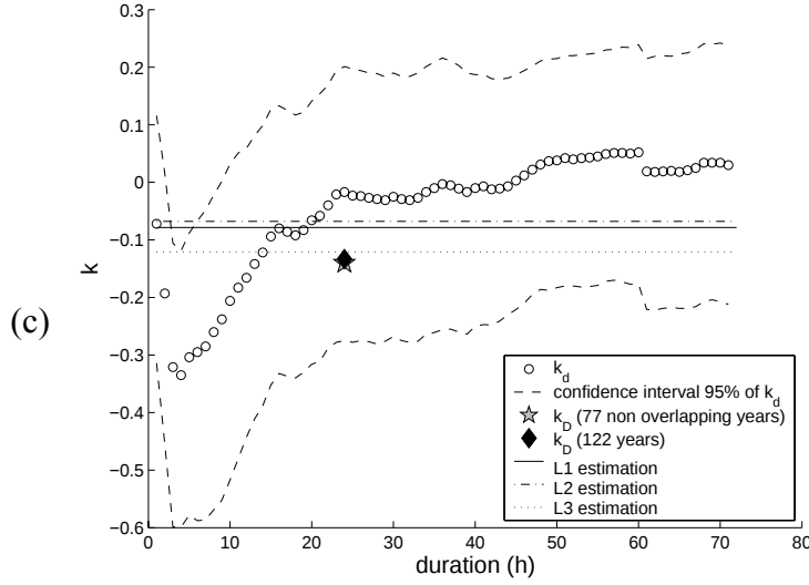
Figure 7: Comparison of \alpha_d , \beta_d , k_d estimates under L_1 , L_2 and L_3 maximizations and constraints
