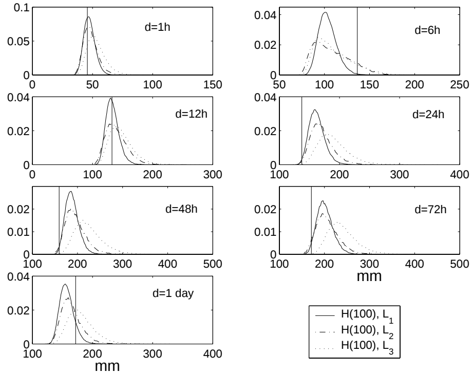
Figure 9: Posterior distributions of the quantiles H_d(100) for d=1 h, 6 h, 12 h, 24 h, 48 h, 72 h and d=1 day (with the last 40 000 simulations of the MCMC algorithm). The vertical lines are
