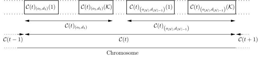
Figure 5.14: Chromosome encoding
