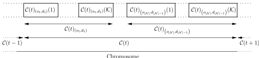
Figure 5.14: Chromosome encoding
