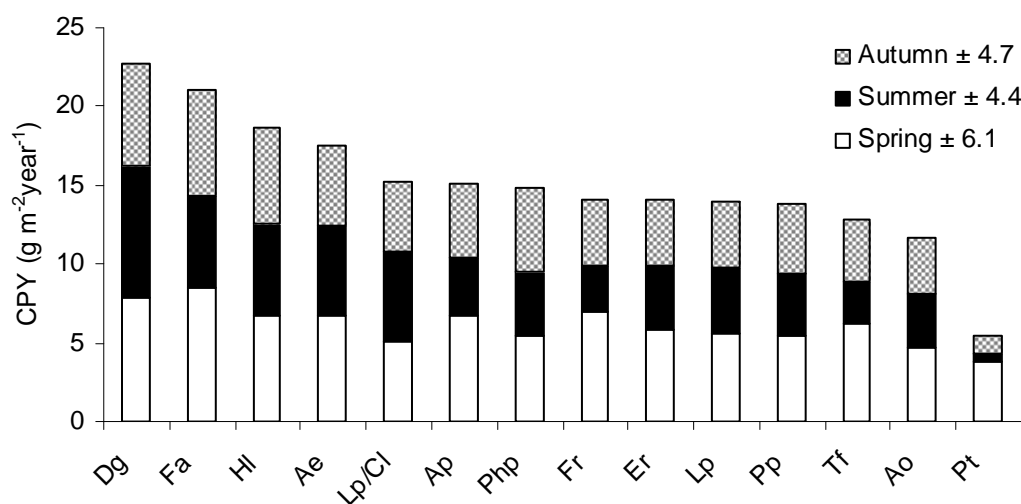
Figure 4-4. Seasonal crude protein yield (CPY, g m -2 year -1 ) for 13 native grasses and for L. perenne cv. Clerpin. Results are means (±SE) of four treatments and two years (n=24). See Figure 4-1 for species code.
