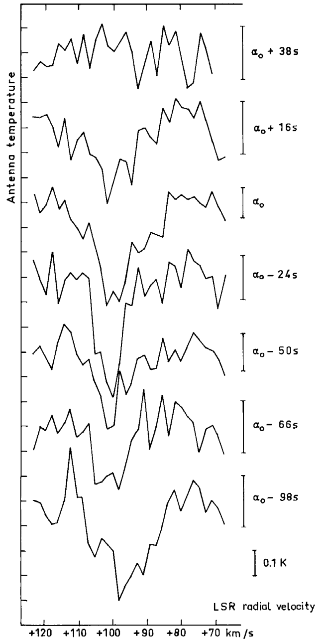
Fig. 5. 1667 MHz profiles taken at the indicated positions, \alpha_0 being the right ascension of G 355.3 + 0.1
