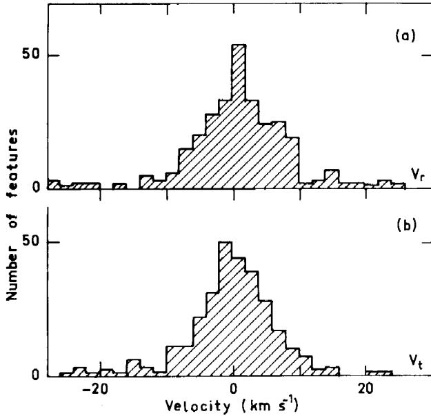
Fig. 1. Velocity histograms. a Observed radial velocities for 296 features at |b| > 10 . b Residual velocities corresponding to the parameters fitted to sample 2 (Table 1)
