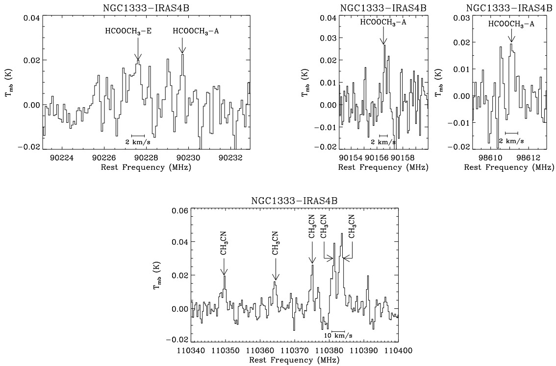
Figure 3.2 Observed spectra towards NGC1333-IRAS4B. The rms are 7, 7 and 5 mK, and the spectral resolutions are 0.2, 0.3, 0.8 \text{km s}^{-1} , at 90, 98 and 110 GHz respectively.
