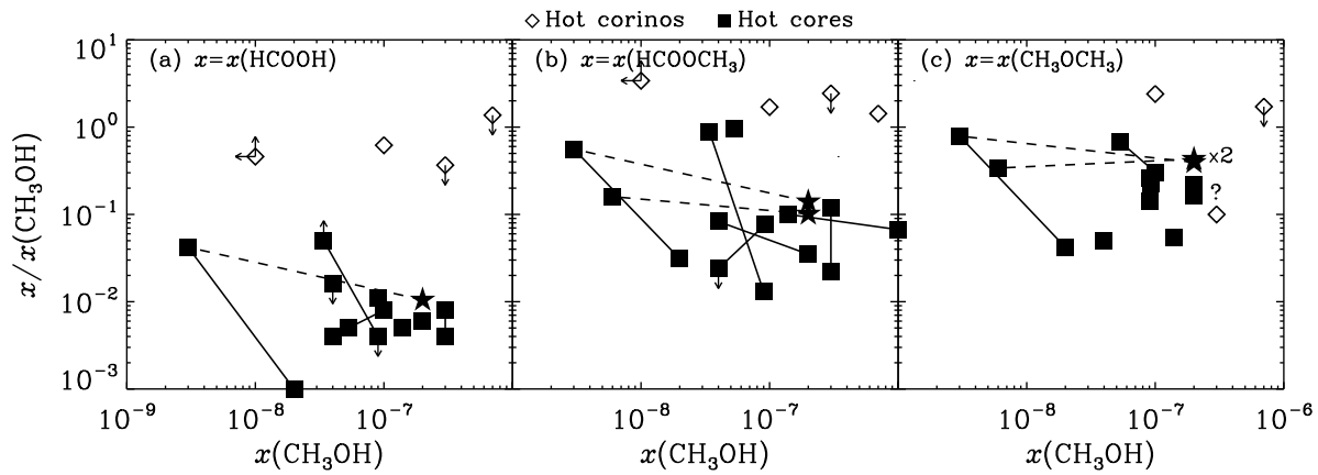
Figure 6.2 Abundance ratios of complex O-bearing molecules to methanol, plotted as a function of the methanol abundance, in hot corinos and in hot cores. Open diamonds represent hot corinos. Filled squares represent abundances ratios of hot cores, derived from beam-averaged column density analysis. See Figure 5.2 for details.
