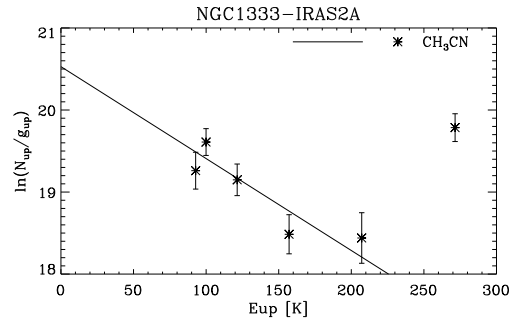
(d) Rotational diagram for \text{CH}_3\text{CN} in IRAS2A. The excess of emission of the transition at 270 K is probably due to contamination from \text{CH}_3\text{OH} 18_{3,16} - 18_{2,17} and this point is not included in the fit.
