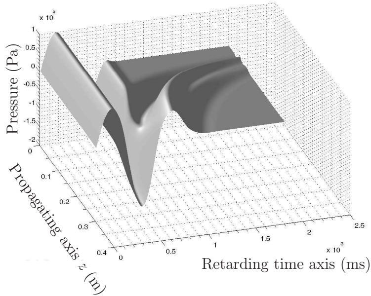
Figure I.1 – The effects of diffraction (I.27) in 3d for the pressure with a square source 3\text{ cm} \times 3\text{ cm} . The parameters of simulation for propagation in water: \Delta y_1 = \Delta y_2 = 3.75 \times 10^{-4}\text{ m} , \Delta z = 6 \times 10^{-4}\text{ m} , \Delta \tau = 6.6667 \times 10^{-9}\text{ s} , \rho_0 = 1000\text{ kg/m}^3 , c = 1500\text{ m/s} .
