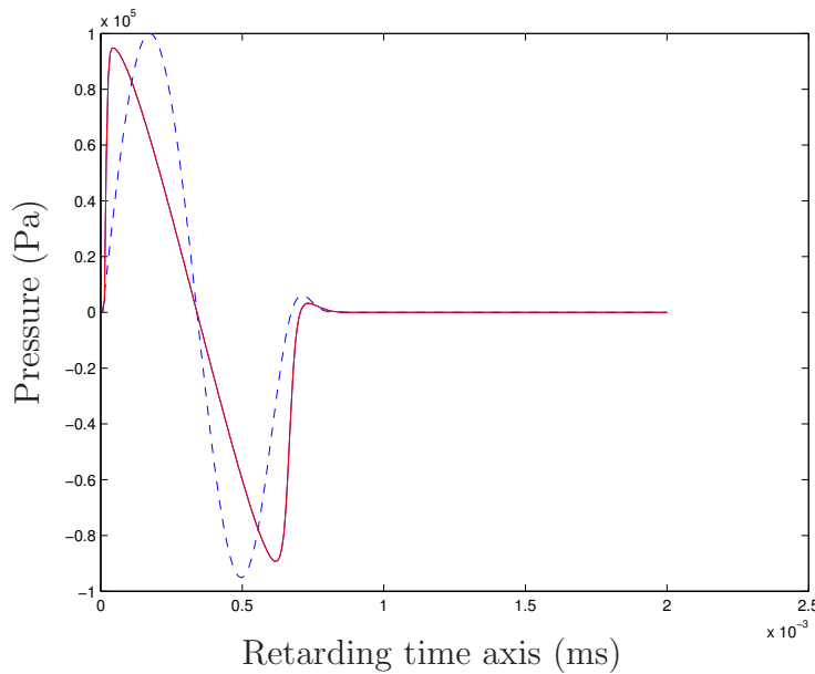
Figure I.4 – The effects of absorption and nonlinear effects (I.30) along the retarded axis \tau in the two different places of the propagation axis z with a square source 3 \text{ cm} \times 3 \text{ cm} . The dotted line corresponds to the signal source z = 0 and the solid line to the pressure at the distance z = 1 \text{ m} . The parameters of simulation are the same as in figure I.3.
