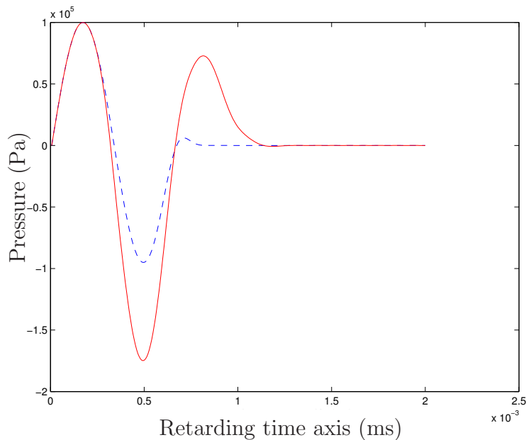
Figure I.2 – The effects of diffraction (I.27) along the retarded axis \tau in the two different places of the propagation axis z with a square source 3\text{ cm} \times 3\text{ cm} . The dotted line corresponds to the signal source z = 0 and the solid line to the pressure at the distance z = 30\text{ cm} . The parameters of simulation are the same as in figure I.1.
