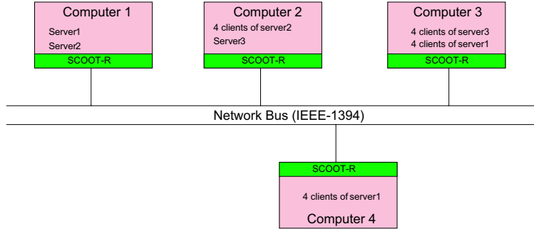
Figure 4.16: Application configuration
