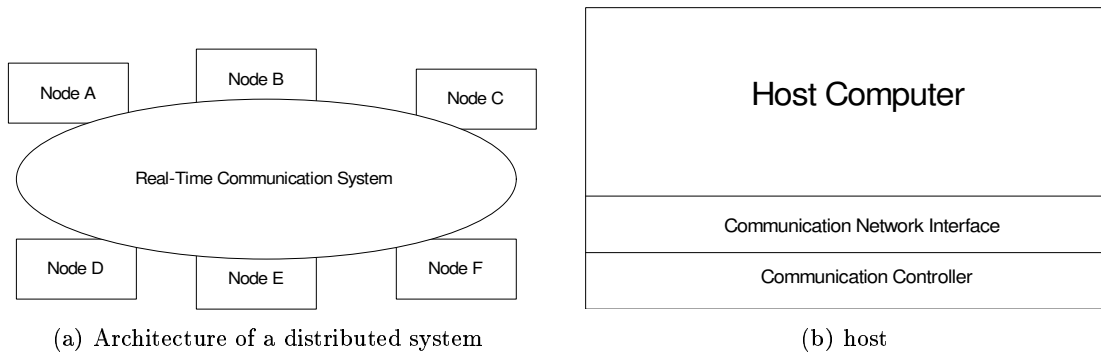
Figure 1.2: Architecture of a distributed system
