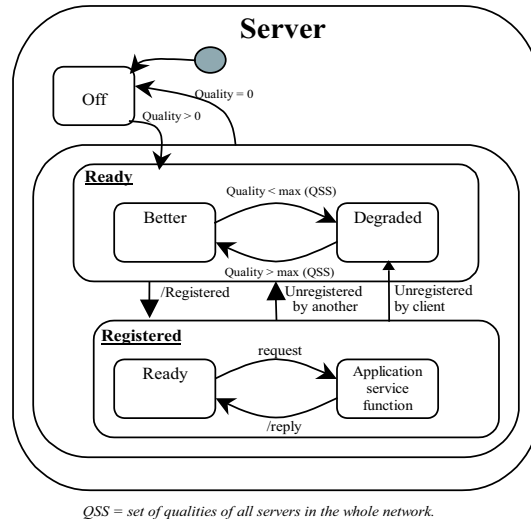
Figure 3.13: Simplified statechart of a server operation
