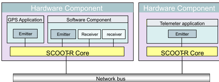
Figure 3.9: Component-oriented architecture – emitter/receiver Model
