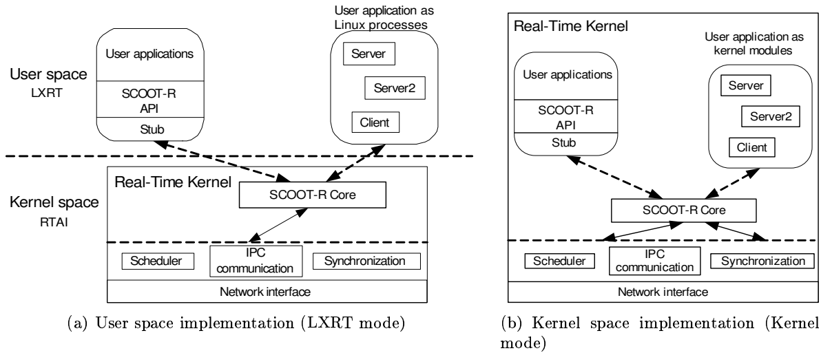
Figure 3.7: Service implementation
