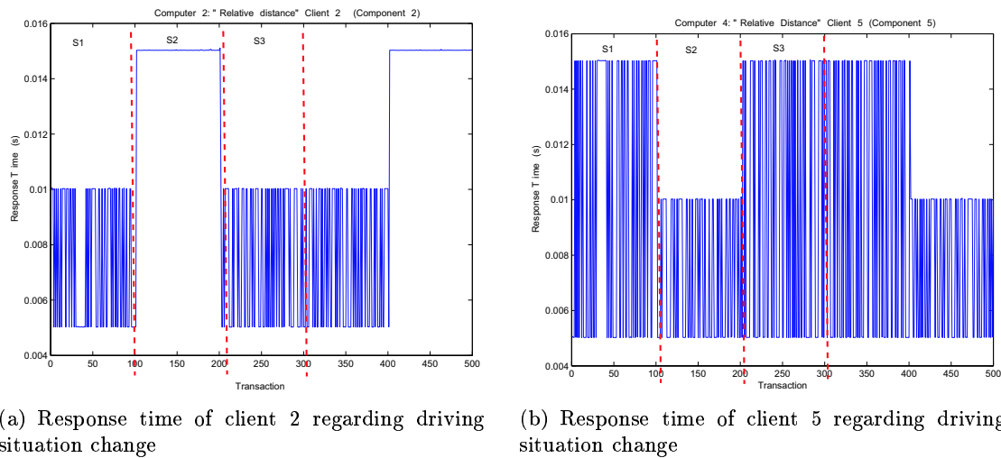
Figure 5.15: Transactions response time
