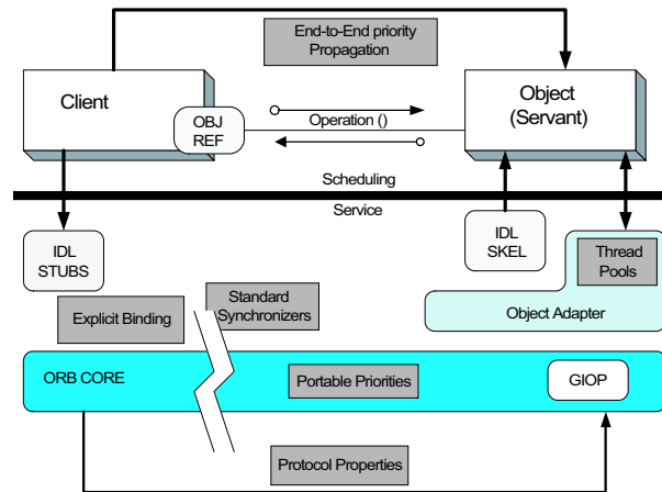
Figure 2.5: Real-Time CORBA
