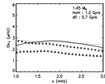
Fig. 5. Small separations for models M 1.45 at 1.2 Gyr (with diffusion) and 1.6 Gyr (without diffusion) on the left, and at 0.7 Gyr (with diffusion) and 1.2 Gyr (without diffusion) on the right. The lines are for models with diffusion (solid lines: D\nu_{0,2} , dotted lines: D\nu_{1,3} ) and the symbols are for models without diffusion (triangles: D\nu_{0,2} , diamonds: D\nu_{1,3} ).
