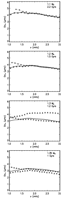
Fig. 4. Small separations for models M 1.1 to M 1.35 at different ages. The lines are for models with diffusion (solid lines: D\nu_{0,2} , dotted lines: D\nu_{1,3} ) and the symbols are for models without diffusion (triangles: D\nu_{0,2} , diamonds: D\nu_{1,3} ).
